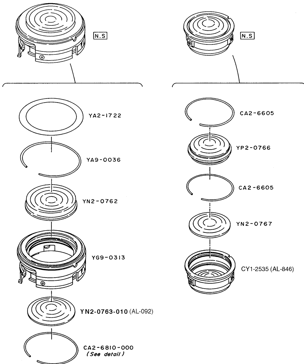
CA2-6810-000 detail
