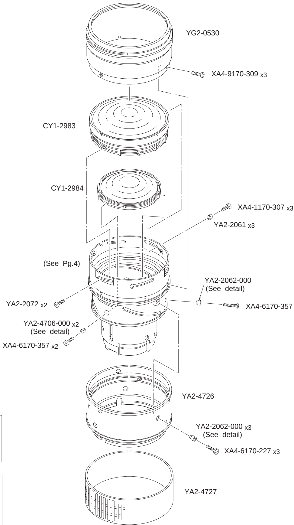
YA2-2062-000 detail
