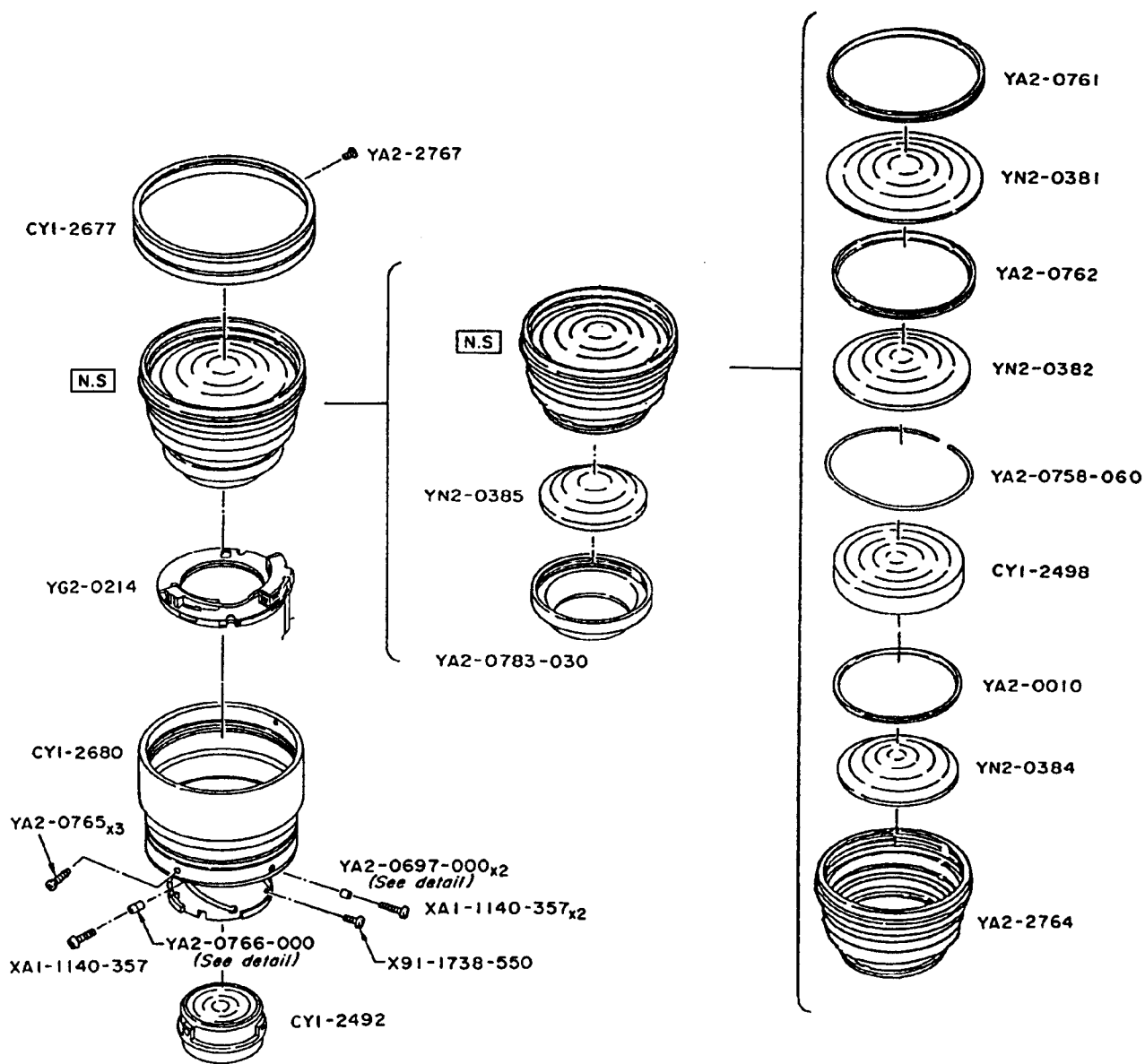
YA2-0697-000 detail
