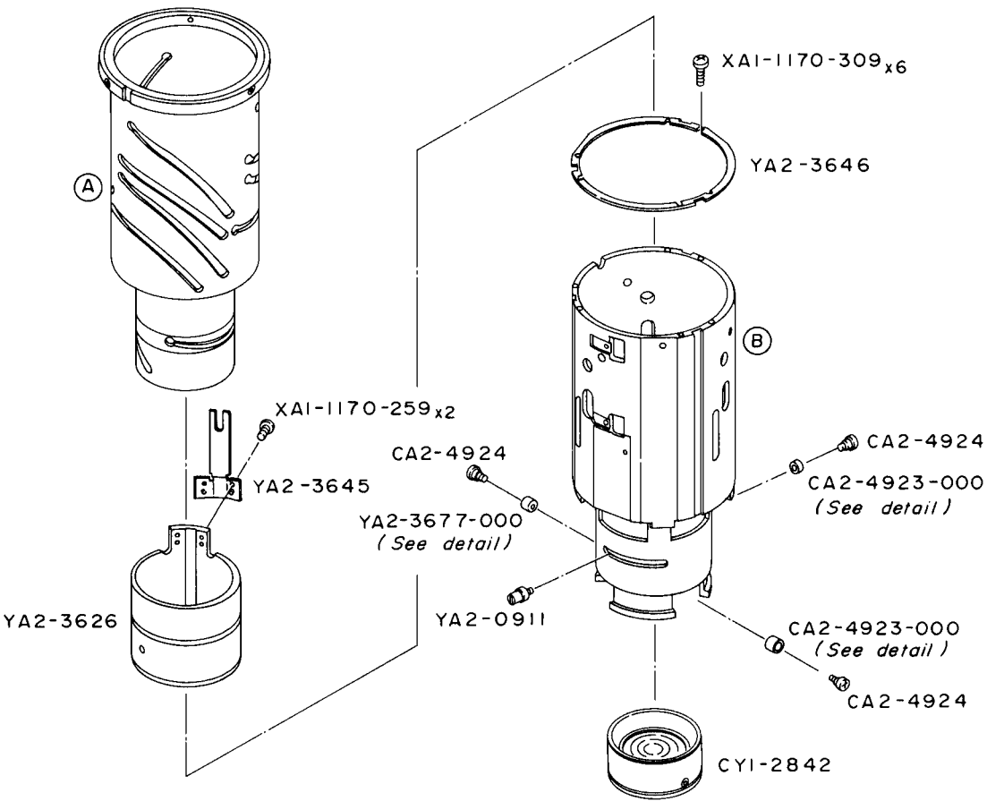
CA2-4923-000 detail
