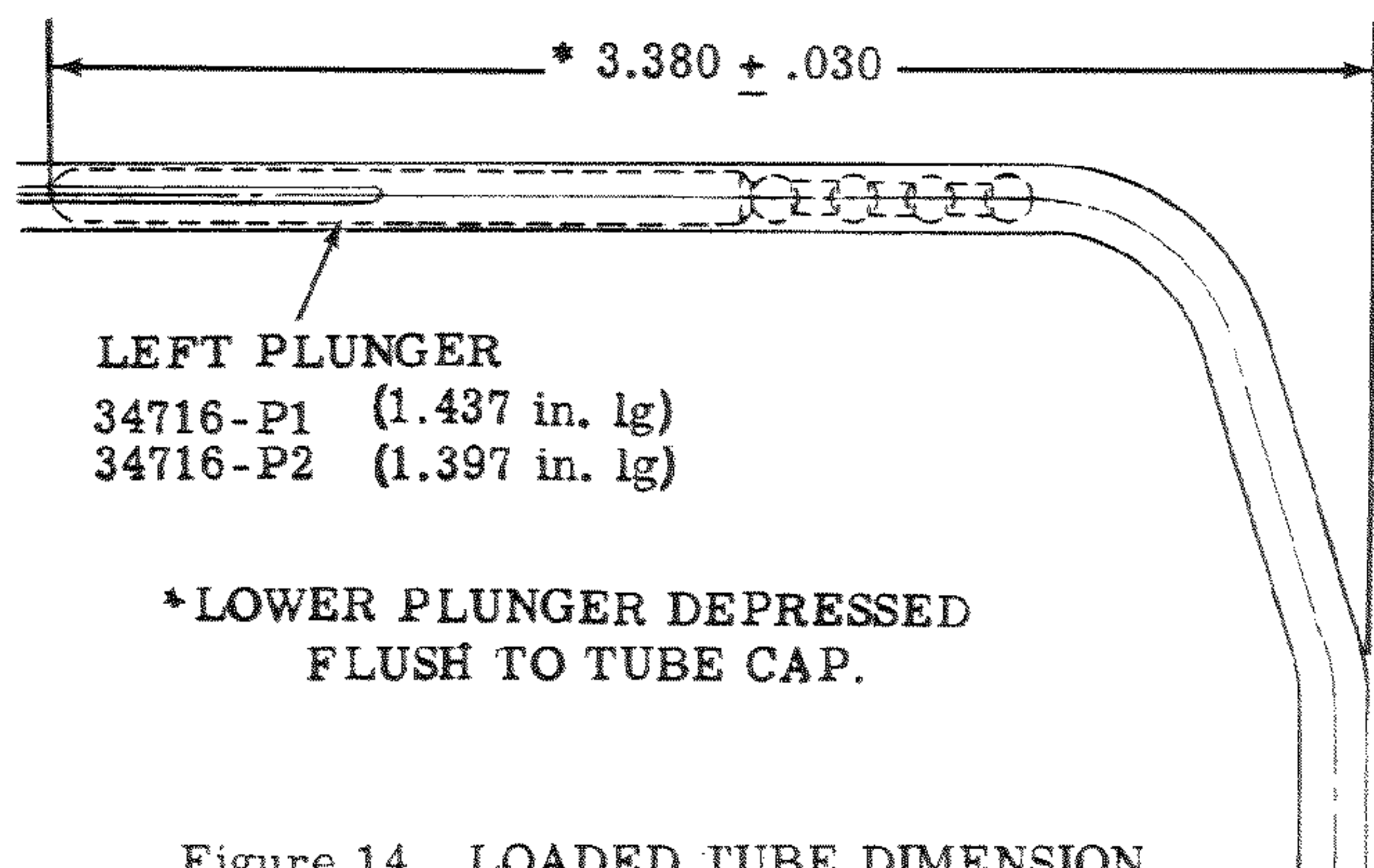
Figure 14. LOADED TUBE DIMENSION.
