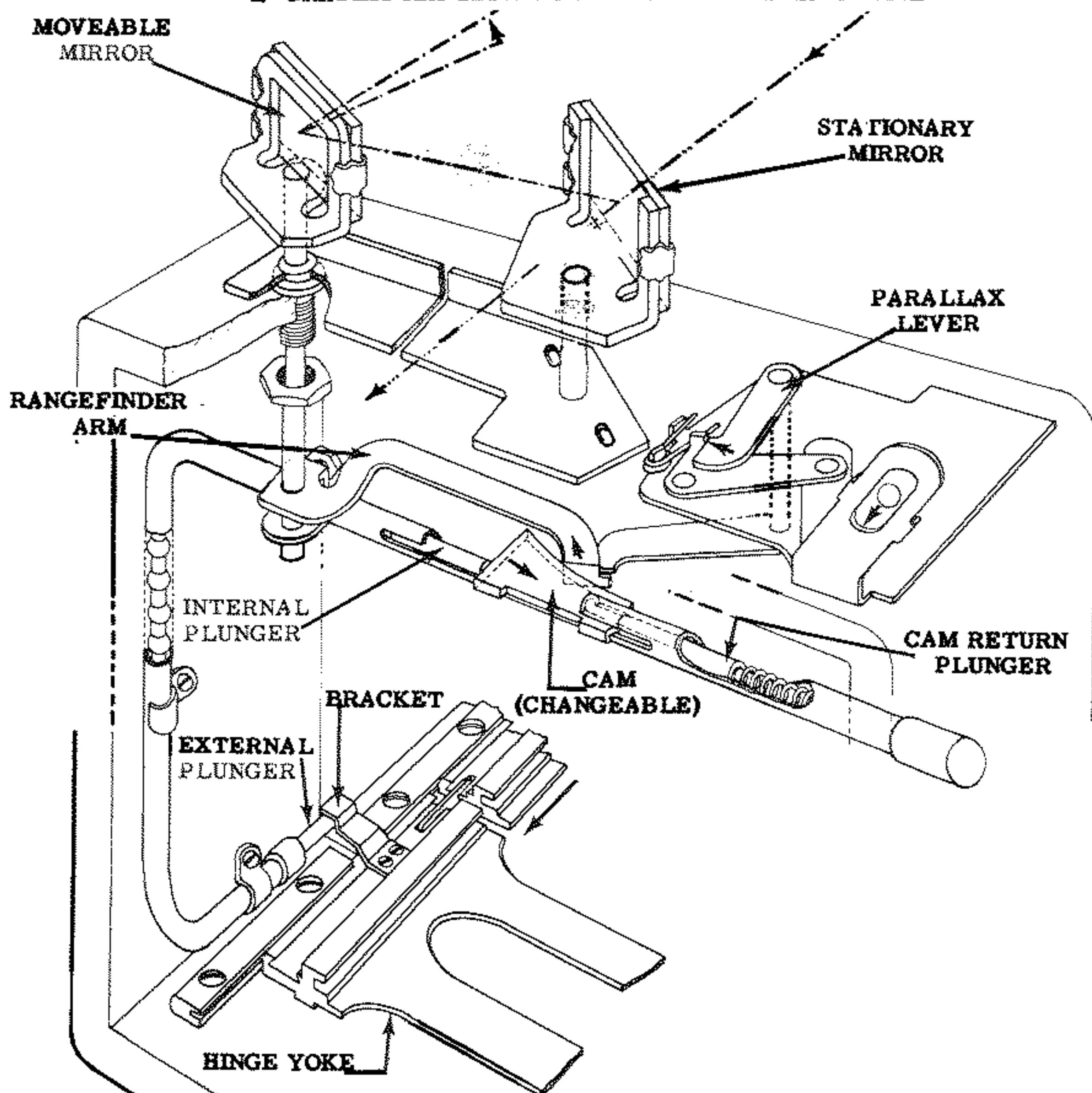
Figure 4. RANGEFINDER OPERATION
