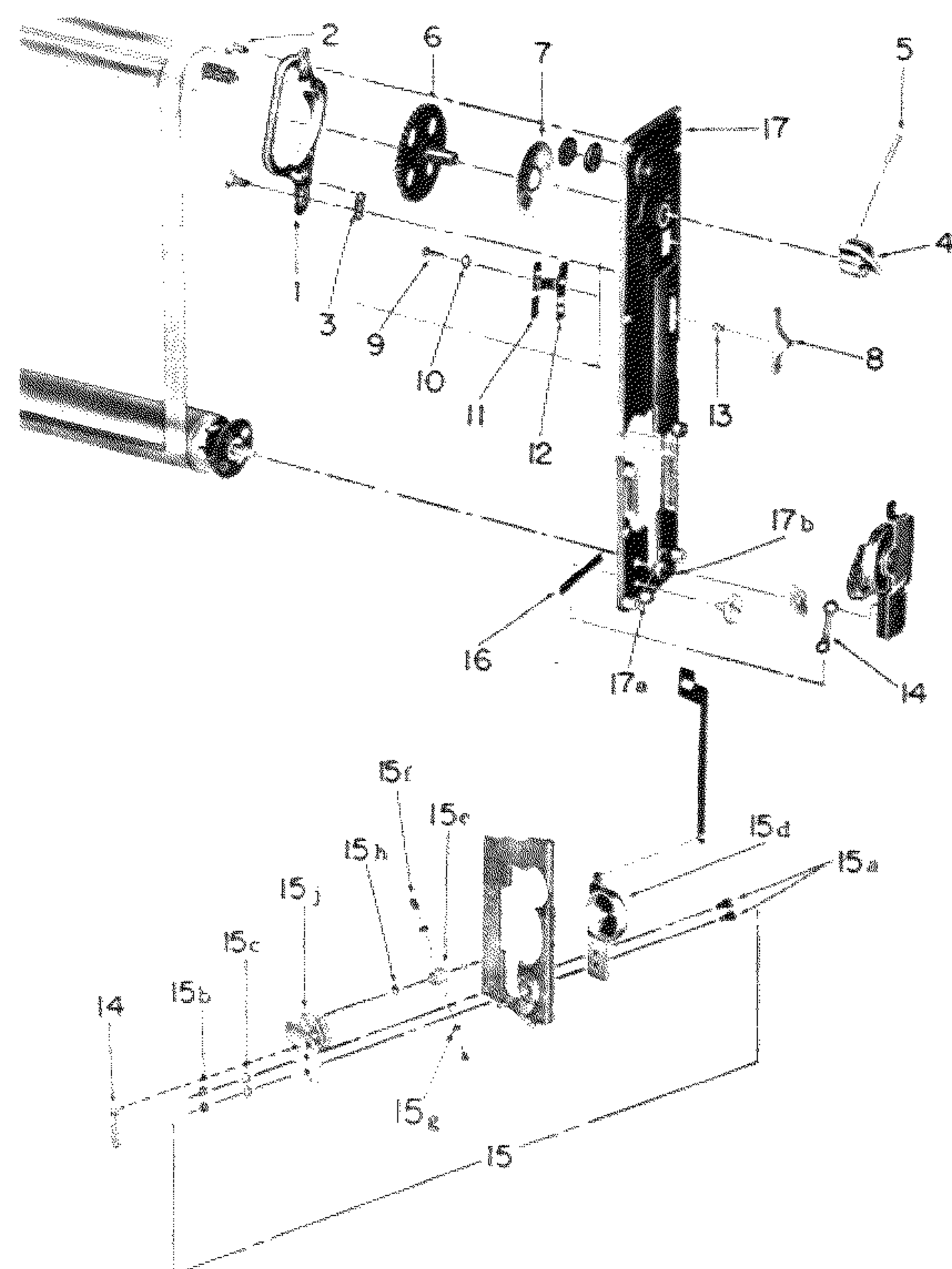
Figure 5. SHUTTER PLATE
