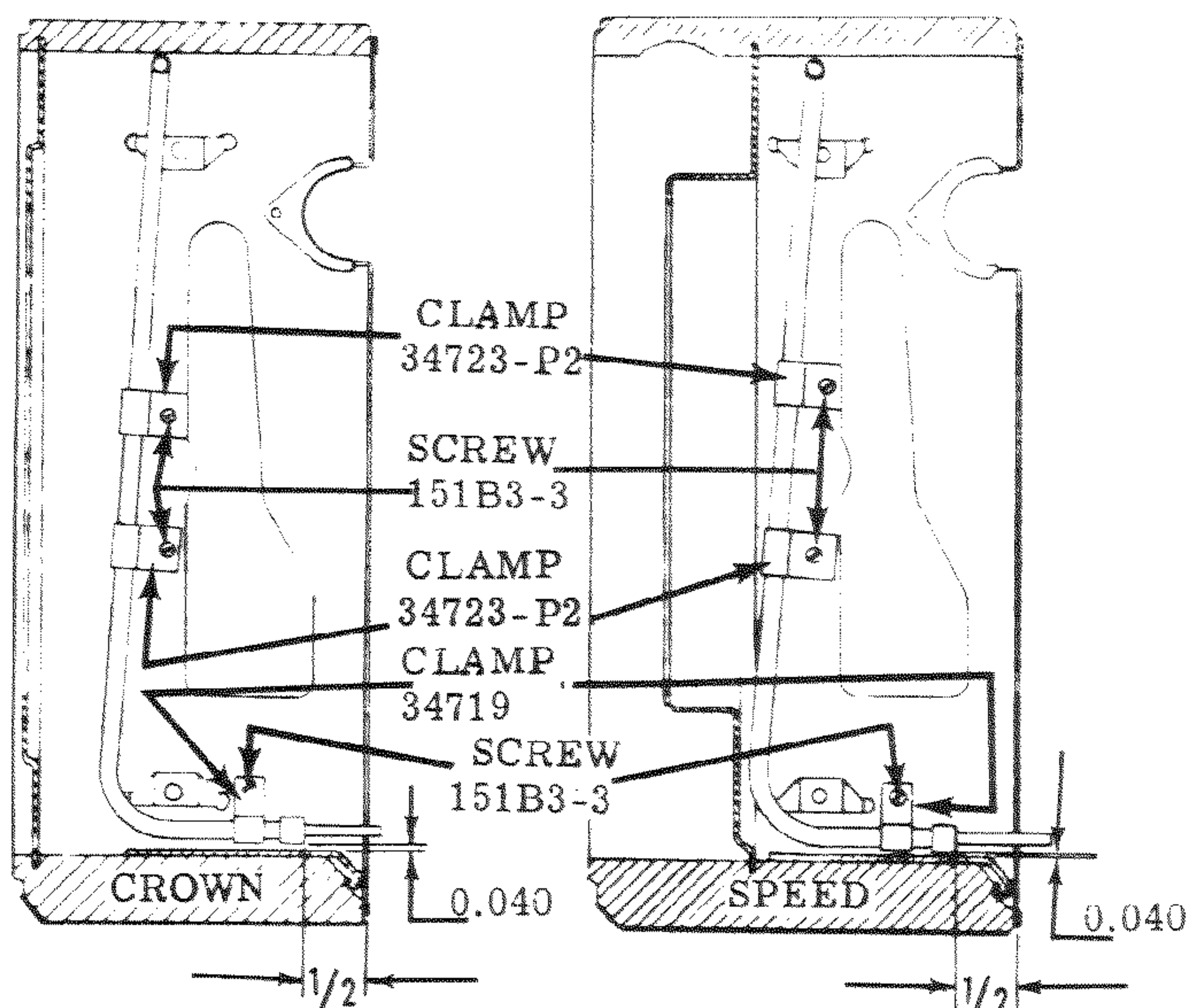
Figure 15. TUBE CLAMPS
