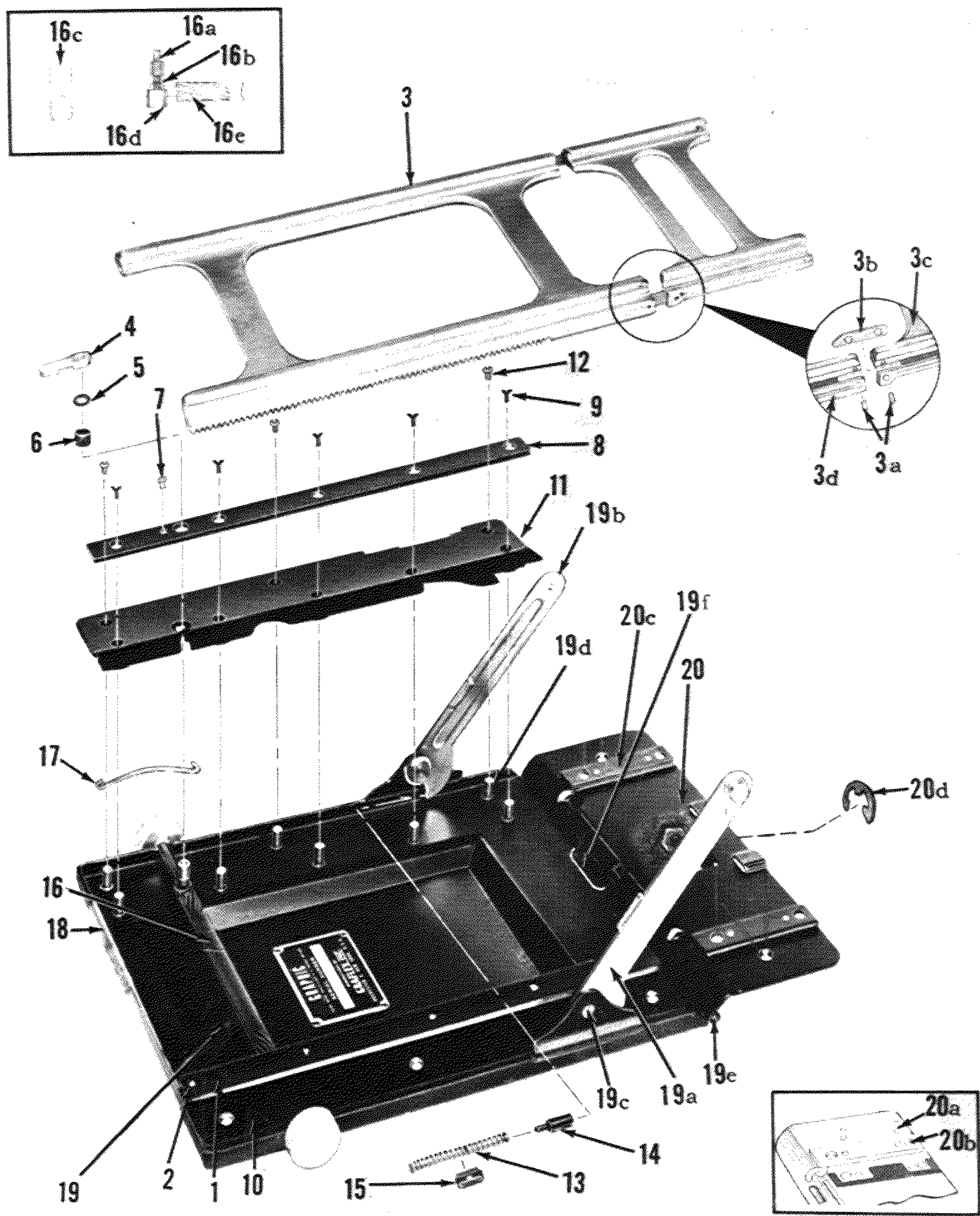
Figure 7. BED COMPLETE
