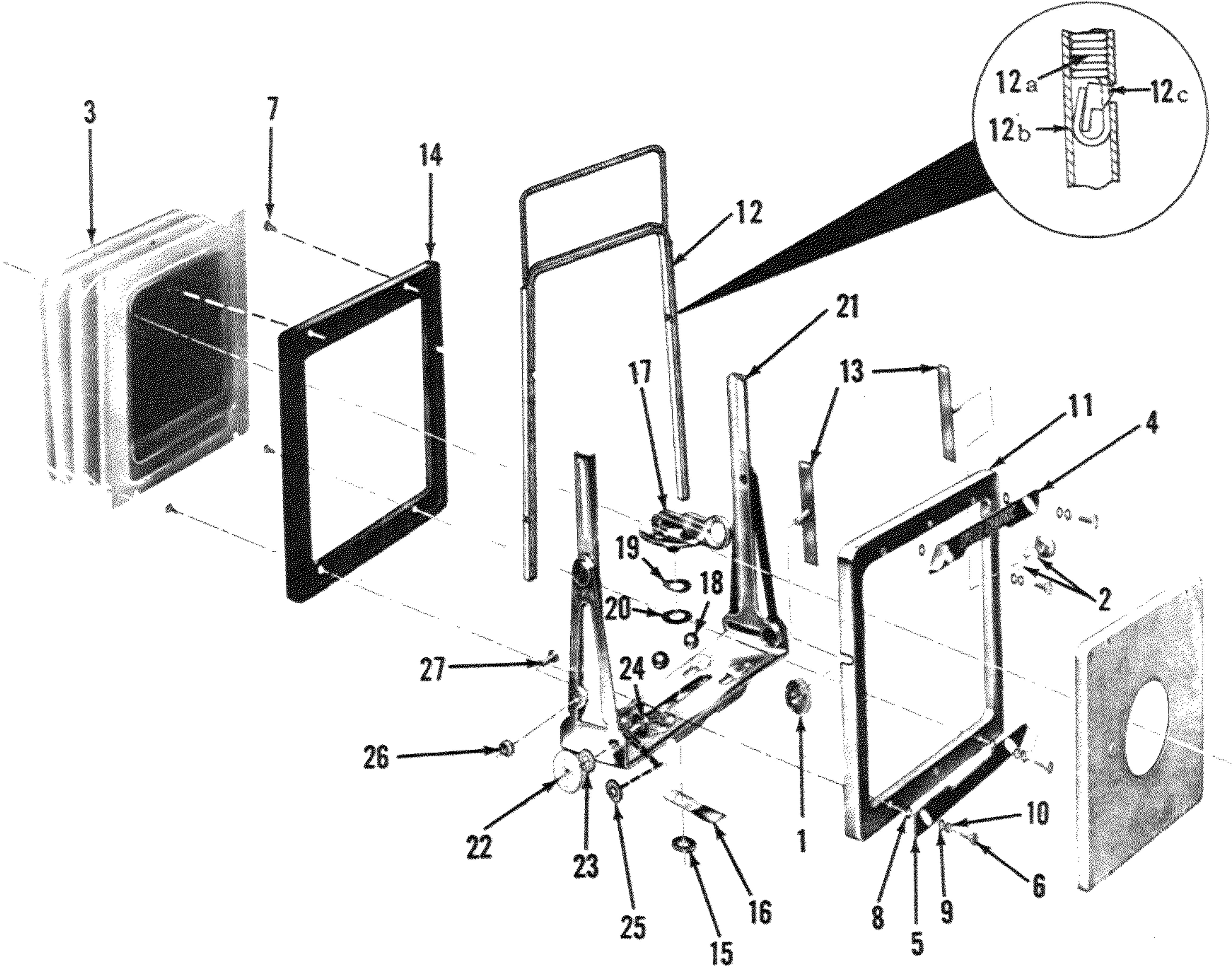
Figure 6. FRONT STANDARD
