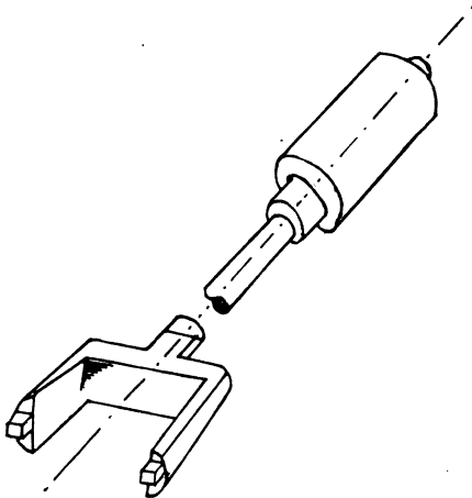
Jam nut(122)driver
