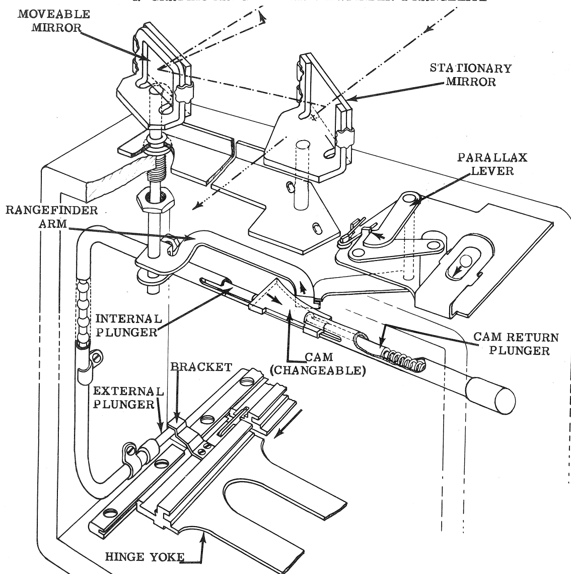
Figure 4. RANGEFINDER OPERATION
