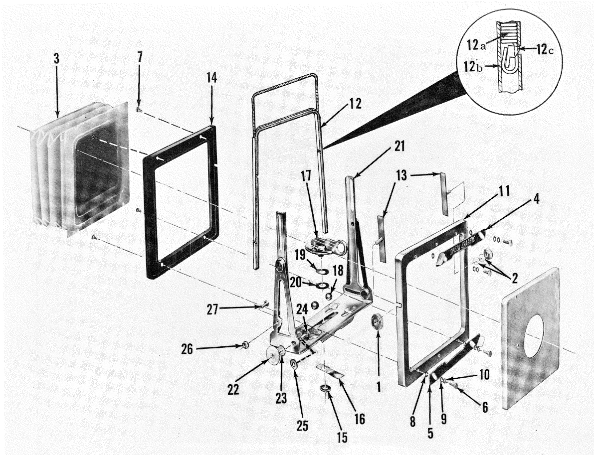
Figure 6. FRONT STANDARD
