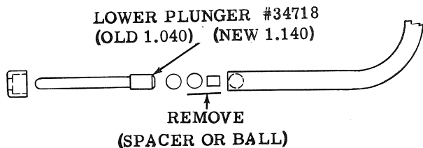
Figure 13. PLUNGER REPLACEMENT
