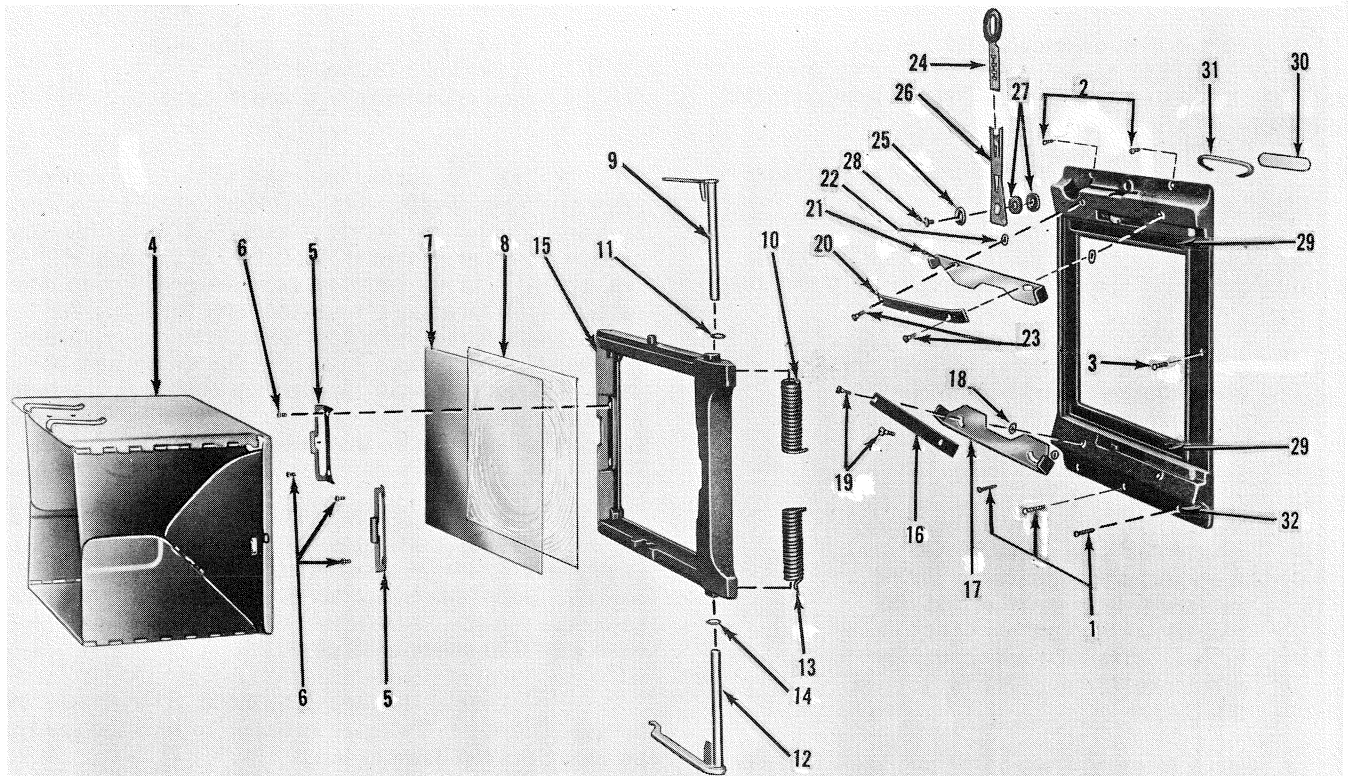
Figure 16. Graflok Back and Hood Assembly
