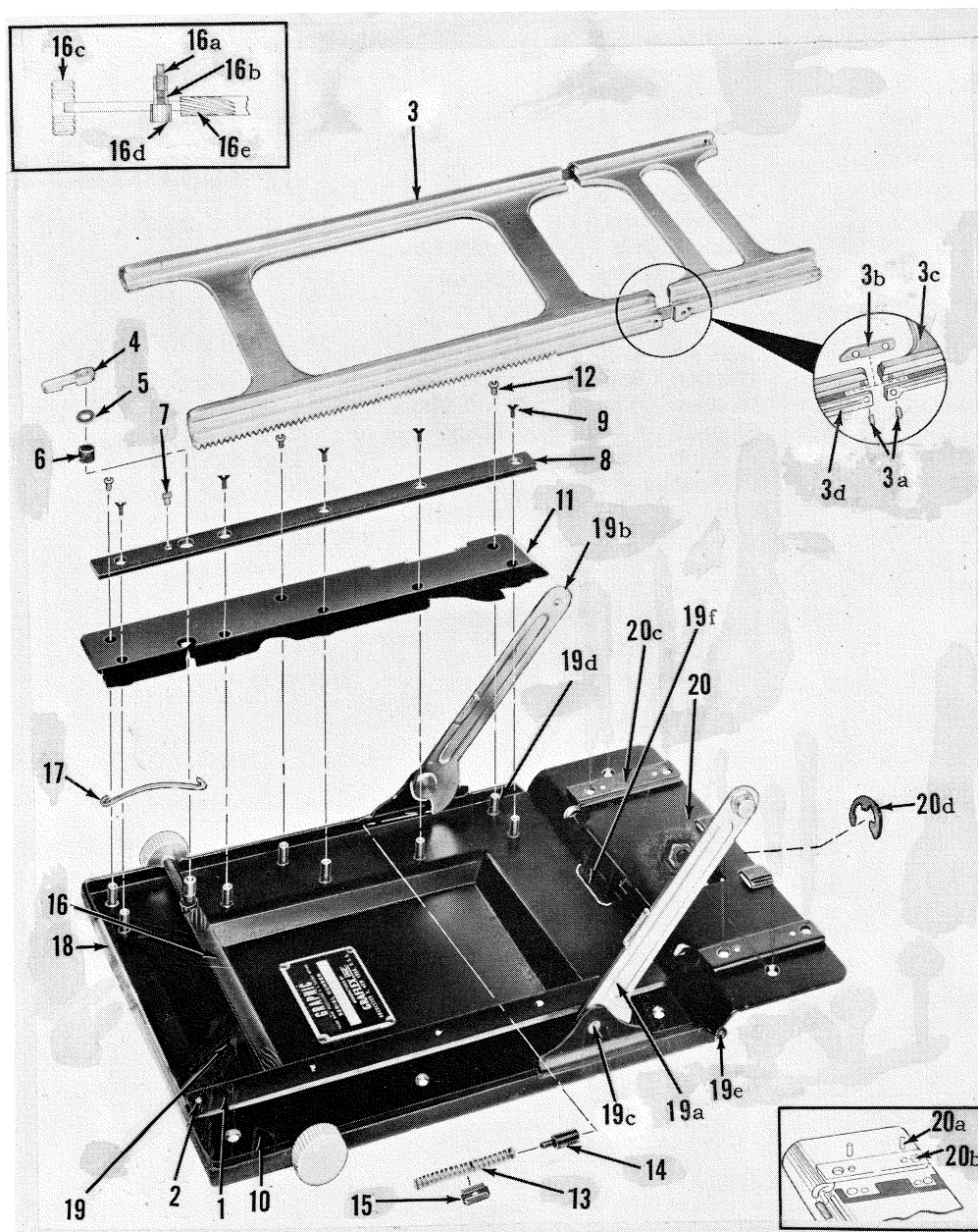
Figure 7. BED COMPLETE
