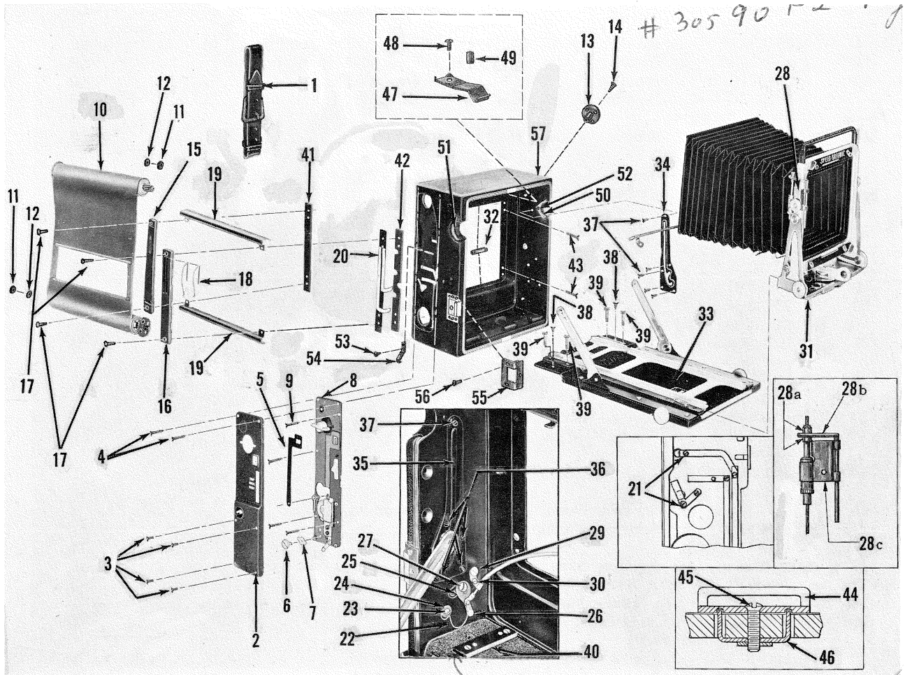
Figure 3. CAMERA BASIC
