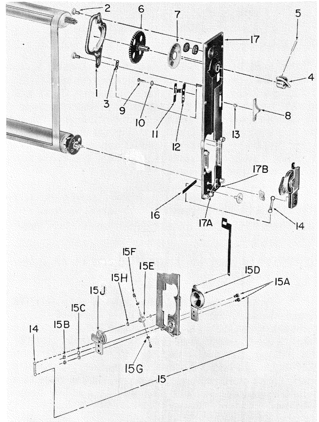
Figure 18. Shutter Plate
