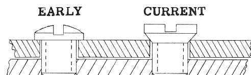
Figure 12. BRACKET SCREWS
