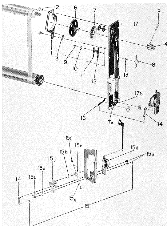
Figure 5. SHUTTER PLATE
