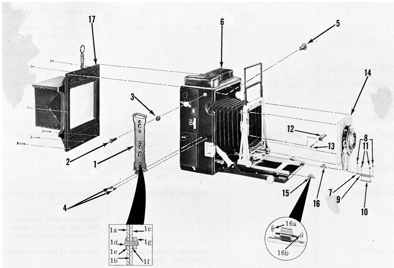
Figure 1. CAMERA COMPLETE
