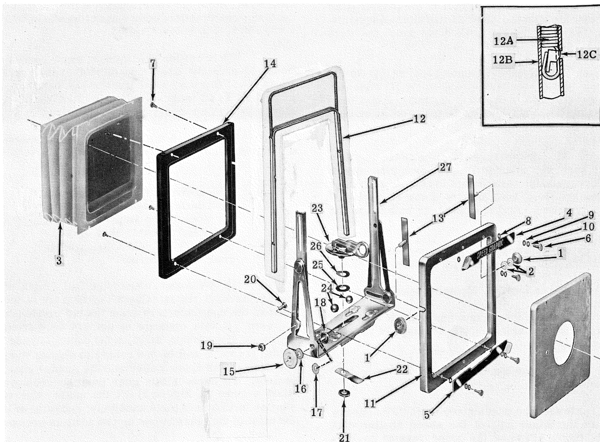
Figure 19. Front Standard Complete
