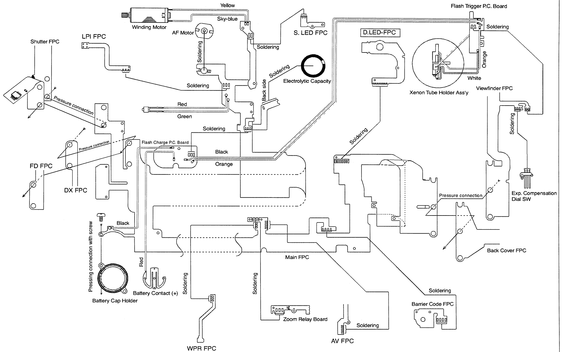
WIRING DIAGRAM
