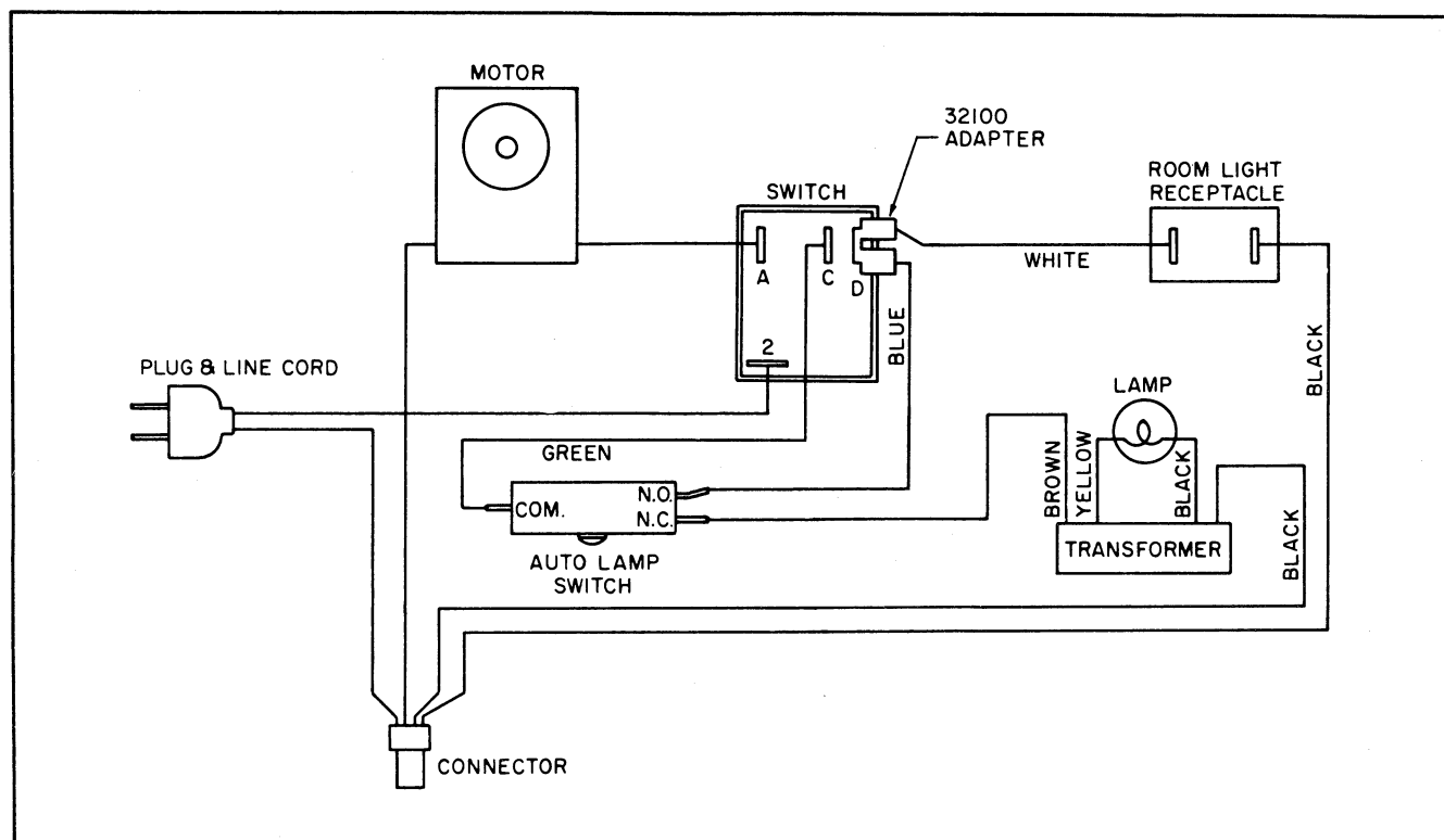
Figure C. Wiring Diagram
