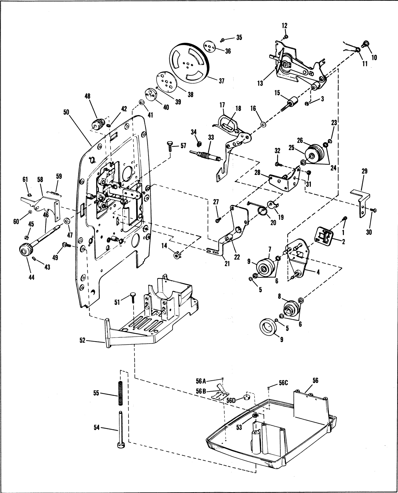
Figure 5. Shutter and Shuttle Mechanism
