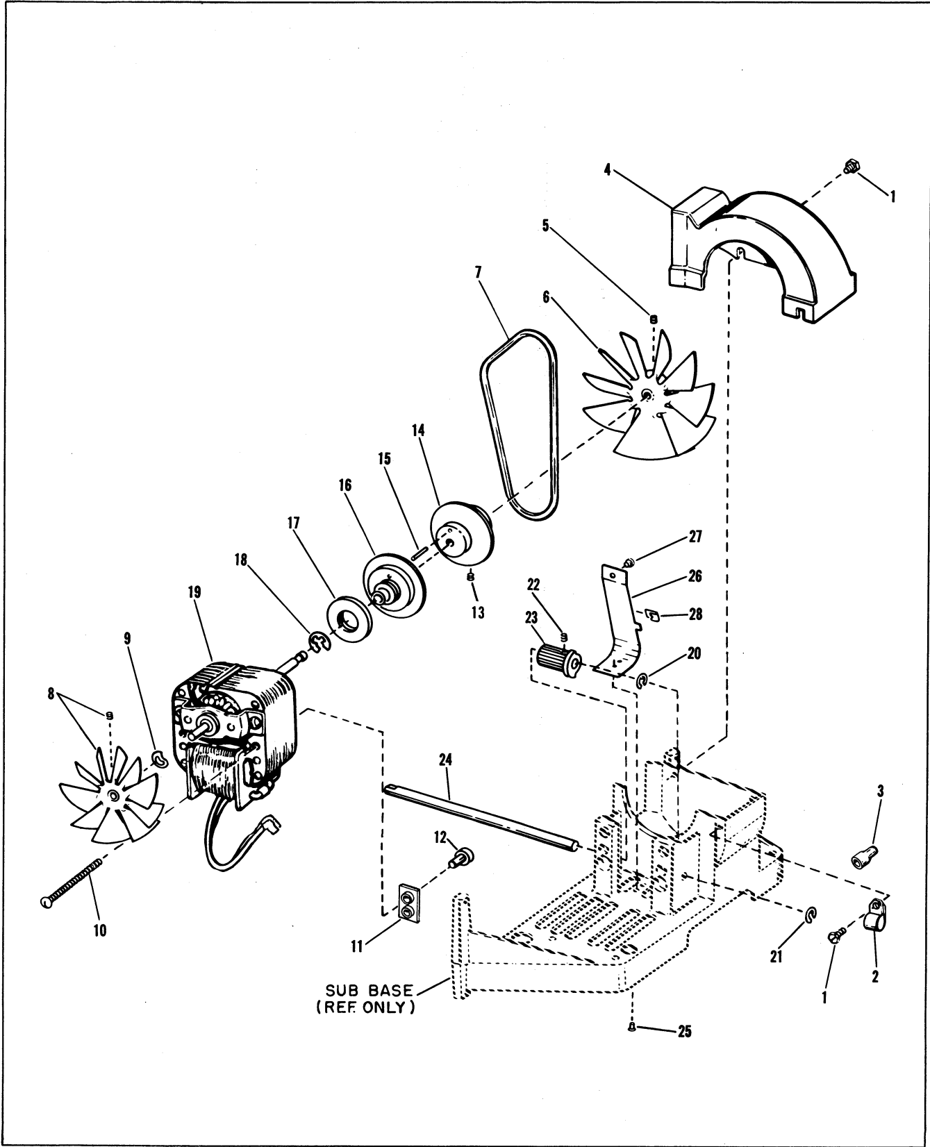
Figure 3. Motor, Fan, and Speed Control
