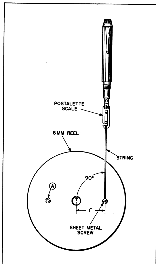
Figure D. Checking Reel Arm Torque
