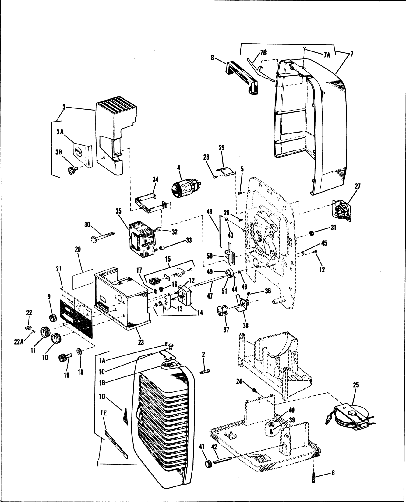
Figure 1. Covers and Lamp
