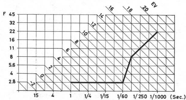
Fig. 61 Programmed shutter diagram (ISO 100, 2.8/75mm)
