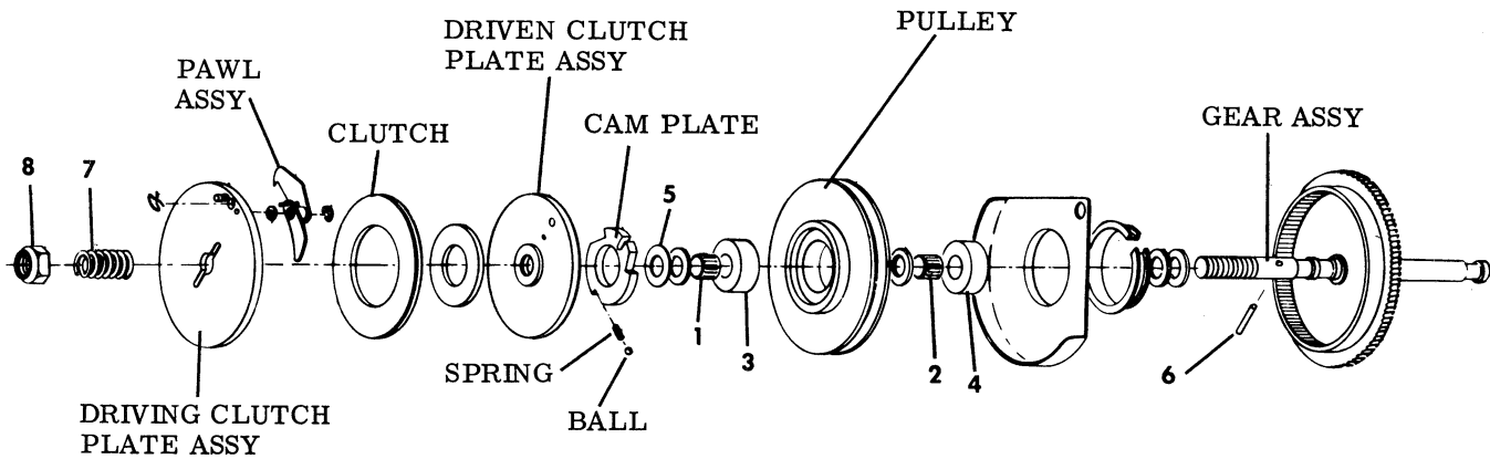
(Figure 1-3). FILM FEED CLUTCH ASSEMBLY
