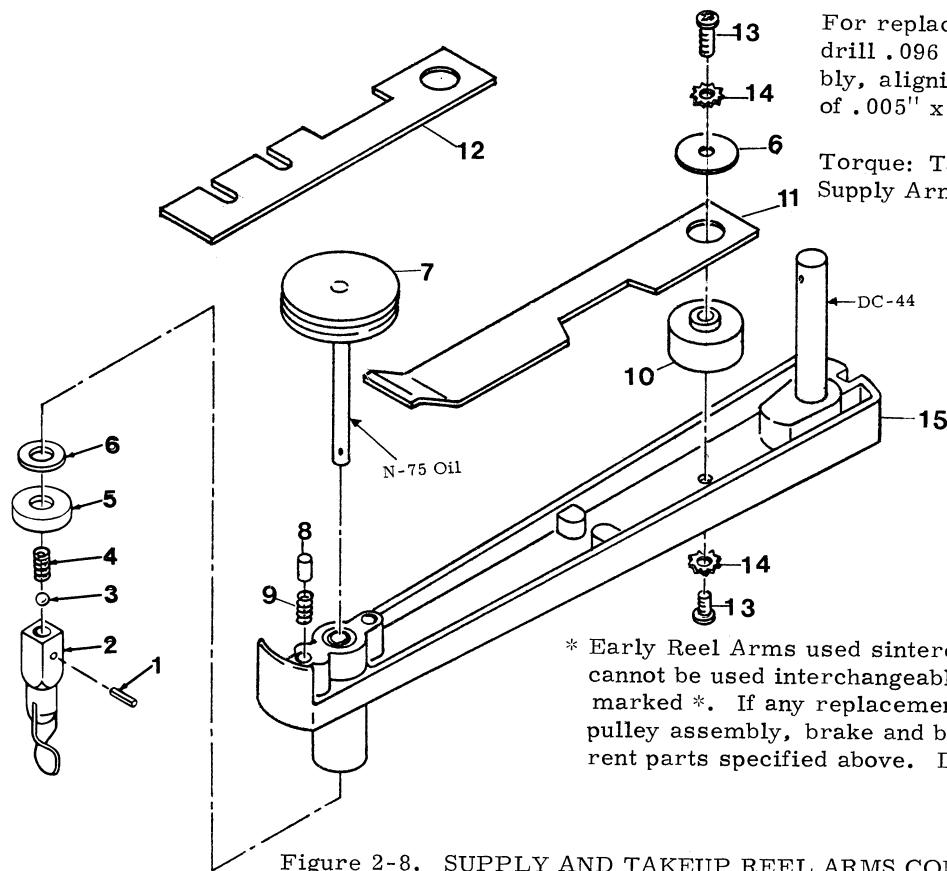
Figure 2-8. SUPPLY AND TAKEUP REEL ARMS COMPLETE
