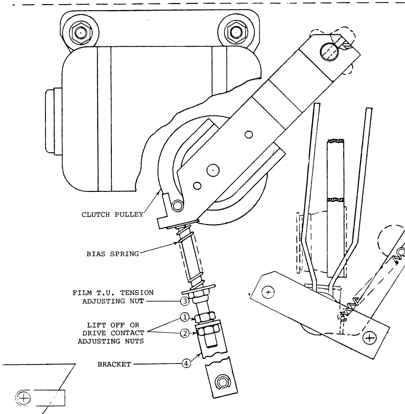
Figure 4-16. TAKE-UP CLUTCH ADJUSTMENTS
