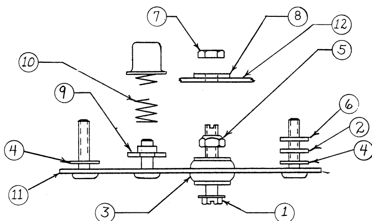
Figure 4-3. 1030N MOTOR MOUNT ADJUSTMENTS
