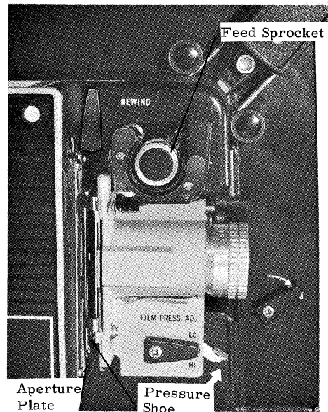
Figure 1-5. GATE AND LENS MOUNT
