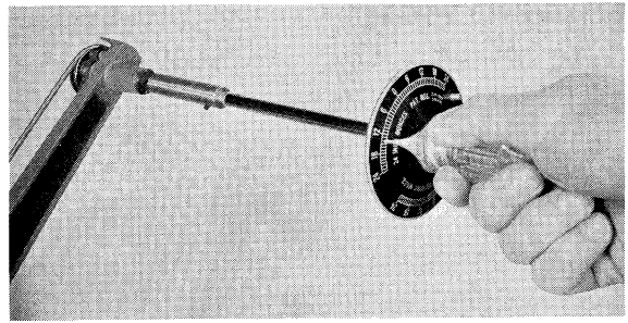
Figure 4-28. REVERSE DRIVE TORQUE MEASUREMENT.
