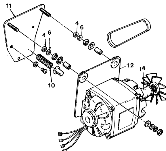
Figure 4-4. 1030N MOTOR MOUNT ADJUSTMENTS
