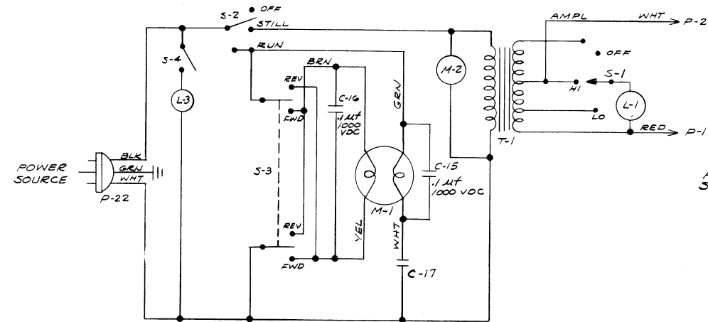
SCHEMATIC DIAGRAM H43947-1, PROJECTOR PORTION. APPLICABLE TO MODELS 1020, 1021 AND 1022.
