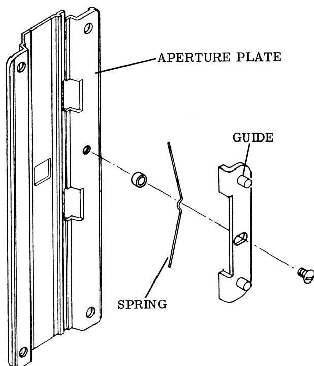
Figure 3-12. APERTURE PLATE ASSEMBLY
