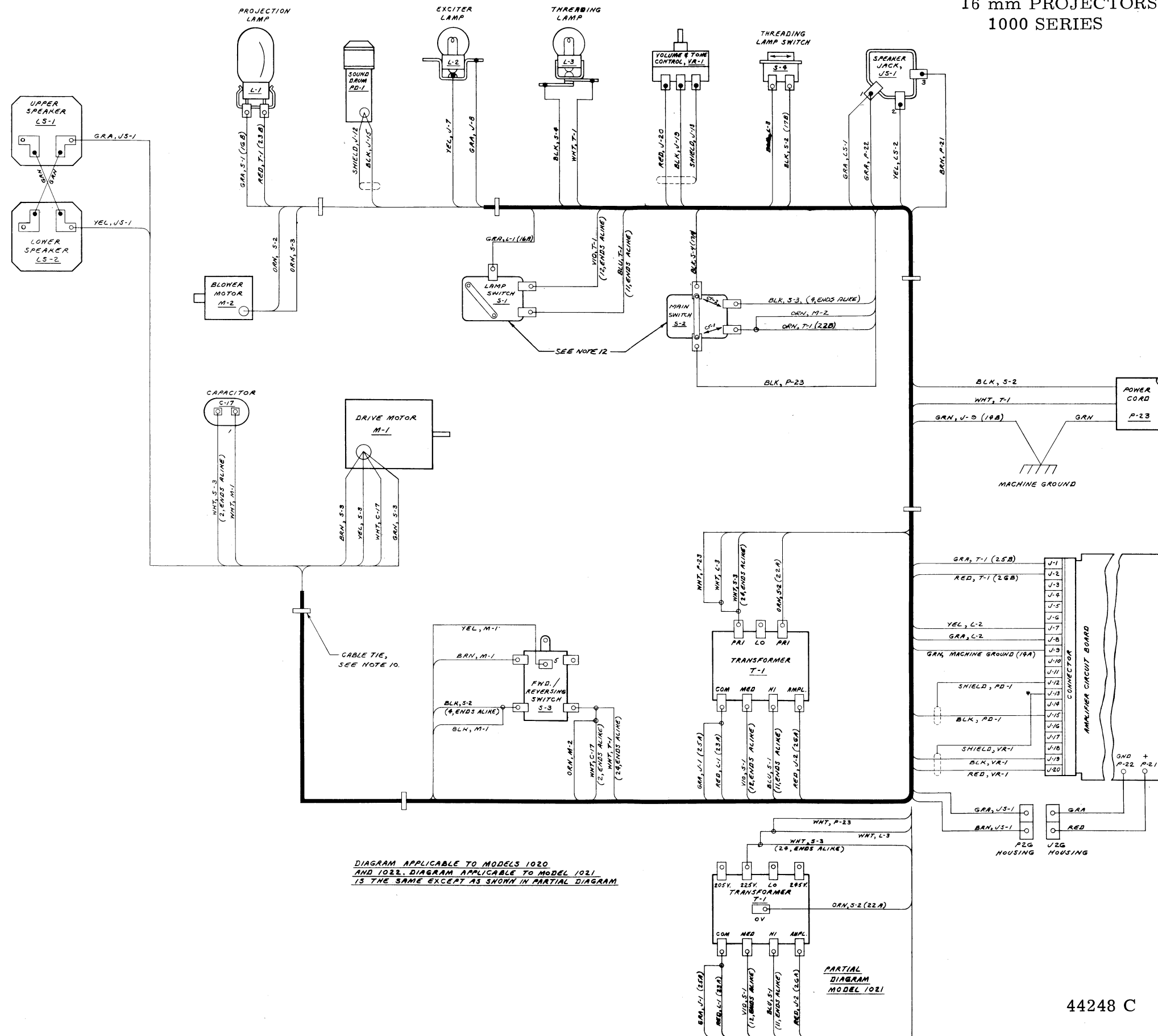
Figure 6-10. PROJECTOR WIRING DIAGRAM (Models: 1020, 1021, 1022)
