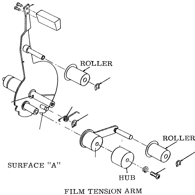
Figure 3-10. REASSEMBLY OF THREADING CONTROL ARM
