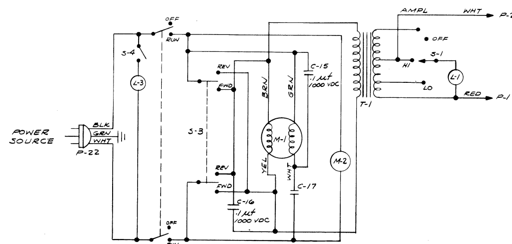
SCHEMATIC DIAGRAM H43947-2, PROJECTOR PORTION APPLICABLE TO MODELS 1000, 1015 AND 1016
