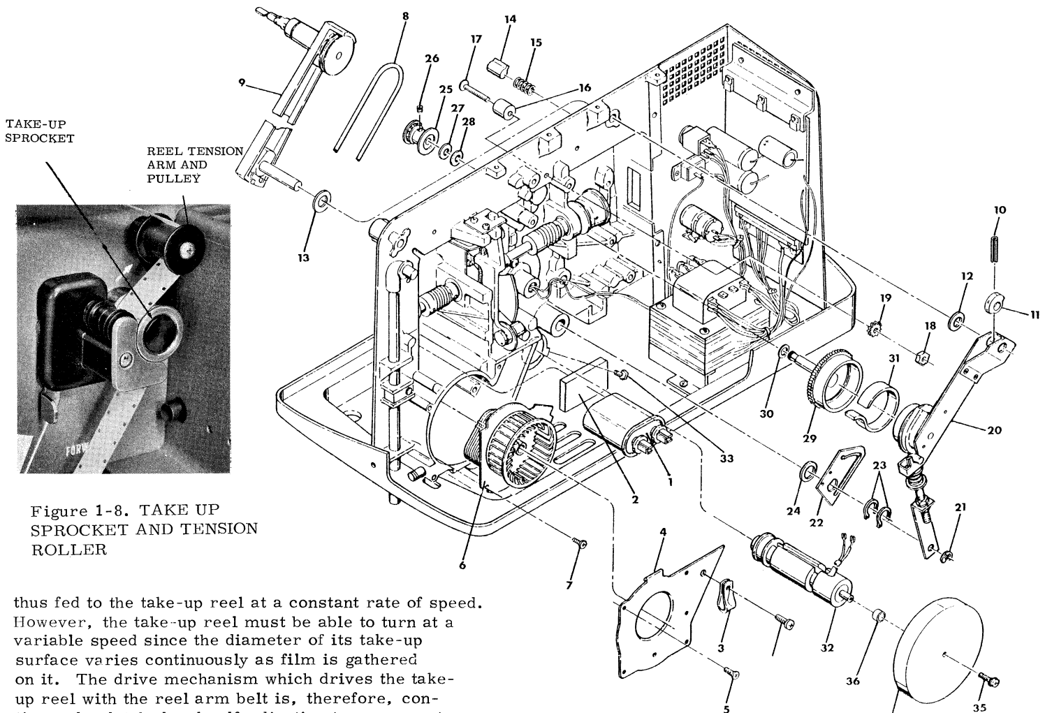
Figure 1-9. TAKE-UP CLUTCH
