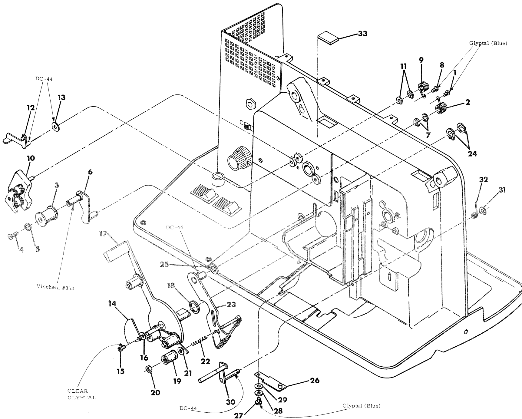
Figure 1-6. PROJECTOR ASSEMBLY (Stage V)
