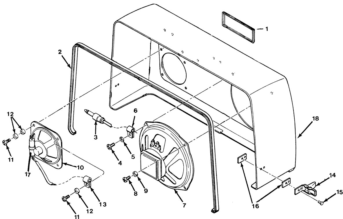
Figure 2-2. FRONT COVER ASSEMBLY W/SPEAKER
