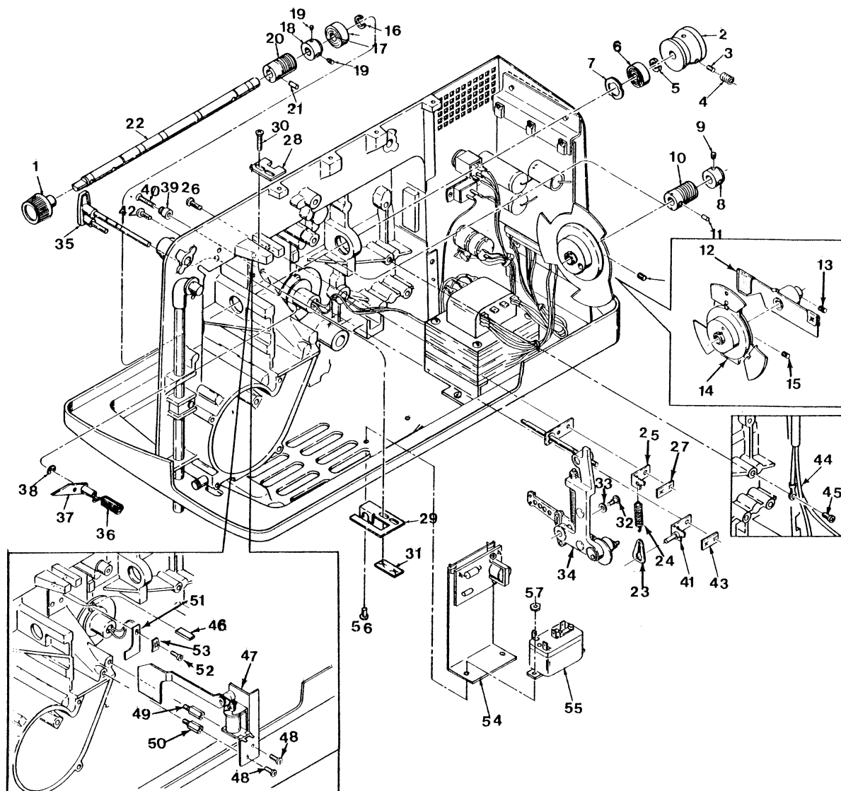
Figure 4-13. FRAMING ADJUSTMENT
