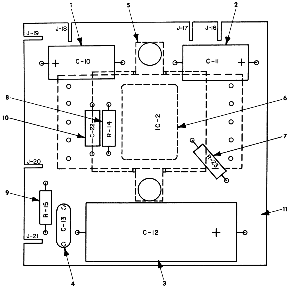
Figure 2-25 POWER AMPLIFIER BOARD ASSEMBLY
