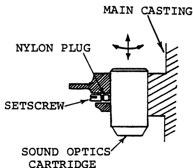
FOCUSING SOUND OPTICS CARTRIDGE
