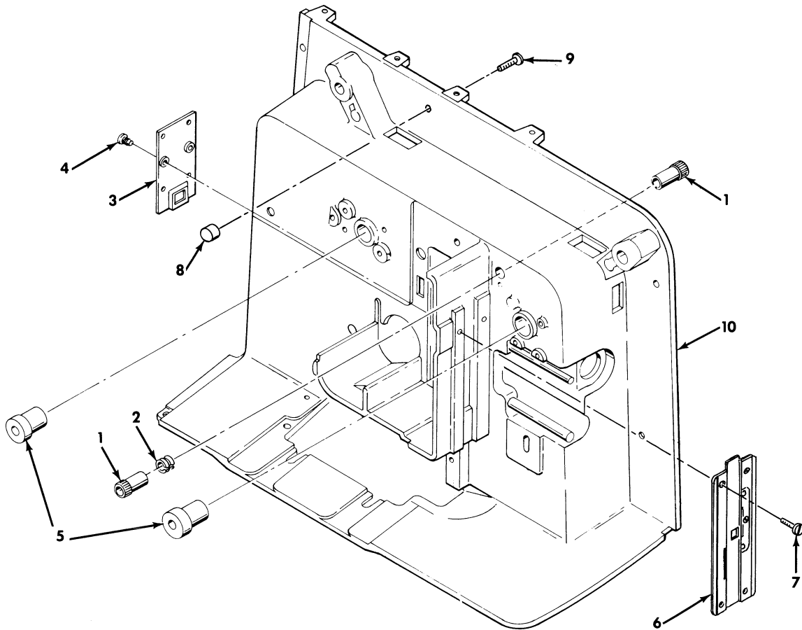
Figure 2-20. HOUSING ASSEMBLY
