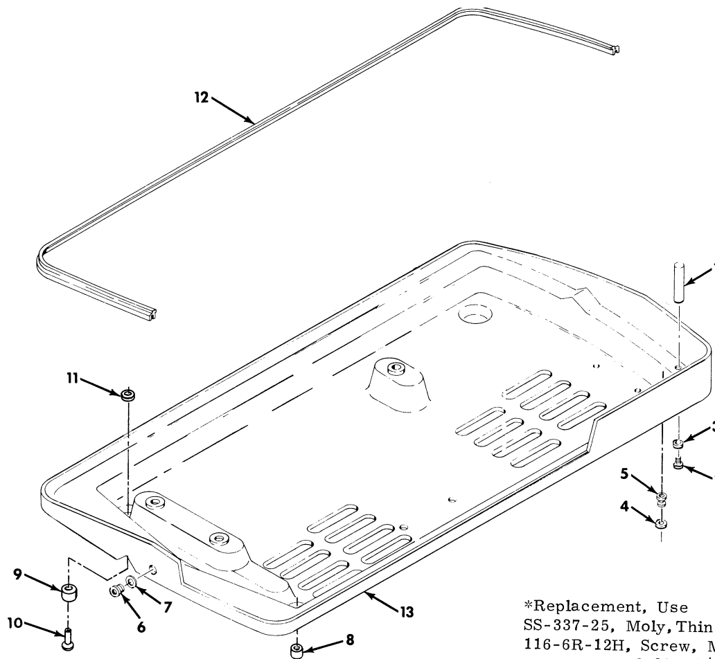
Figure 2-21. BASE ASSEMBLY
