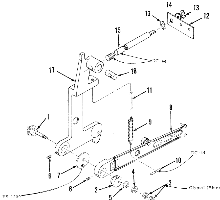
Figure 2-17. CLAW ARM COMPLETE
