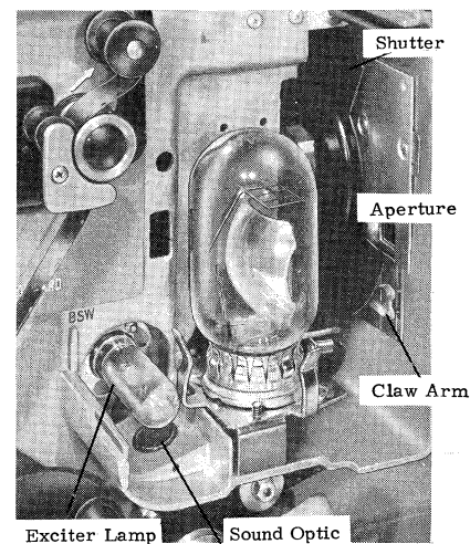
Figure 1-6. CLAW ARM AND SHUTTER
