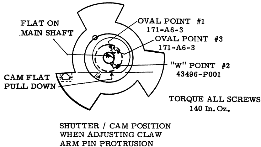
Figure 4-6. SHUTTER AND SHAFT ALIGNMENT
