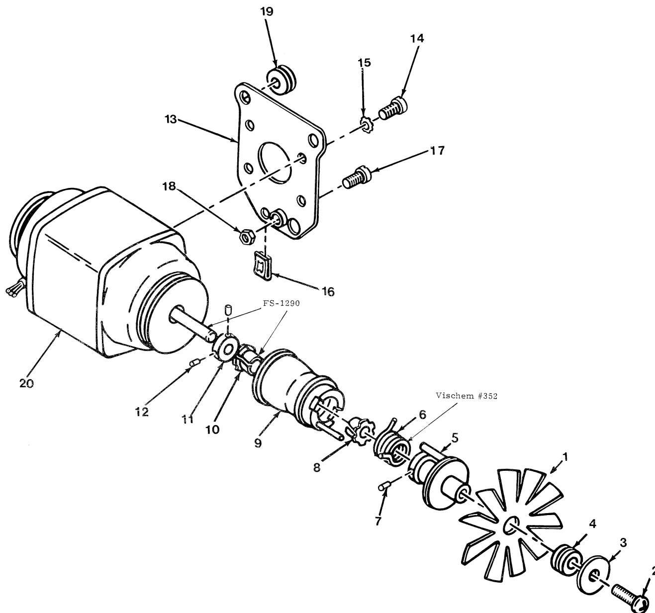
Figure 2-9. DRIVE UNIT ASSEMBLY
