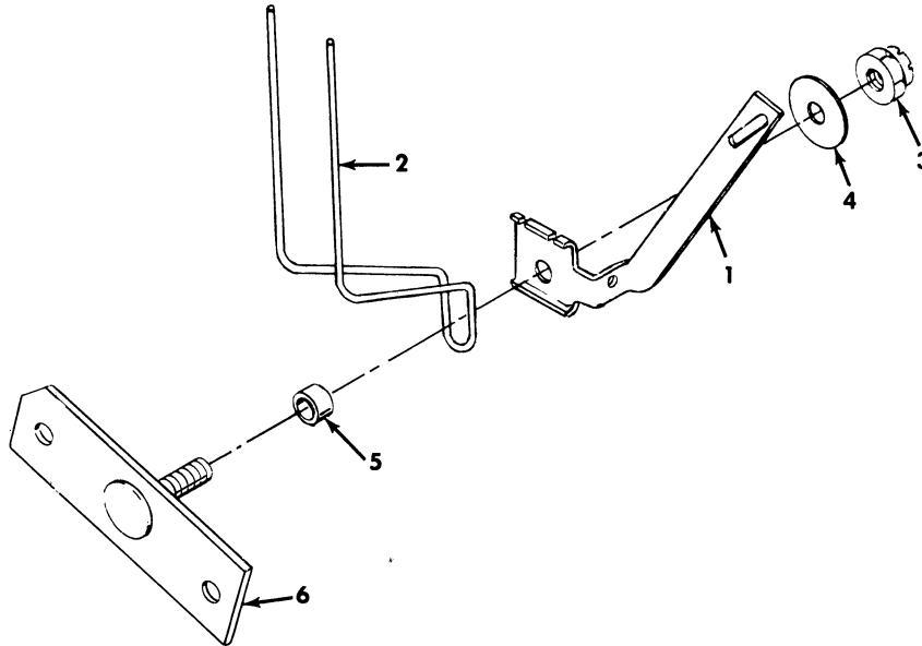
Figure 2-10. DRIVE BELT SHIFT FORK ASSEMBLY
