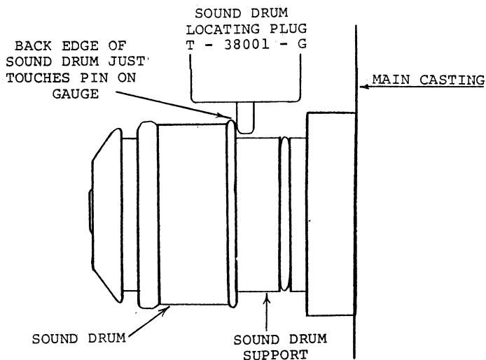
Figure 4-19. SOUND DRUM LATERAL POSITIONING
