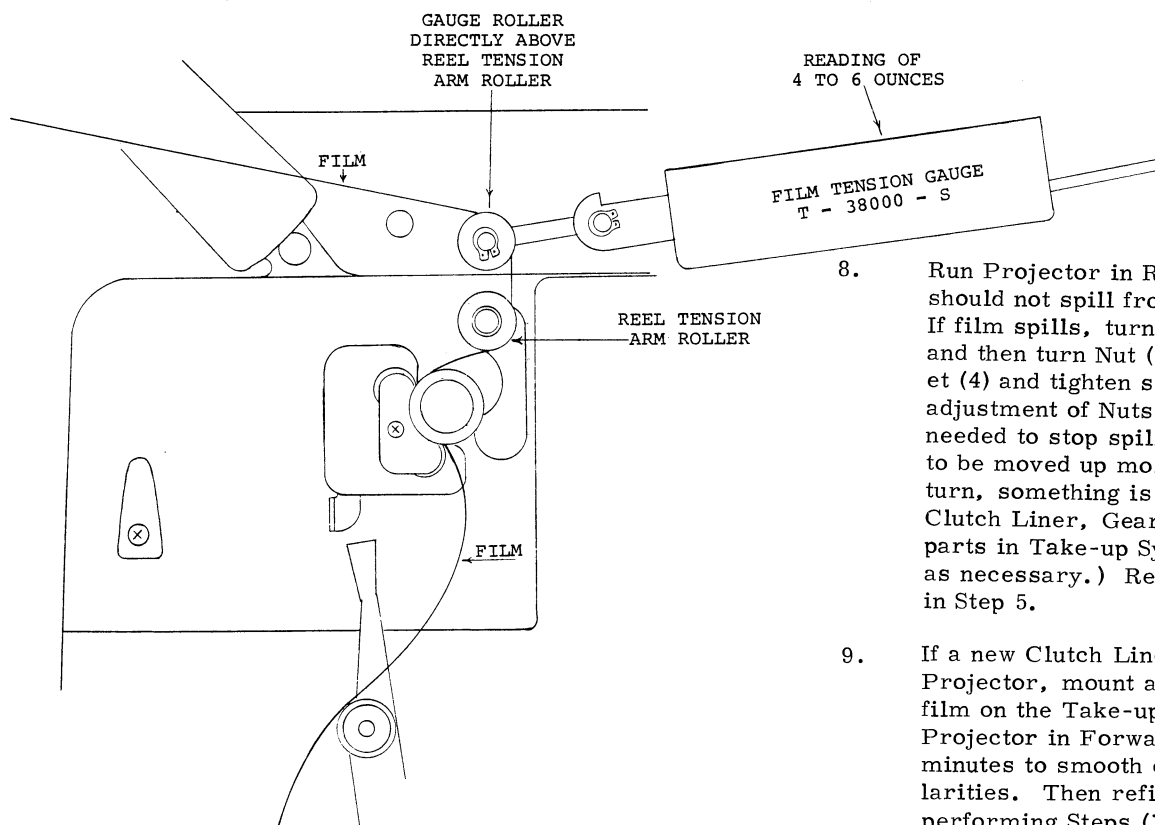
Figure 4-17. TAKE-UP TENSION MEASUREMENTS
