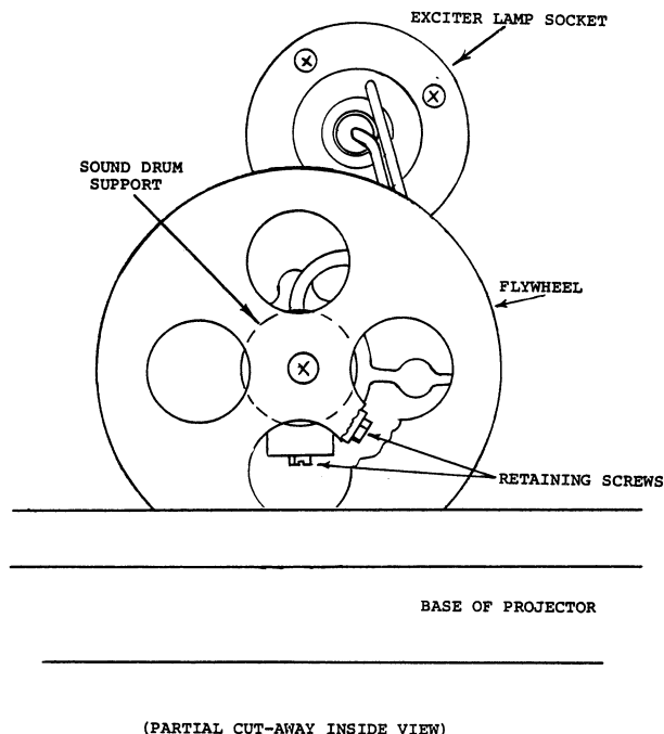
Figure 4-20. SOUND DRUM SUPPORT RETAINING SCREWS.
