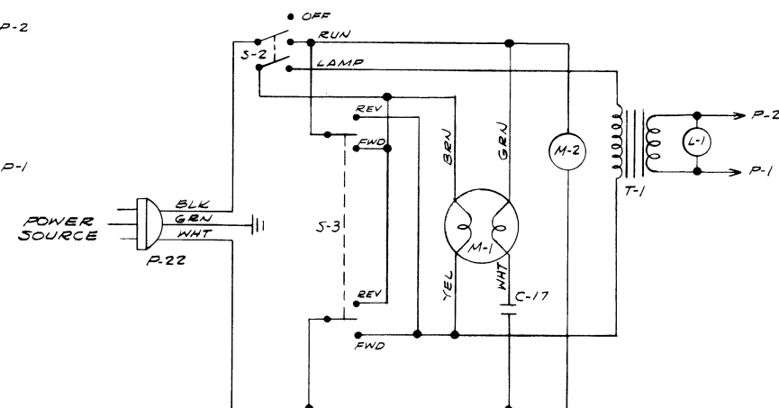
SCHEMATIC DIAGRAM H43947-3, PROJECTOR PORTION. APPLICABLE TO MODEL 1050.
