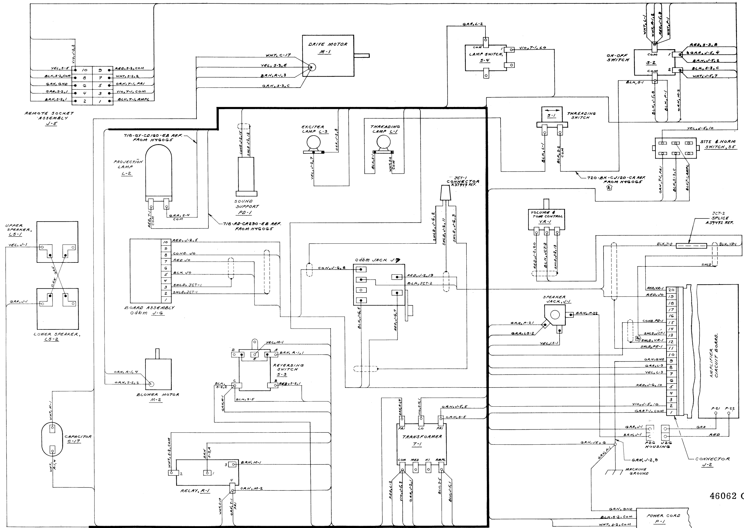
Figure 6-13. PROJECTOR WIRING DIAGRAM (Model: 1030N)
