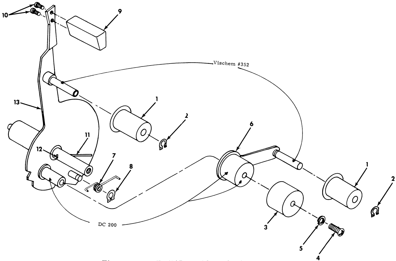
Figure 2-14. THREADING CONTROL ARM COMPLETE
