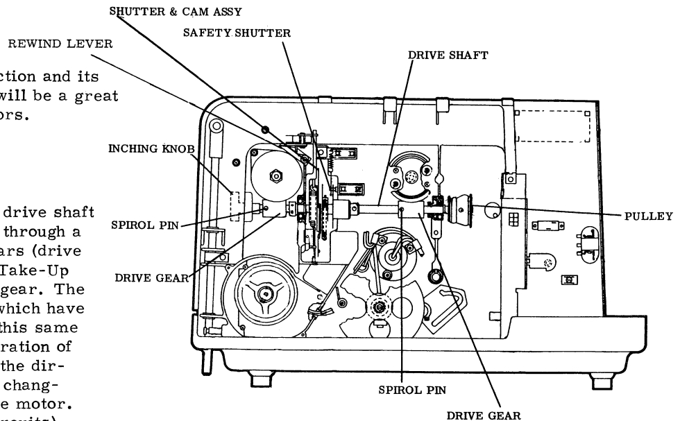
Figure 1-1. MAIN DRIVE SYSTEM
