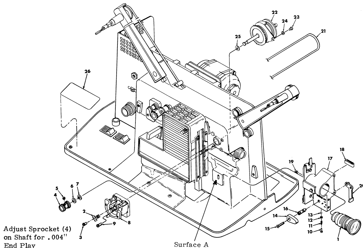
Figure 3-1. DISASSEMBLY AND REASSEMBLY FEED AND REWIND CLUTCH
