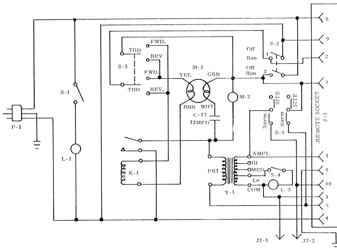
Figure 1-13. POWER SUPPLY AND MOTOR DRIVE CIRCUIT - Model 1030N
