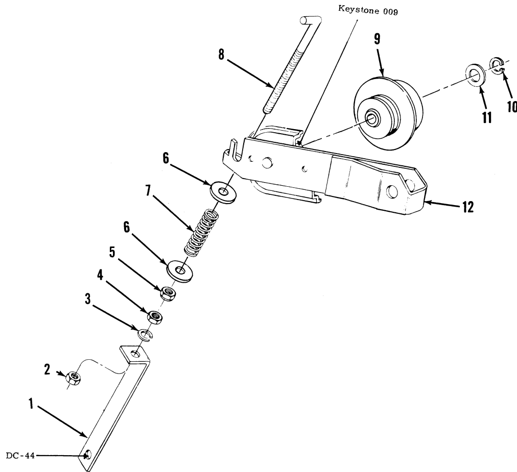
Figure 2-12. TAKEUP CLUTCH ARM COMPLETE
