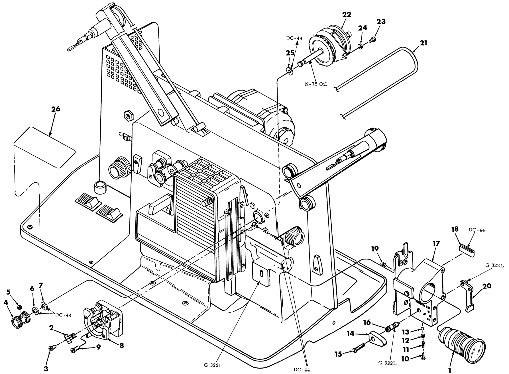
Figure 1-2. PROJECTOR ASSEMBLY (Stage I).
