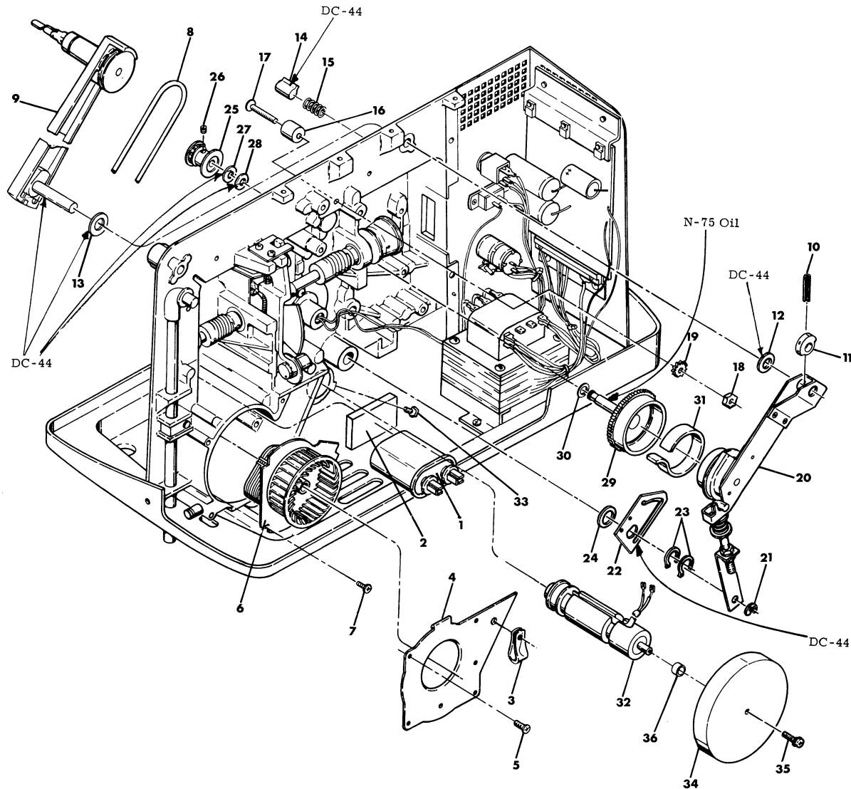
Figure 1-5. PROJECTOR ASSEMBLY Stage IV
