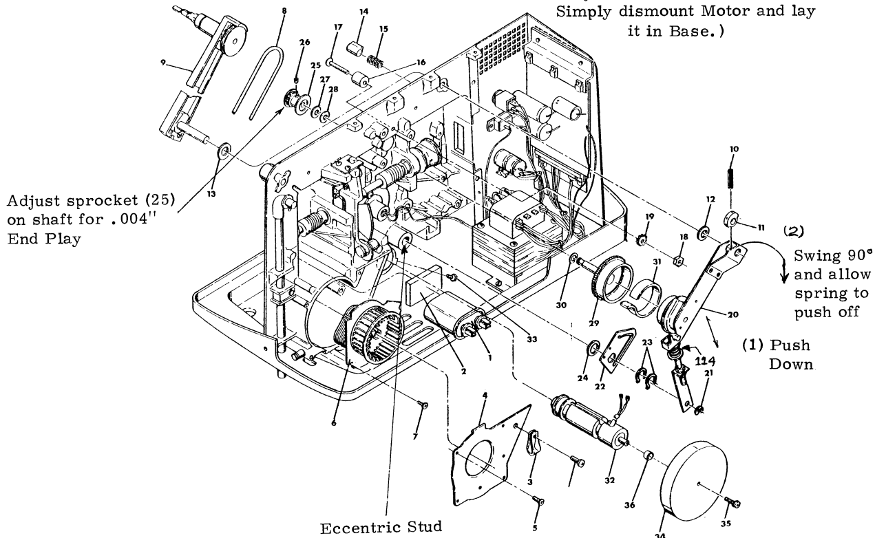
Figure 3-2. DISASSEMBLY AND REASSEMBLY TAKE-UP CLUTCH
