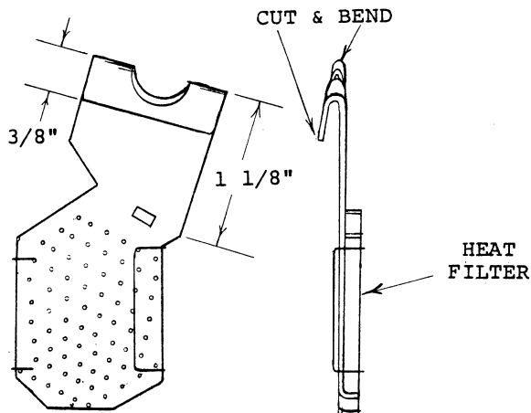
Figure 4-12. MODIFIED SAFETY SHUTTER (42994-G1)
