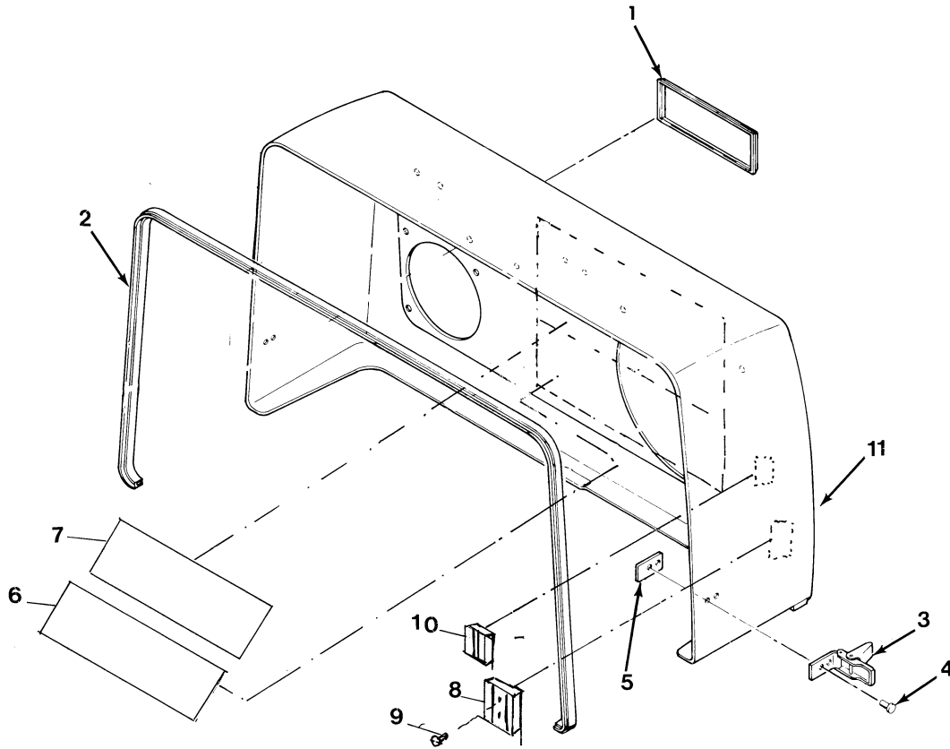
Figure 2-1. FRONT COVER ASSEMBLY.
