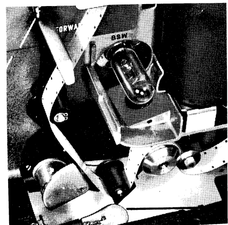
Figure 1-7. SOUND DRUM AND OPTIC
