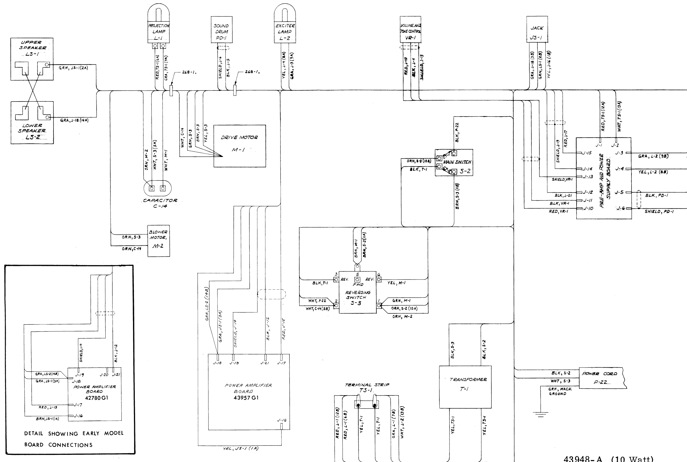
Figure 6-6. PROJECTOR WIRING DIAGRAM (Model: 1050)
