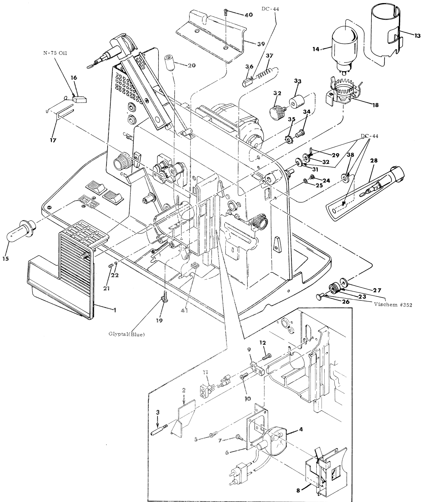
Figure 1-3. PROJECTOR ASSEMBLY (Stage II)
