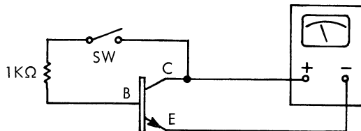
Figure 5-1. TEST CIRCUIT
