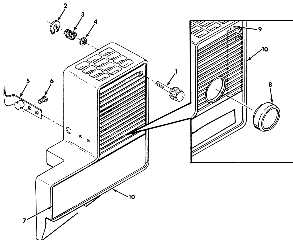
Figure 2-7. LAMPHOUSE COVER ASSEMBLY
