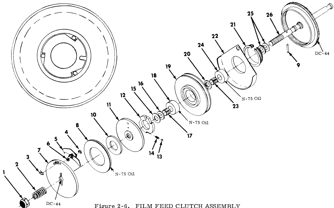
Figure 2-6. FILM FEED CLUTCH ASSEMBLY
