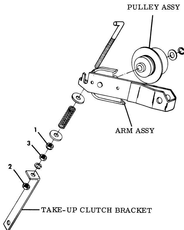
Figure 3-13. TAKE-UP CLUTCH ARM COMPLETE
