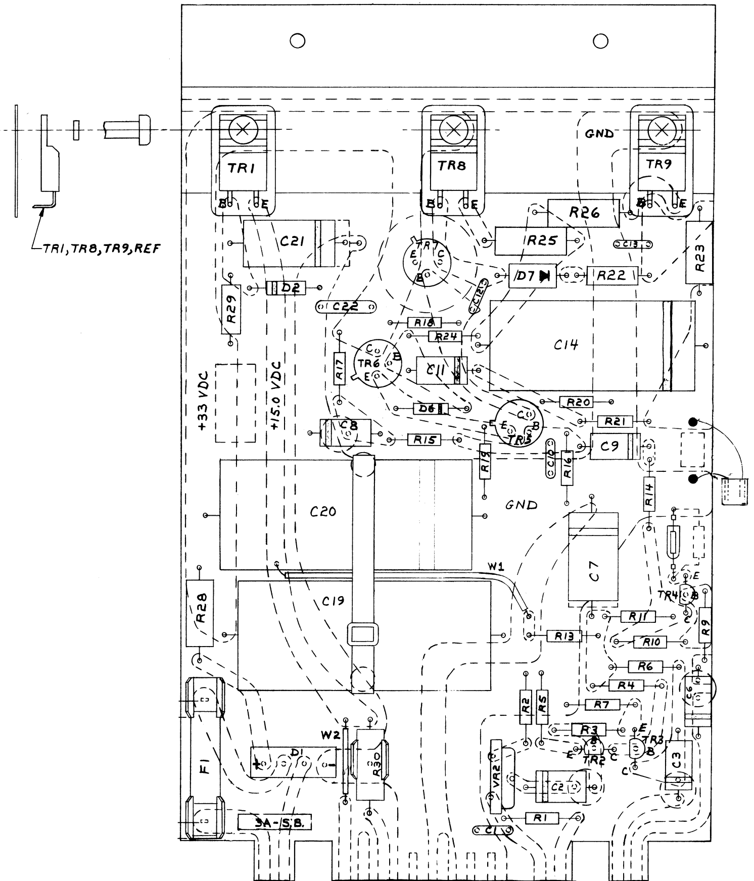
Figure 2-23. AMPLIFIER BOARD ASSEMBLY.
