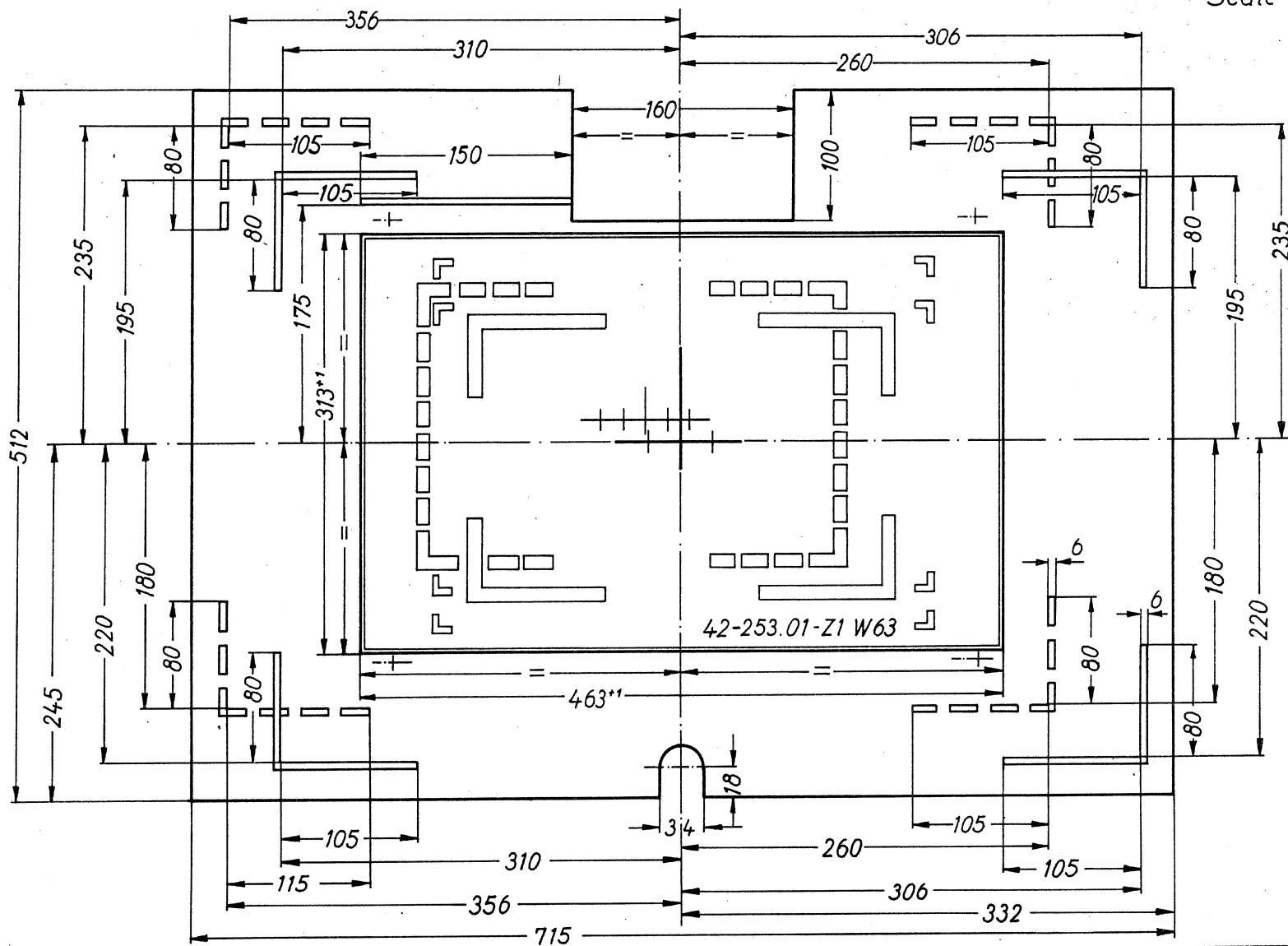
Fig. 30.1 Scale 1:4
