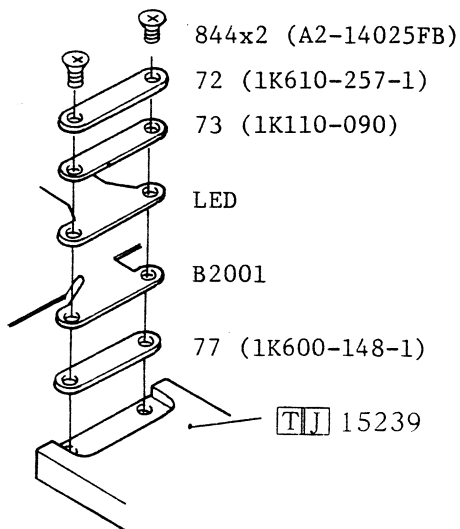
Fig.3-4 FPC retainer
