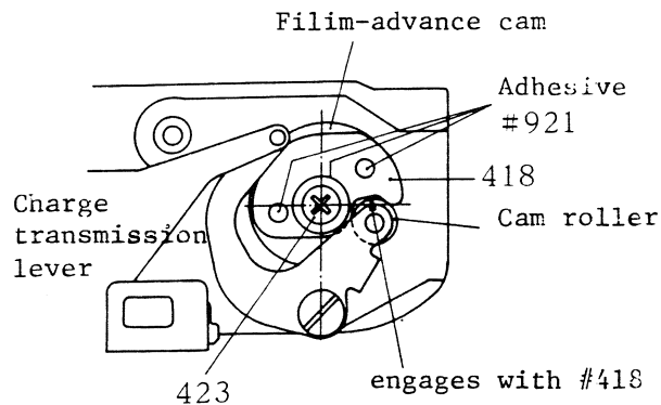
Fig 4-1 Film-advance timing adjustment
