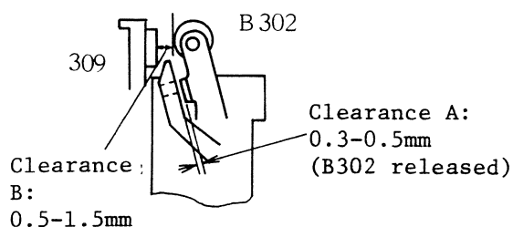
Fig.7-2 Mirror actuating lever
