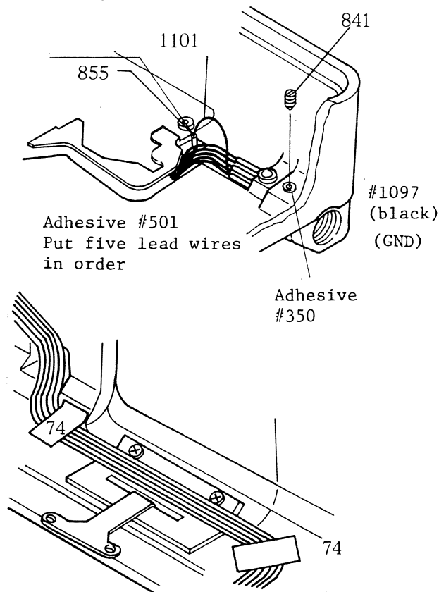
Fig.8-2 Sync terminal wires
