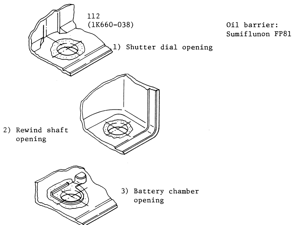
Fig.2-1 Oil barrier application
