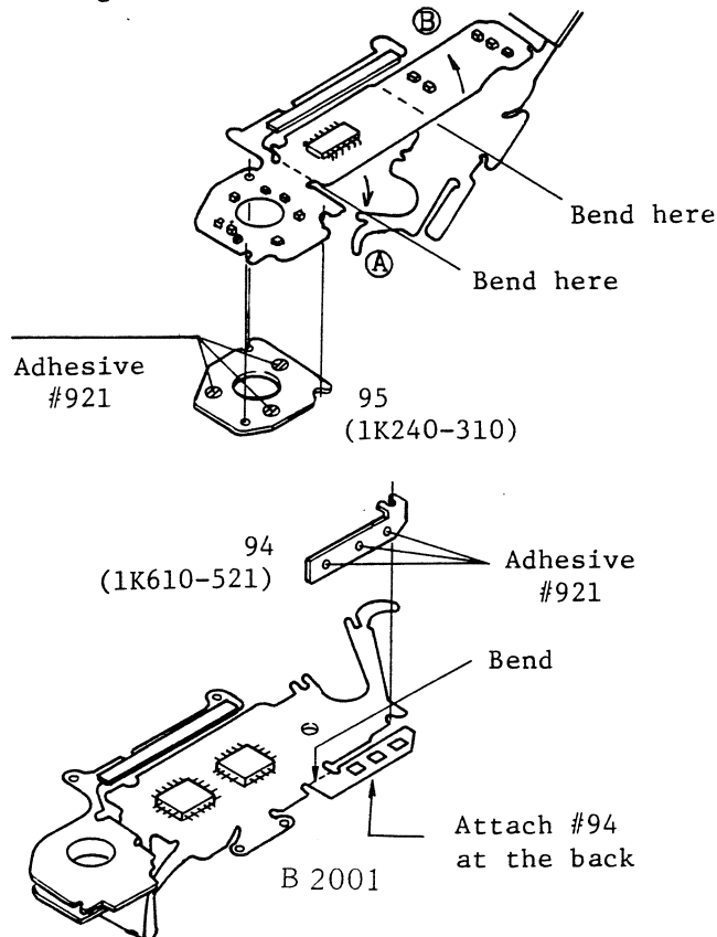
Fig.3-1 FPC installation 1
