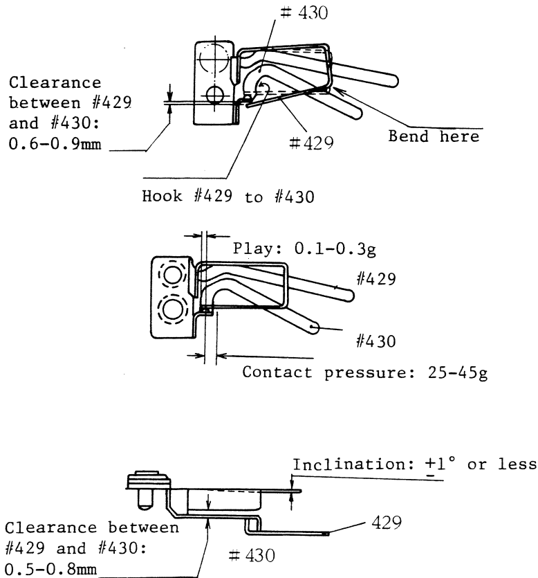
Fig.6-1 Release button switch
