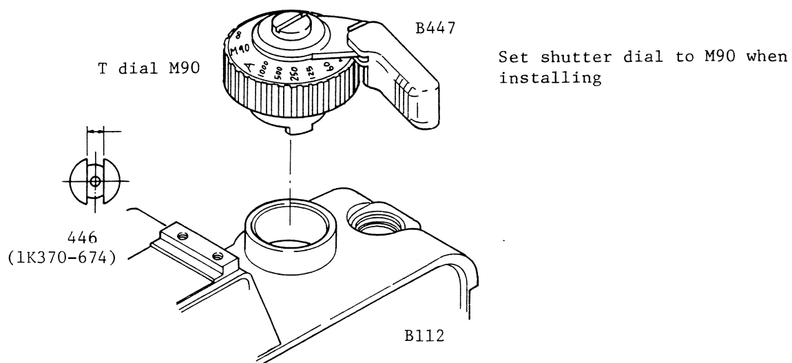
Fig.2-2 Shutter dial/film-advance lever installation
