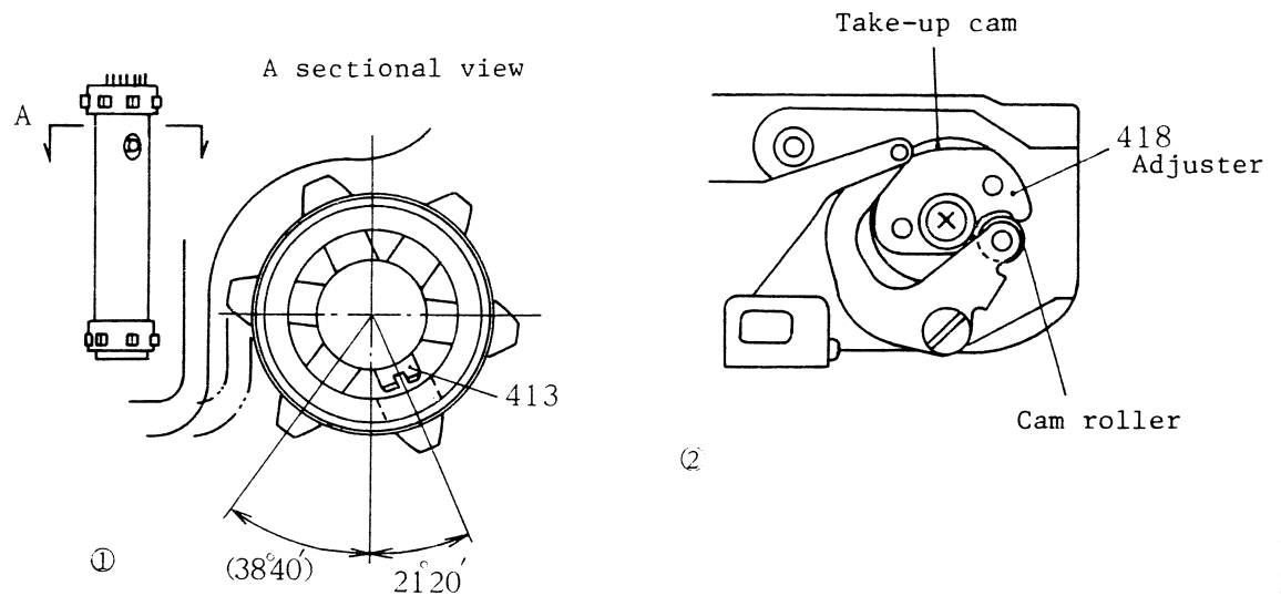
Fig.5-1 Film-advance unit
