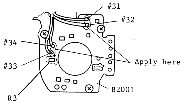
Fig.3-4 FPC retainer
