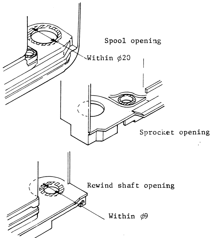
Fig 4-2 Oil barrier application
