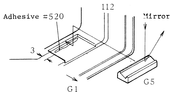
Fig.8-4 Mirror G5 installation
