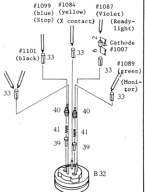
Fig.8-3 Sync terminal
