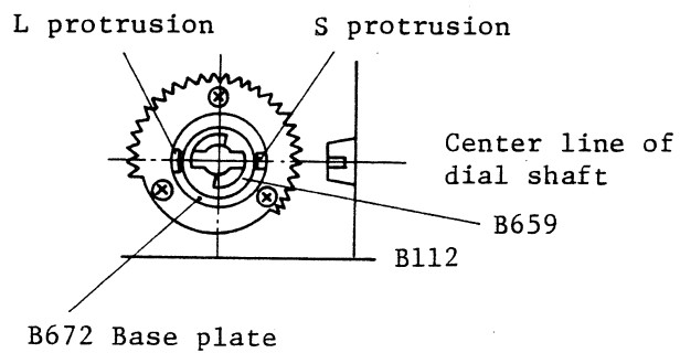
Fig.2-3 ASA/ISO dial installation
