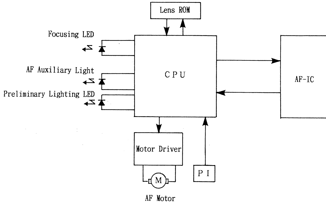
AF Control block Diagram
