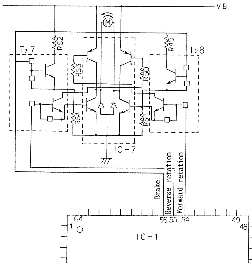
Sequence motor drive circuit
