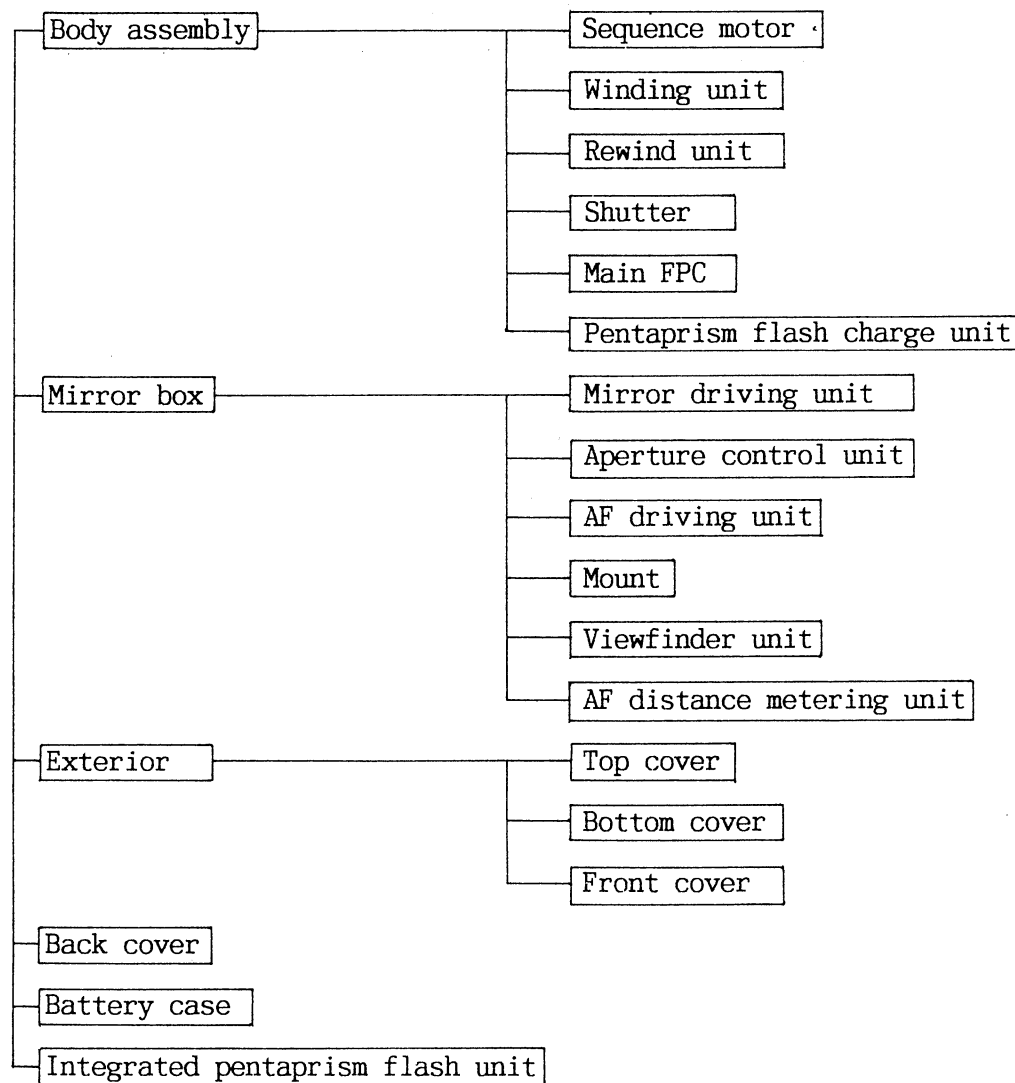
Mechanical System Diagram
