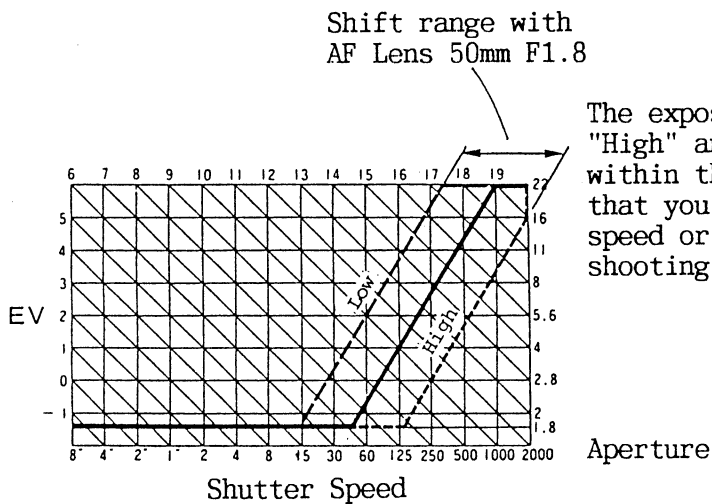
Program Shift Diagram (ISO 100)
