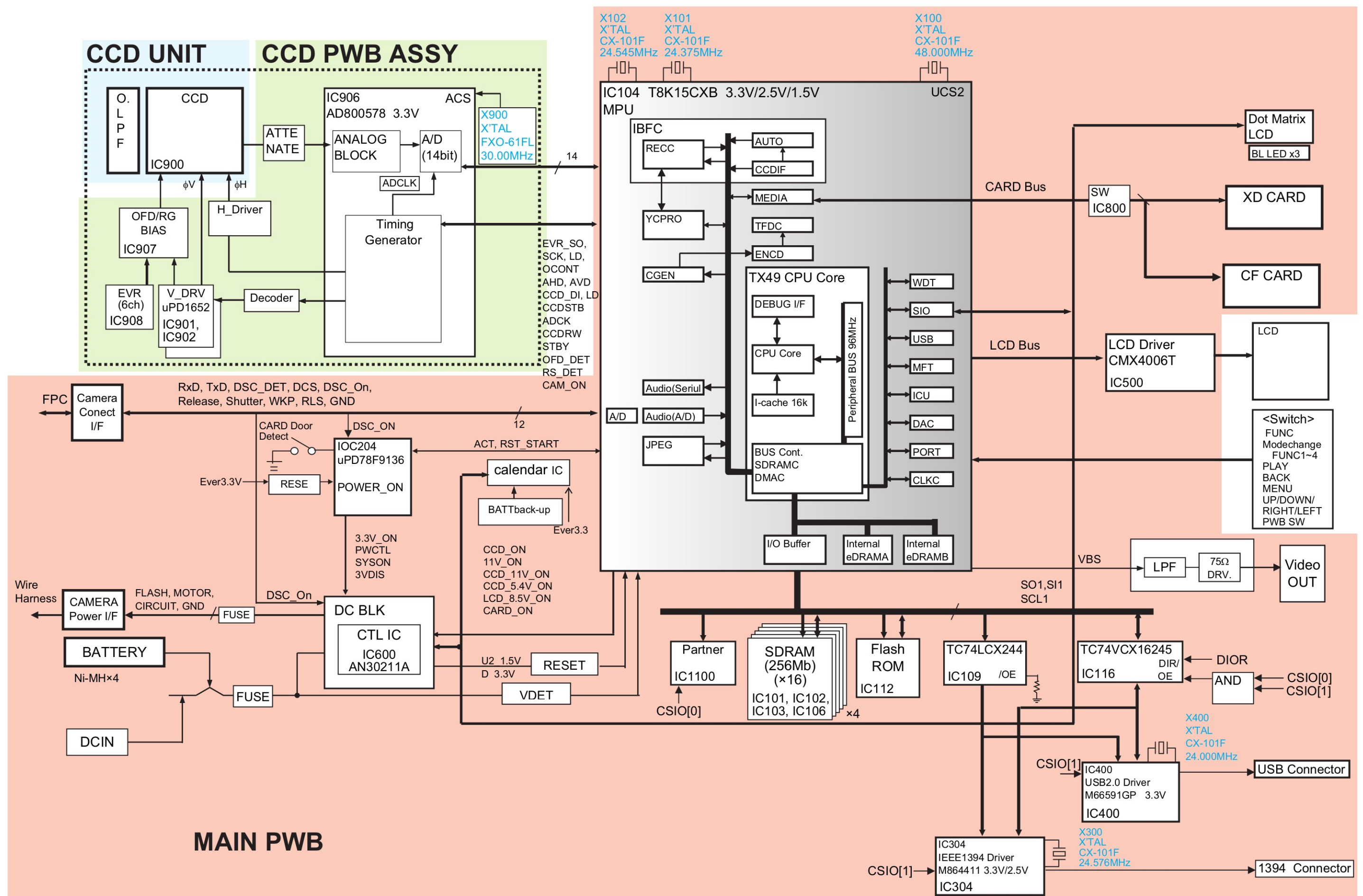
3-4. Block Diagram
