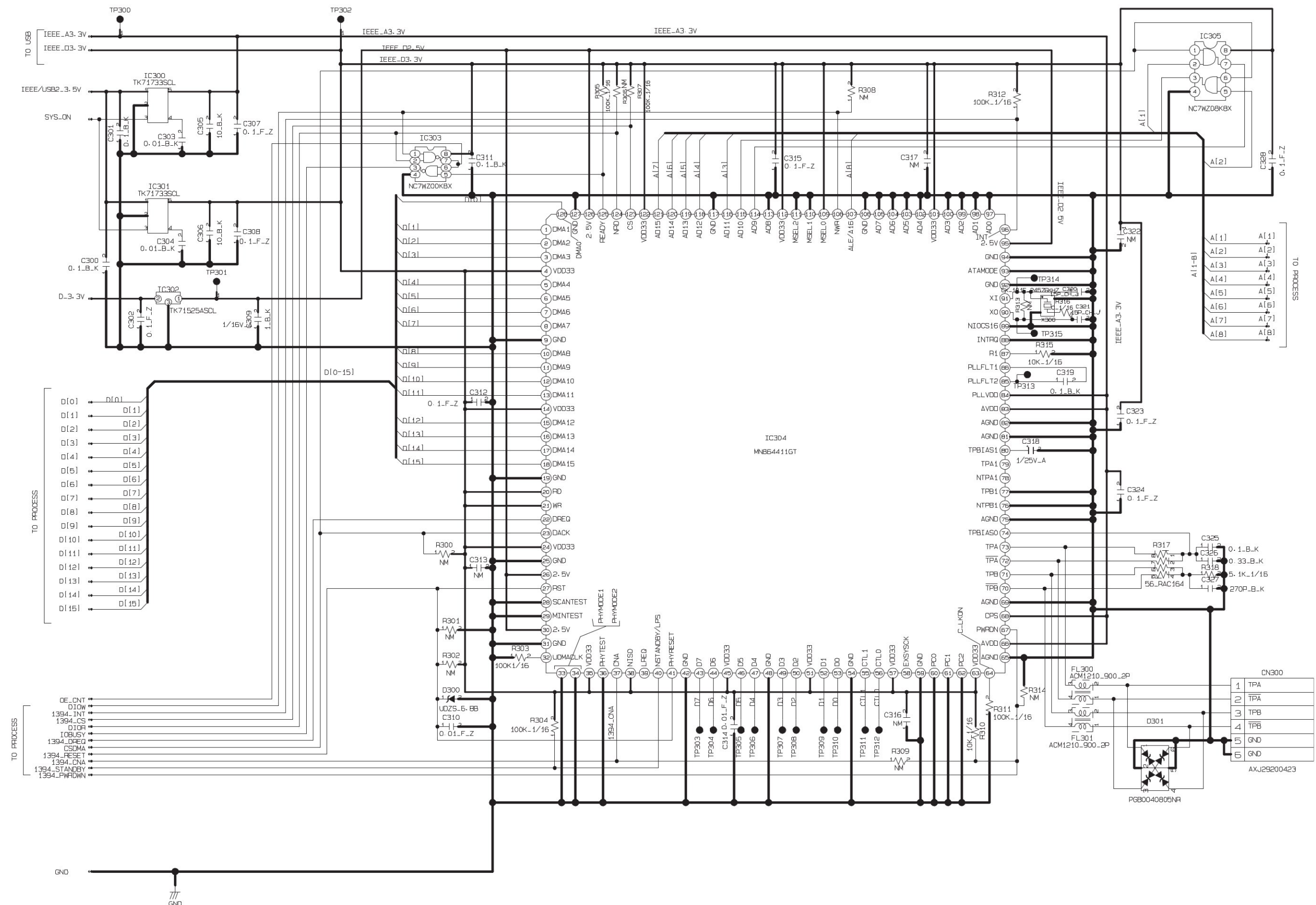
3-6-3. IEEE1394 BLOCK
