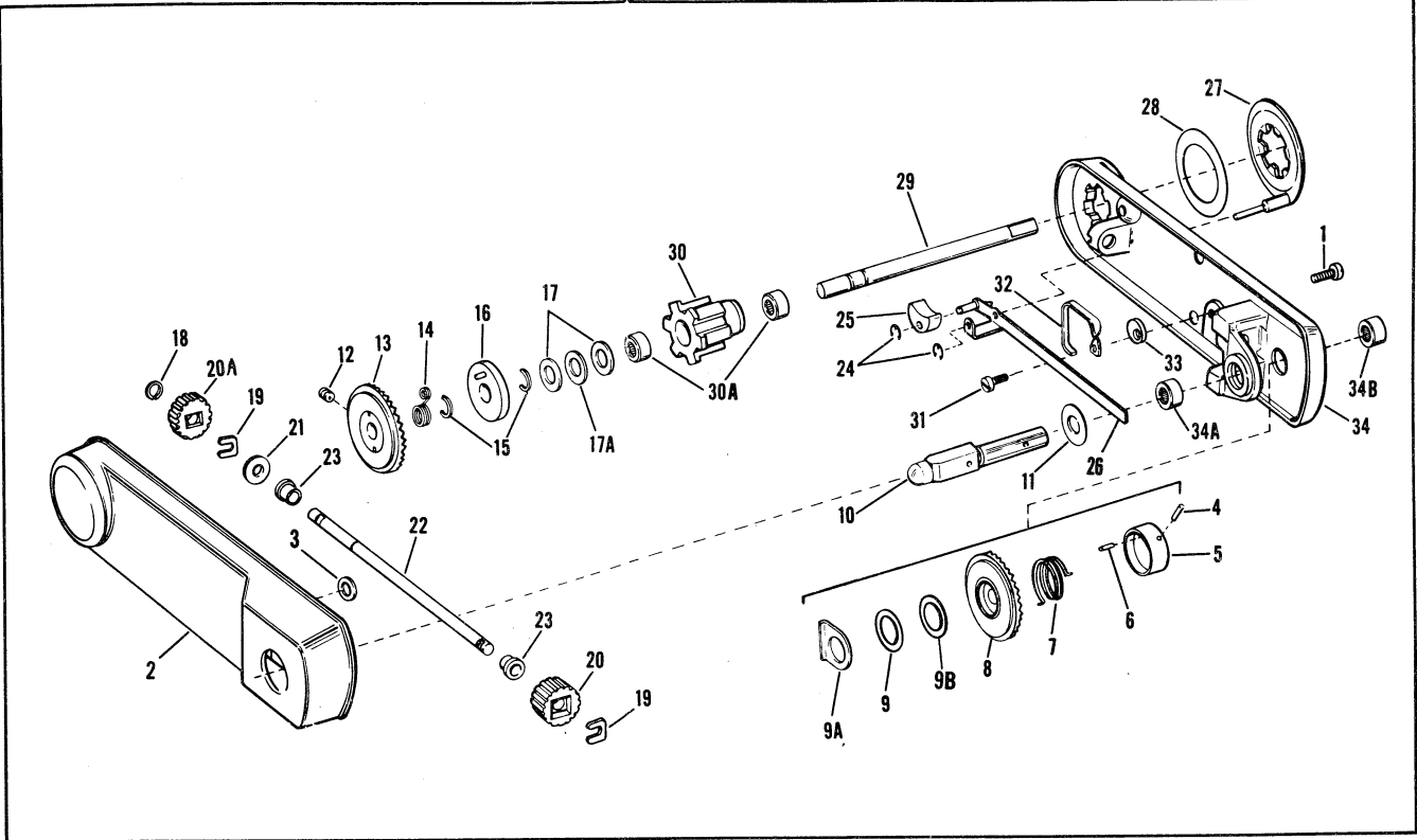
Figure 9. Front Reel Arm Assembly
