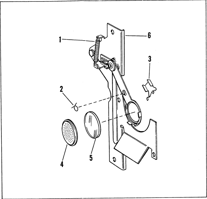
Figure 22. Fire Shutter Assembly (Code CDIJ only)
