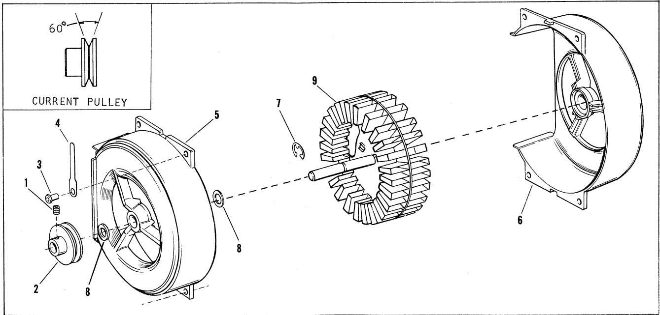
Figure 25A. Blower Assembly (Pressed Bearing Type)
