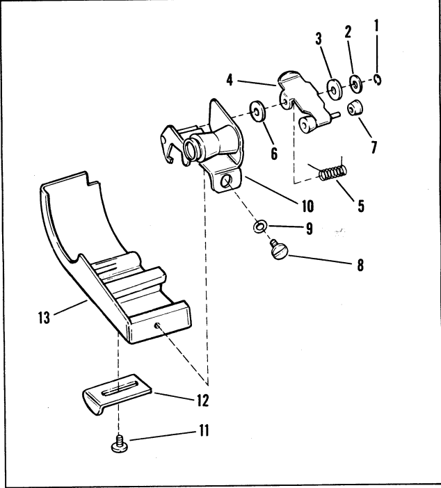
Figure 19A. Sprocket Guard Assembly (Interim 09897 Design)
