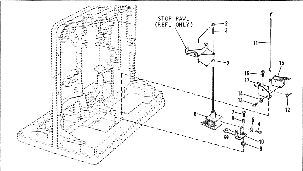
Figure 5. Solenoid Operated Clutch and Fire Shutter (Code C and D only)
