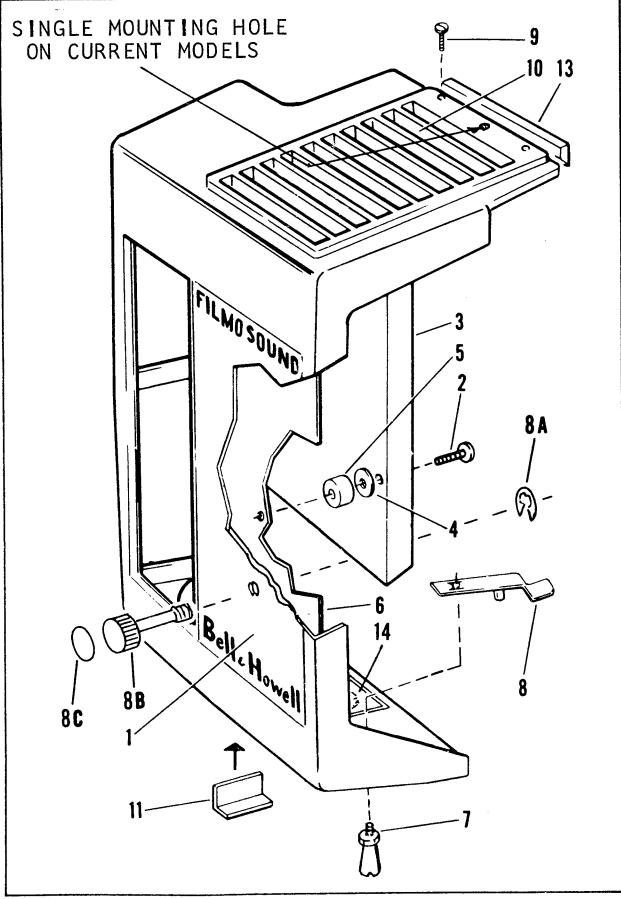
Figure 12. Lamphouse Assembly
