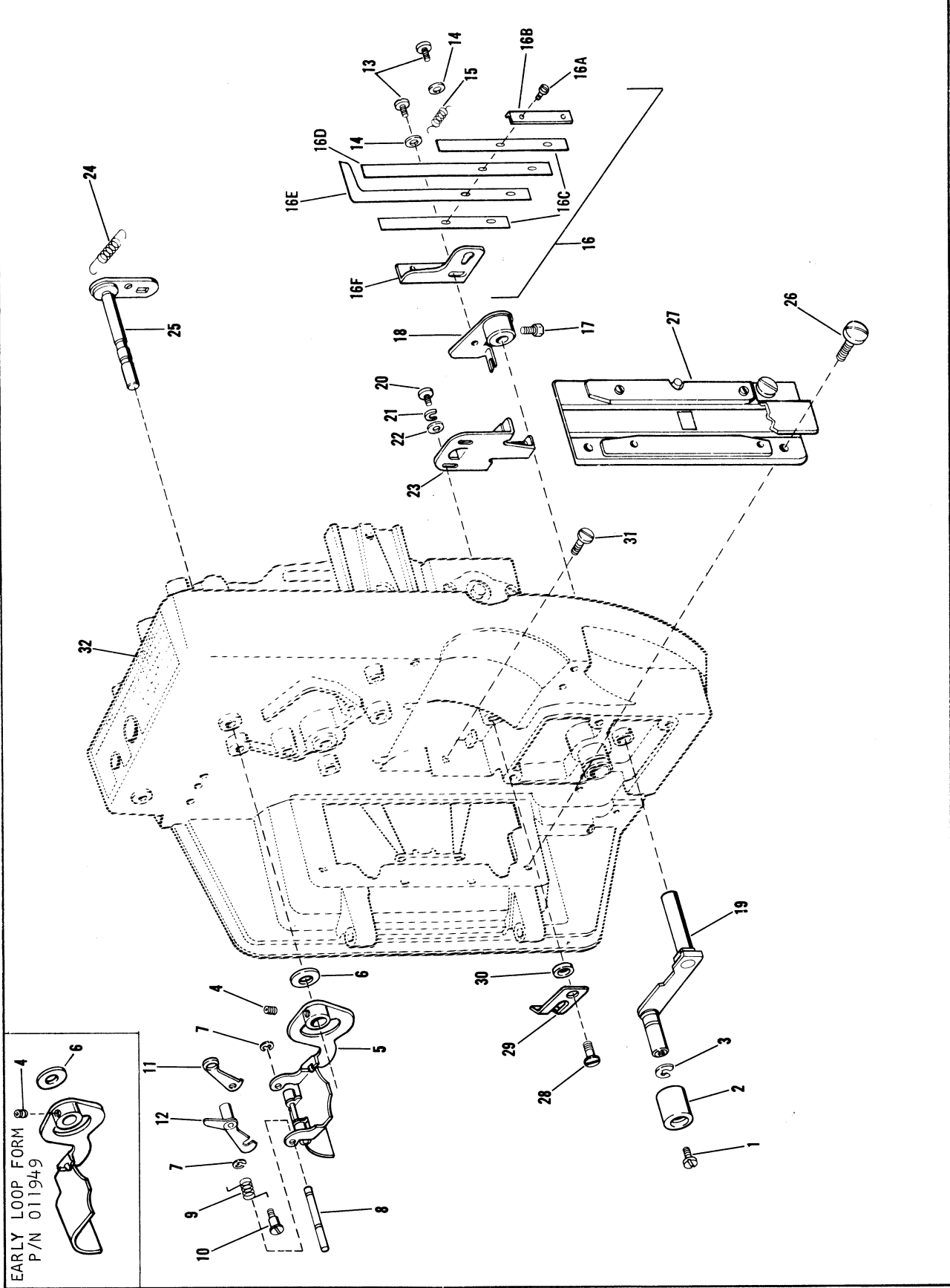
Figure 16. Mechanism Assembly (Cont'd)
