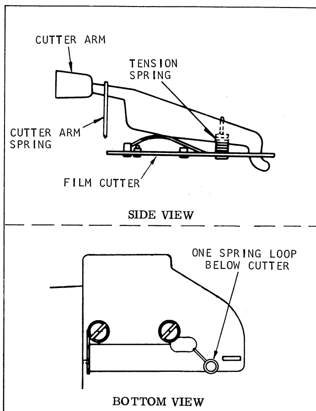
Figure J. Installing Film Cutter Parts
