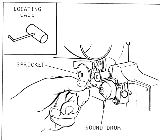
Figure W. Positioning the Soundhead Assembly
