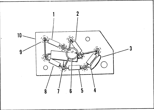
Figure 24. Preamplifier Assembly (Code ABCDE only)
