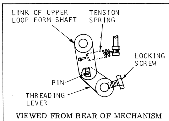
Figure T. Autoload System Adjustments — View I
