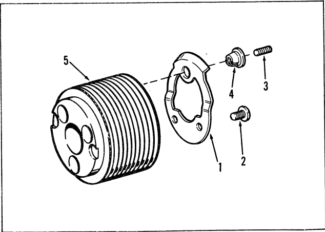
Figure 23. Worm Gear Assembly (Code CDIJ only)
