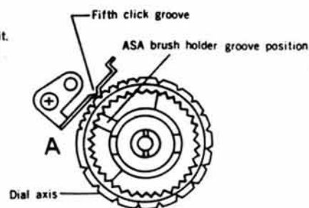
Fig. 19 ASA brush holder and dial axis setting position
