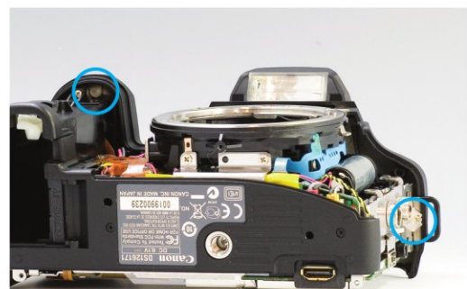
Fig. 030 The Position of the Top Cover Ass'y Screws (Bottom)
