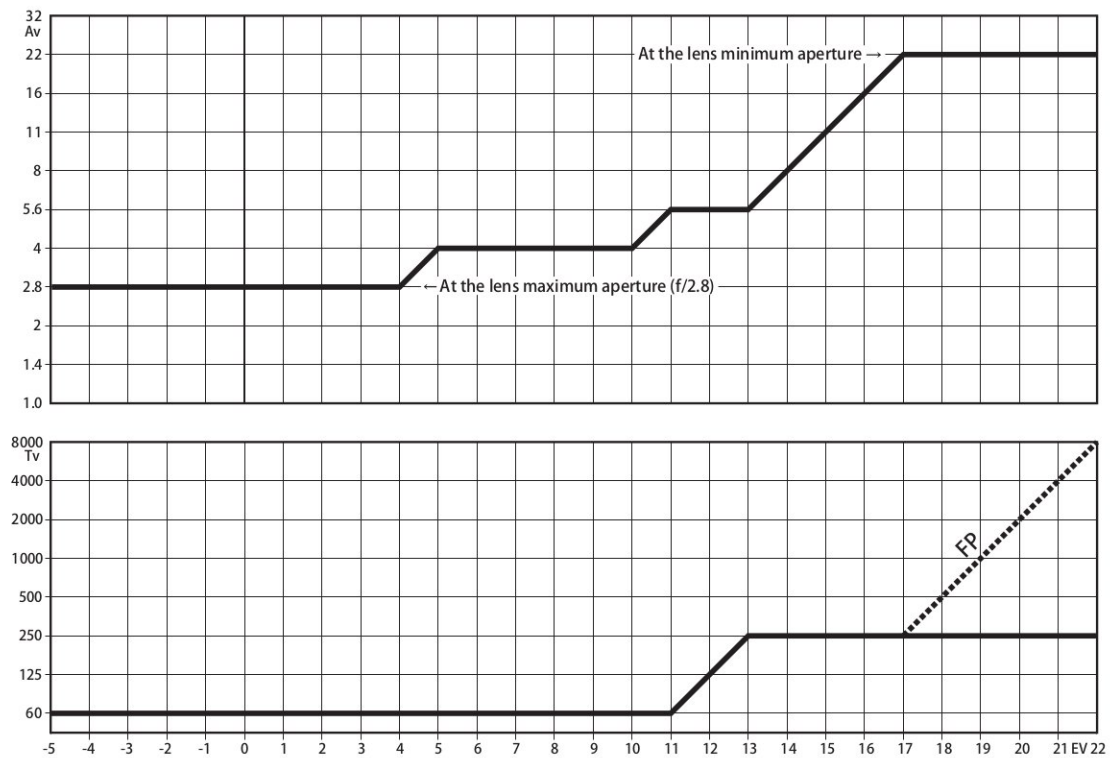
Fig. 039 E-TTL II autoflash program line (EF50mm f/1.4 USM, at ISO 100)
