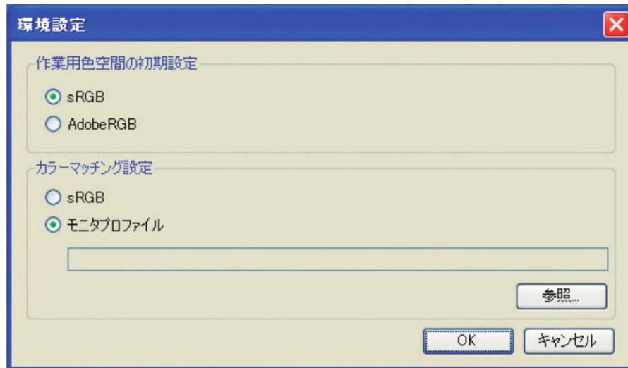
Fig. 003 Preferences window
