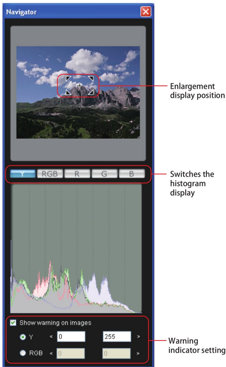
Fig. 006 Navigator window
