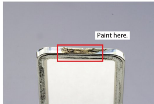
Fig. 033 Display Window Reassembly
