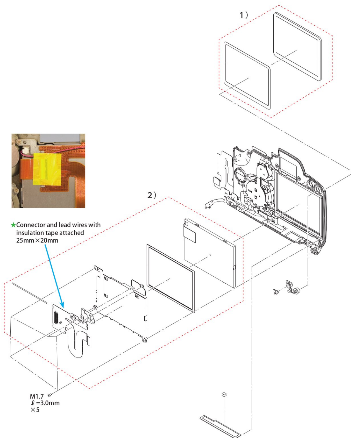
Fig. 082 Back Cover Ass'y Disassembly
