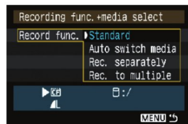
Fig. 009 Recording function
