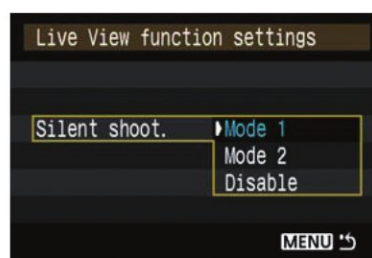
Fig. 024 Silent shooting
