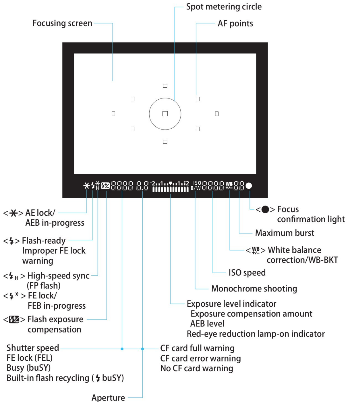
Fig. 035 Viewfinder Information
