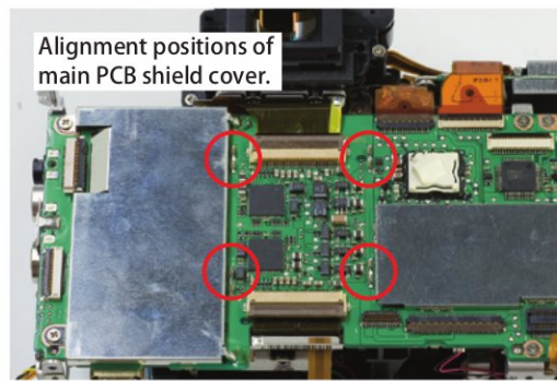
Fig. 055 Position for the Main PCB Shield Cover (on Main PCB Ass'y)
