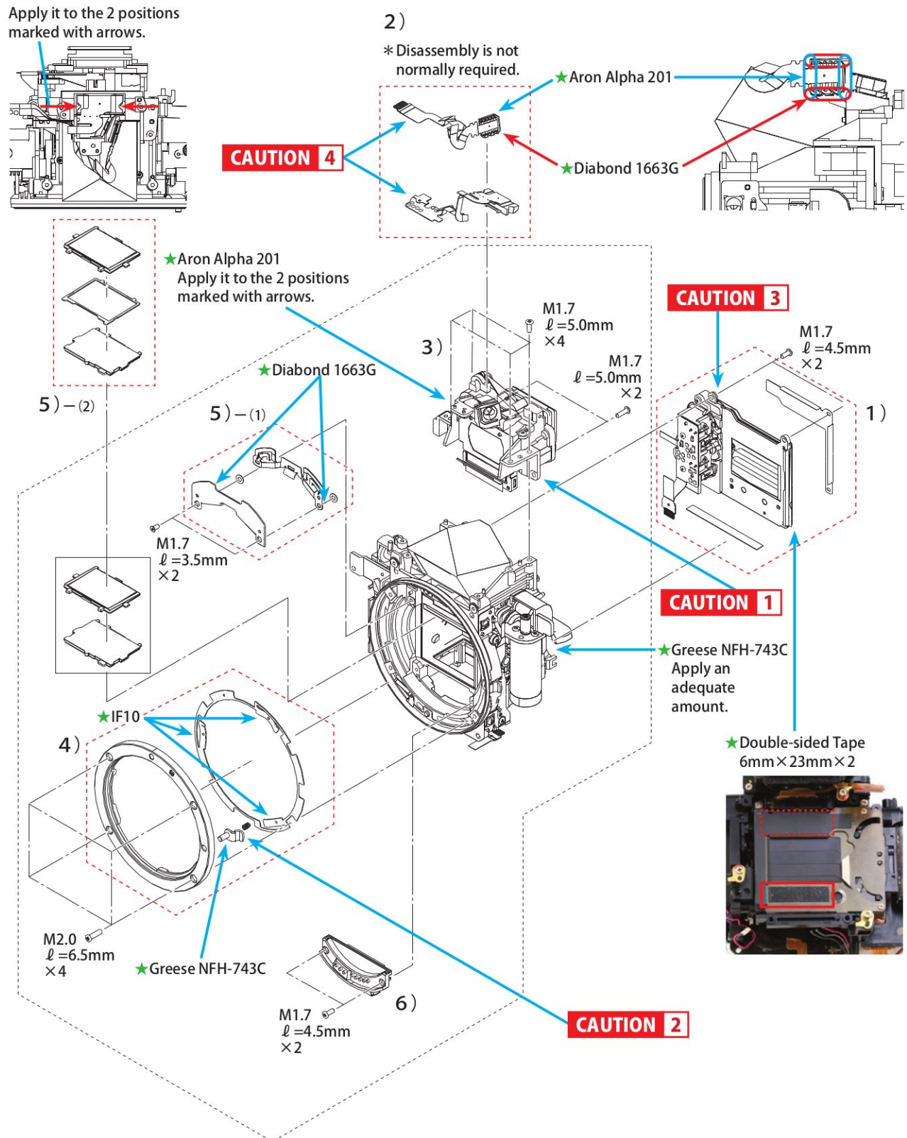
Fig. 072 Mirror Box Ass'y Disassembly
