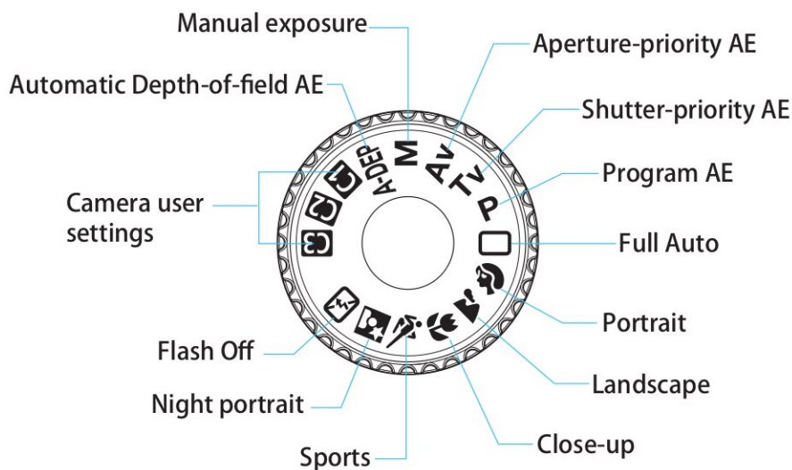
Fig. 037 Mode dial
