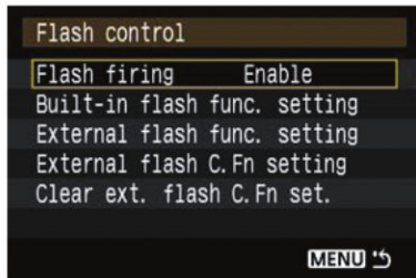
Fig. 017 Flash control
