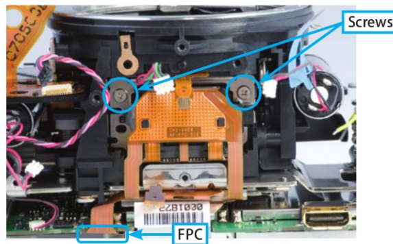
Fig. 041 Position of Screws and FPC of AF FPC Ass'y (Bottom)
