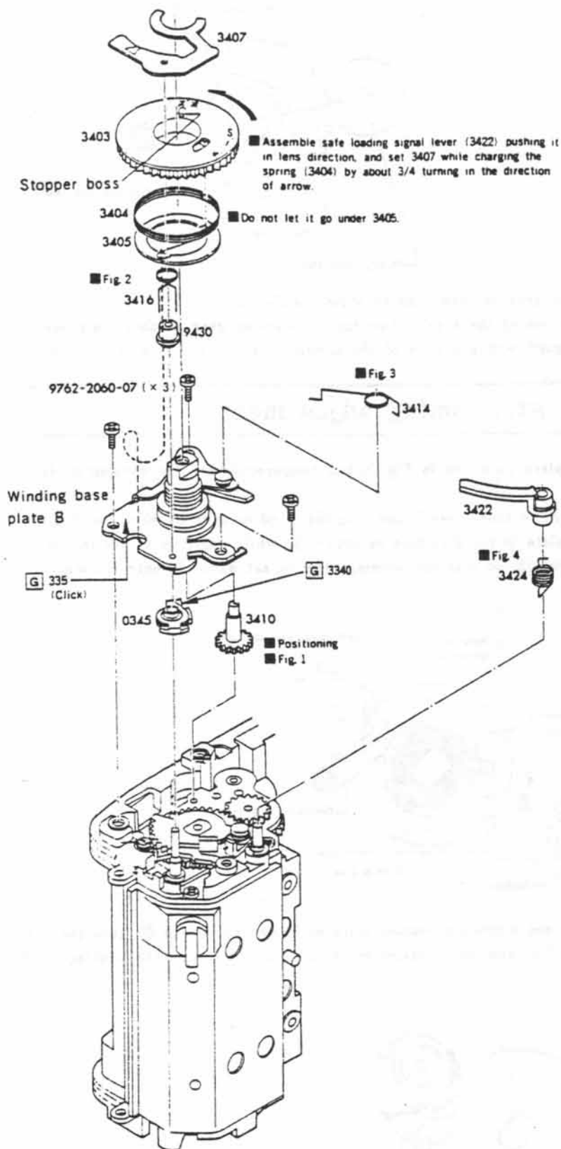
Fig. 2 3416 spring setting
