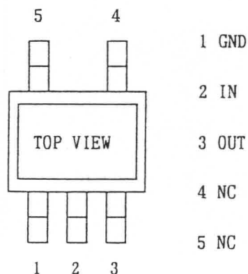
(IC102 Regulated DC Voltage IC Pin Arrangement)
