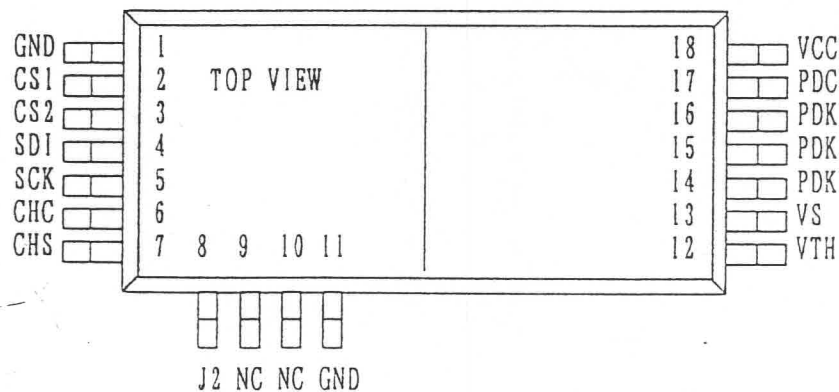
(IC401 TTL Flash Auto IC Pin Arrangement)
