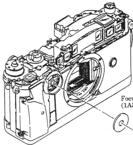
Focus Dial (1AS27010)
