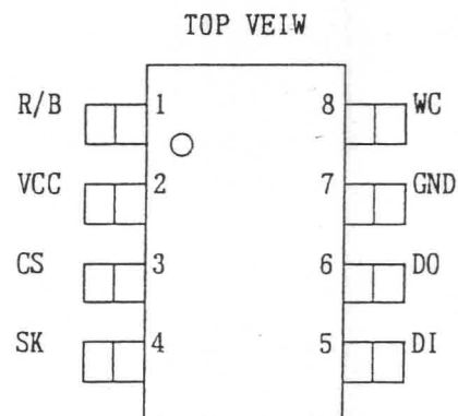
(IC151 EEPROM1 Pin Arrangement)
