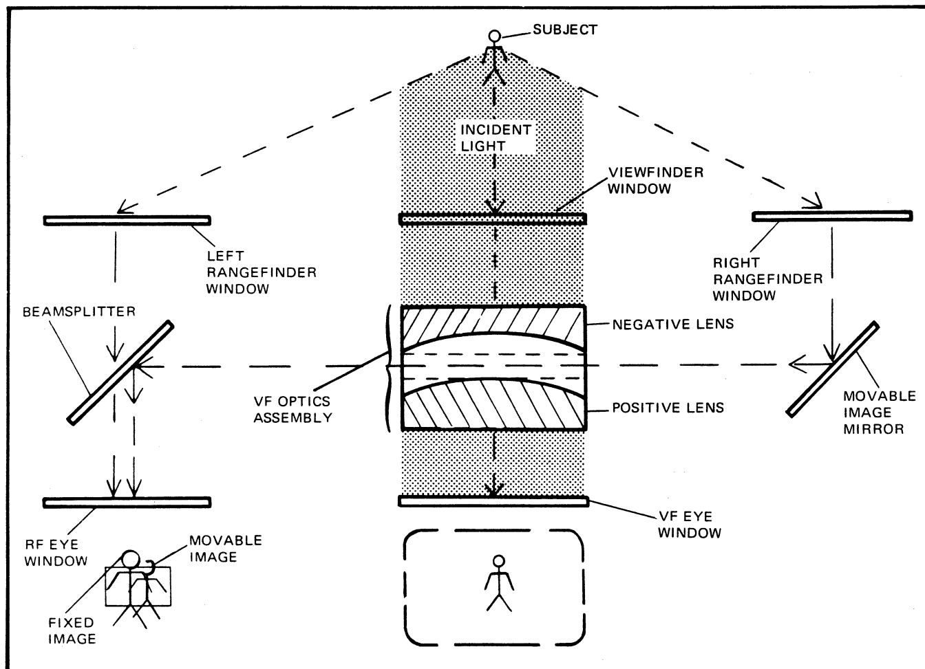
FIG. 2.8 POLAROID RANGEFINDER/VIEWFINDER INTERNAL CONFIGURATION
