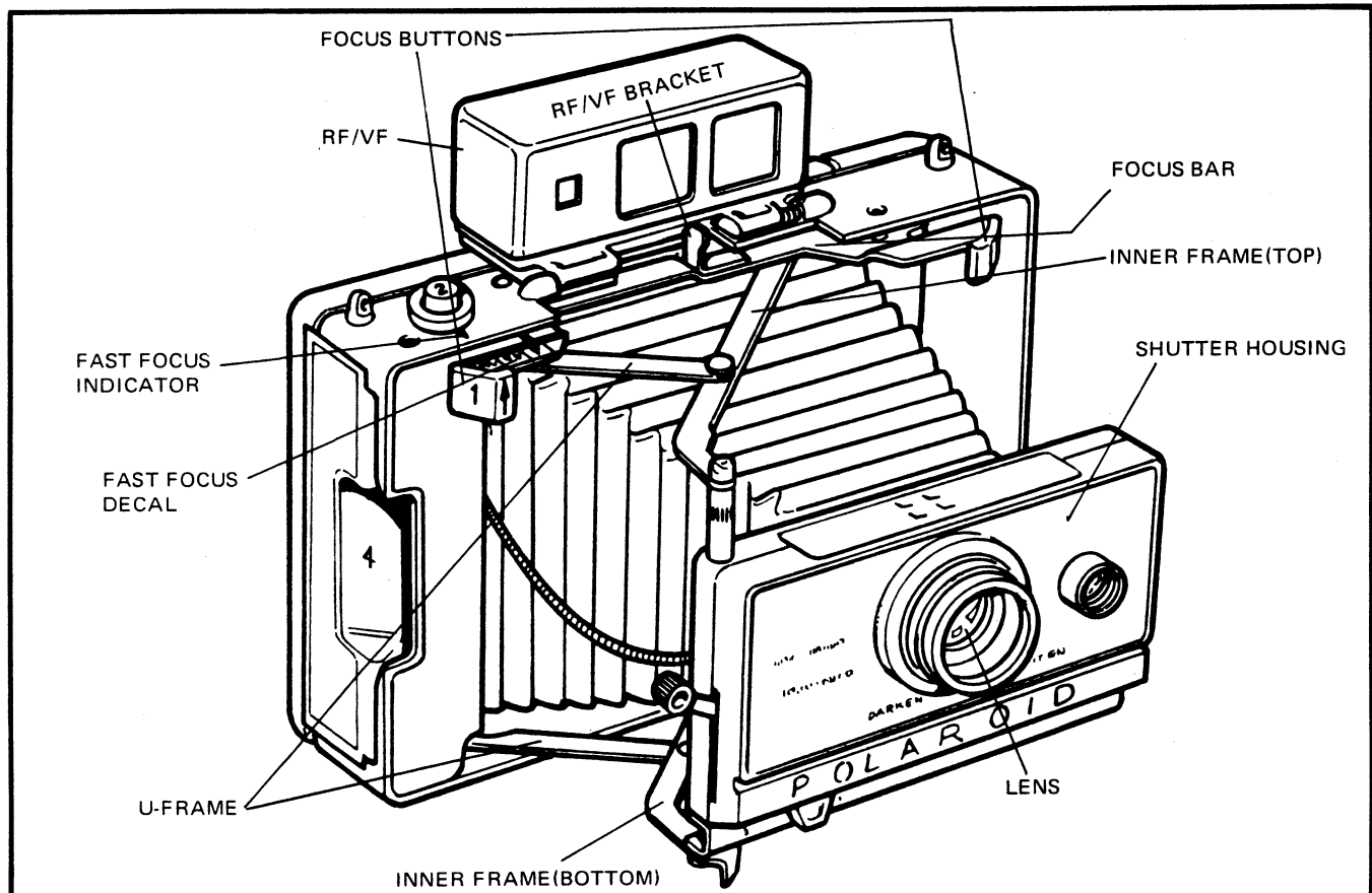
FIG. 2.6 FOCUSING COMPONENTS
