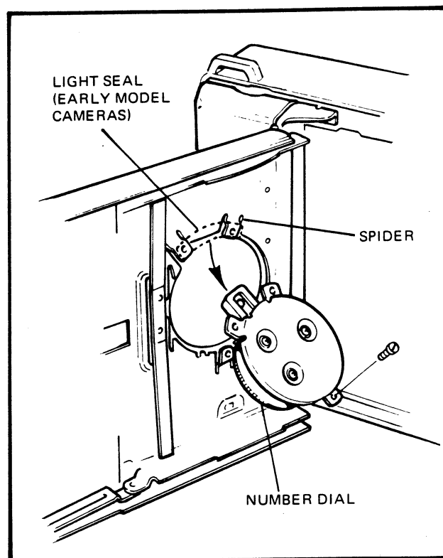
FIG. 5.31 REMOVING THE MECHANICAL TIMER
