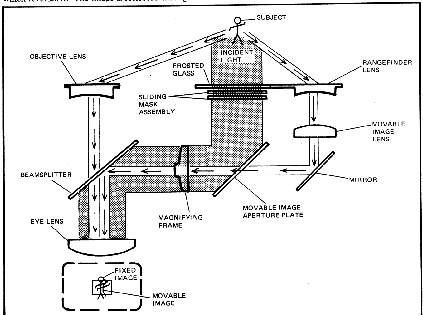
FIG. 2.9 ZEISS IKON RANGEFINDER/VIEWFINDER INTERNAL CONFIGURATION
