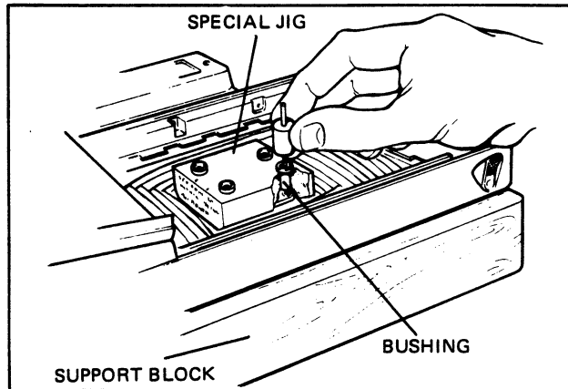
FIG. 5.11 DRILLING OUT THE POST
