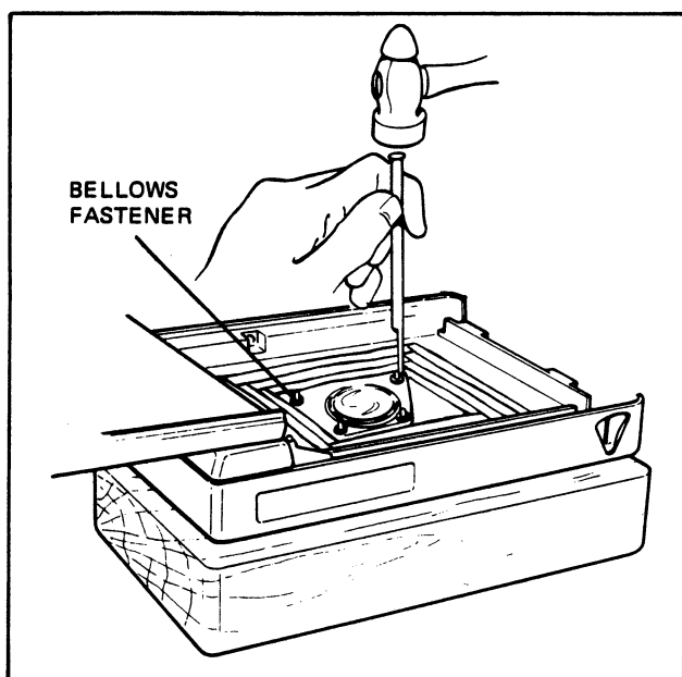
FIG. 5.8 REMOVING THE BELLOWS FASTENERS
