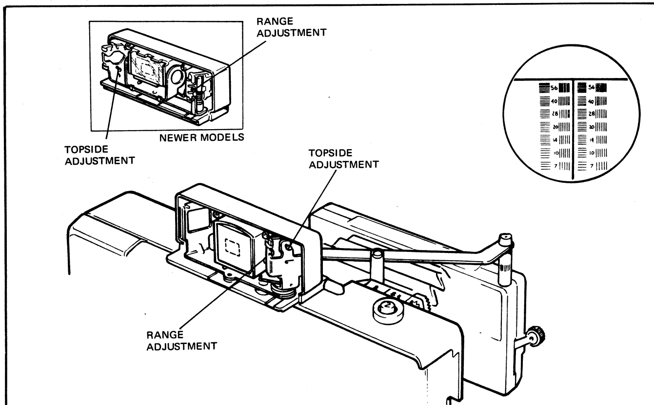
FIG. 5.47 RANGE/TOPSIDE ADJUSTMENTS FOR POLAROID RF/VF
