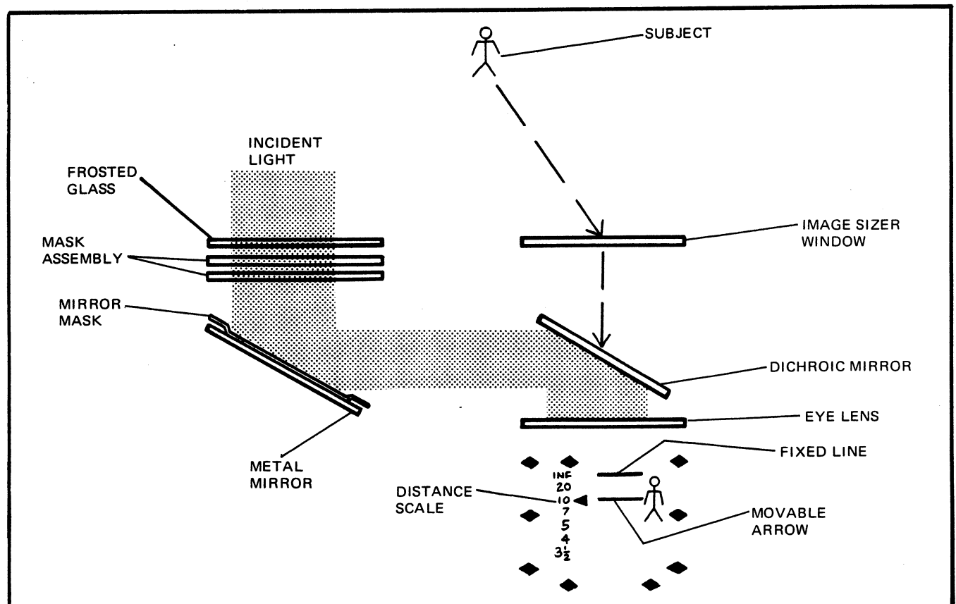
FIG. 2.7 IMAGE SIZER INTERNAL CONFIGURATION
