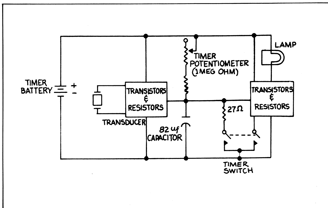
FIG. 2.14 ELECTRONIC TIMER SCHEMATIC
