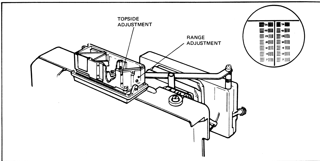
FIG. 5.46 RANGE/TOPSIDE ADJUSTMENTS FOR ZEISS IKON RF/VF
