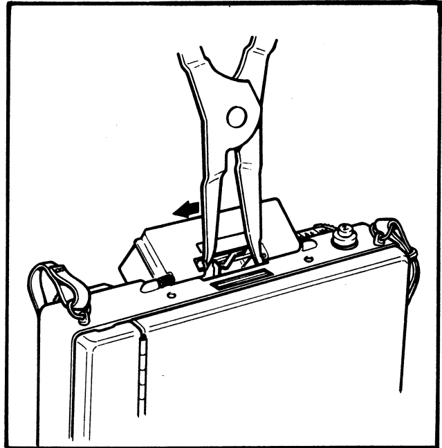
FIG. 5.43 INSTALLING A FOLDING RF/VF
