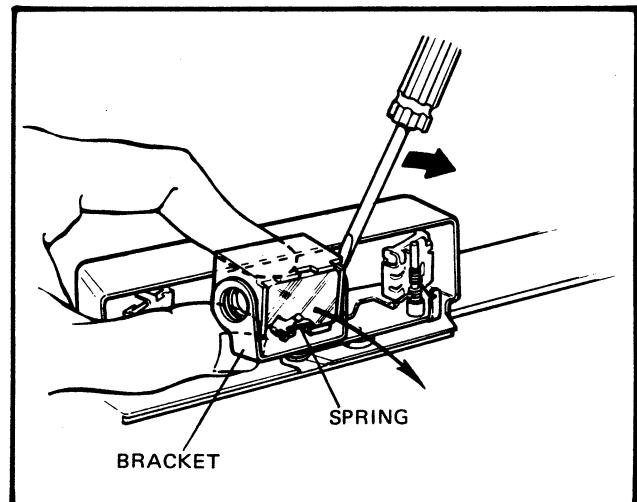
FIG. 5.44 REMOVING THE OPTICS ASSEMBLY
