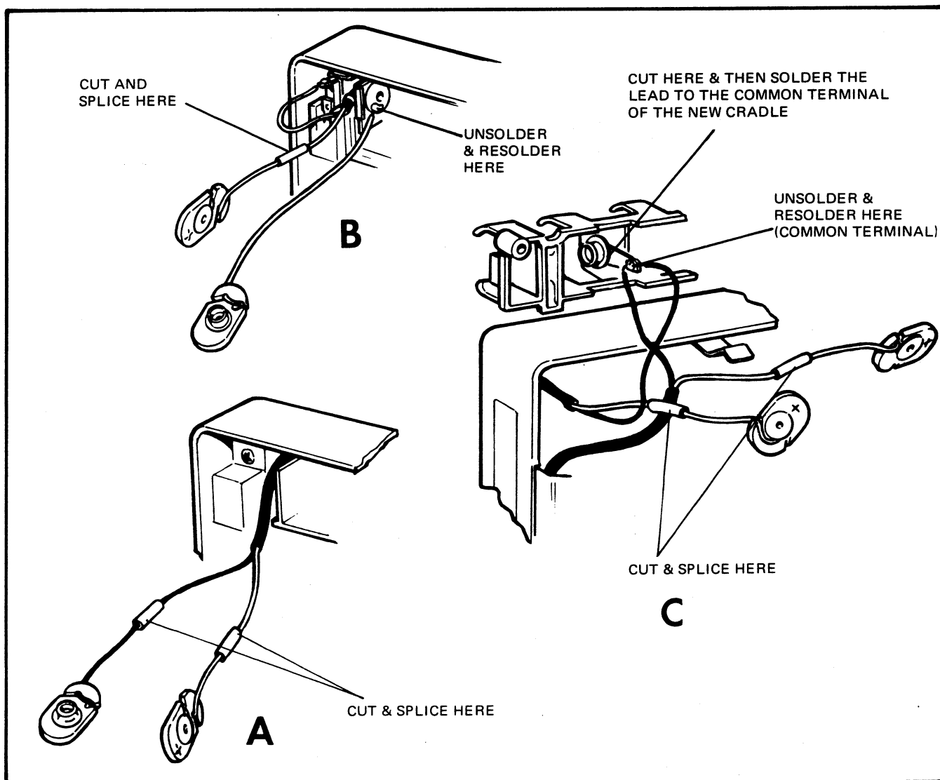
FIG. 5.30 REPLACING BATTERY TERMINAL
