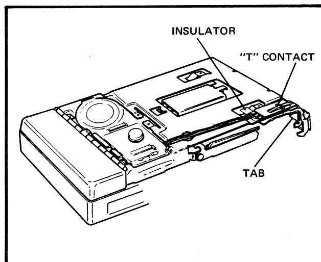
FIG. 5.40 CHECKING THE SWITCH UNDER LOAD
