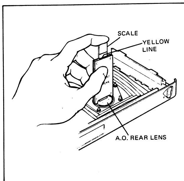
FIG. 5.17 IDENTIFYING THE REAR LENS
