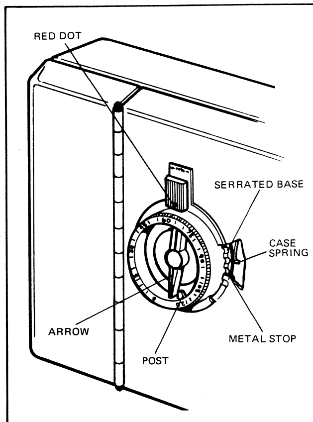
FIG. 2.12 SETTING OF THE TIMING RING
