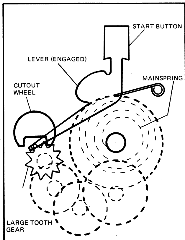
FIG. 2.11 INTERNAL CONFIGURATION OF THE MECHANICAL TIMER
