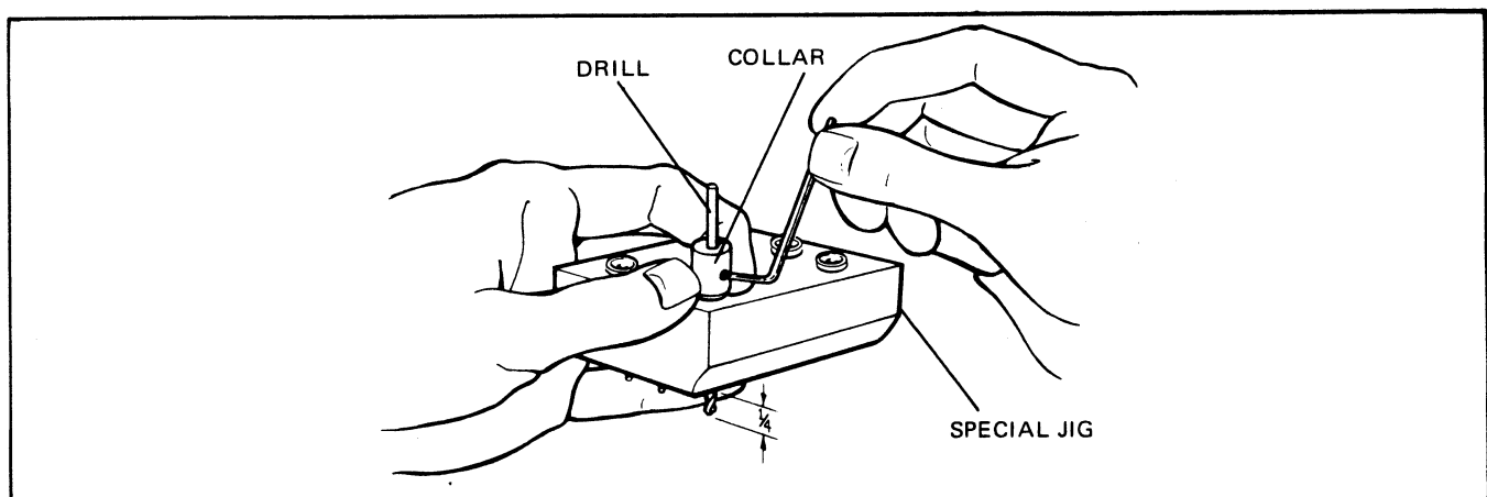
FIG. 5.10 PREPARING THE DRILL
