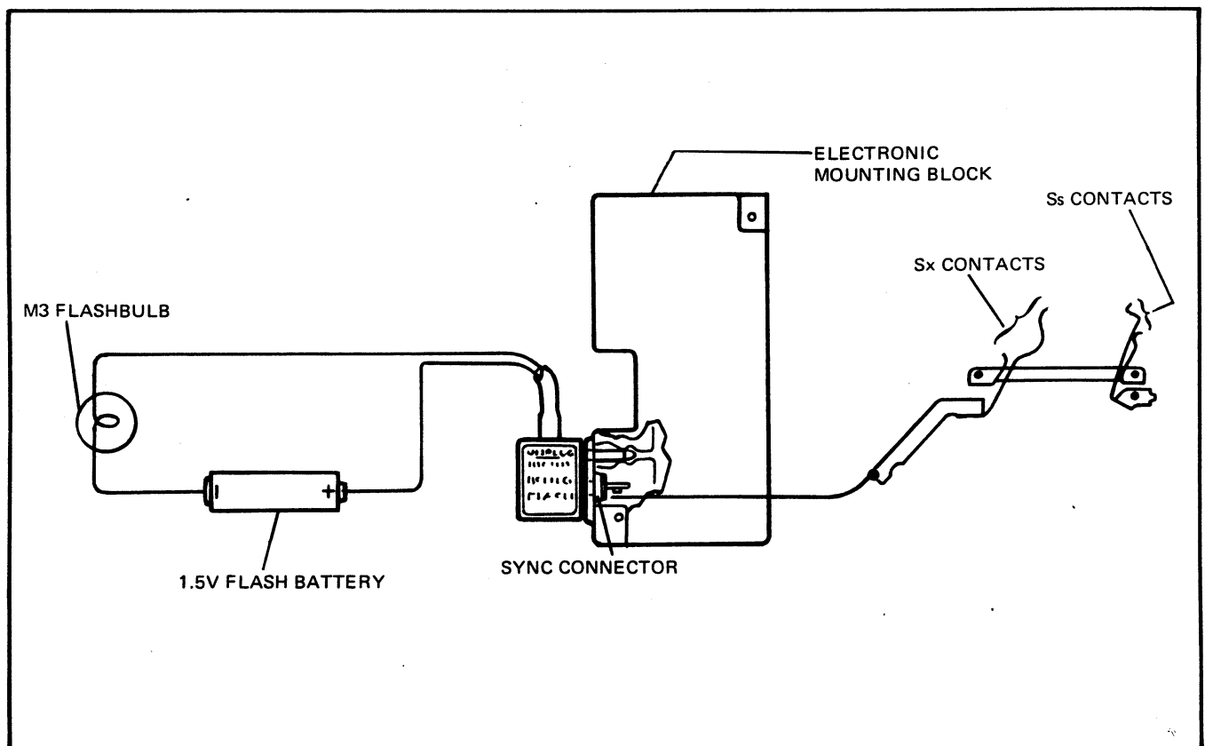
FIG. 2.16 FLASHGUN CIRCUIT
