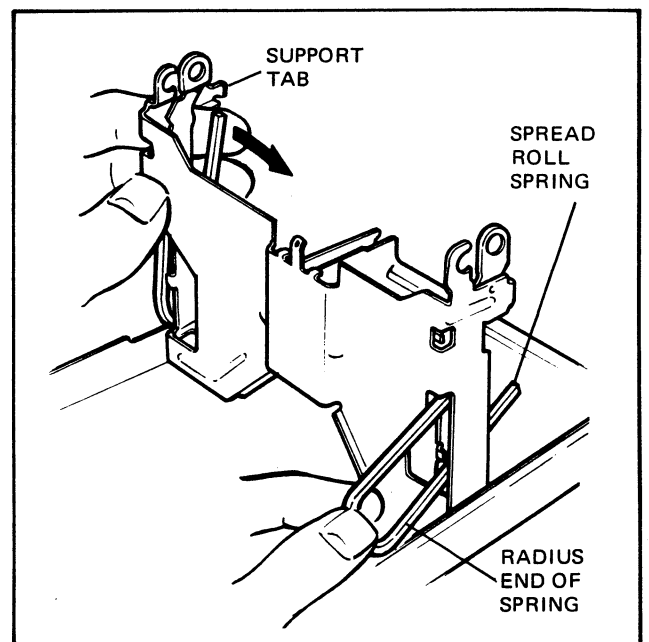
FIG. 5.7 REMOVING THE SPREAD ROLL SPRING
