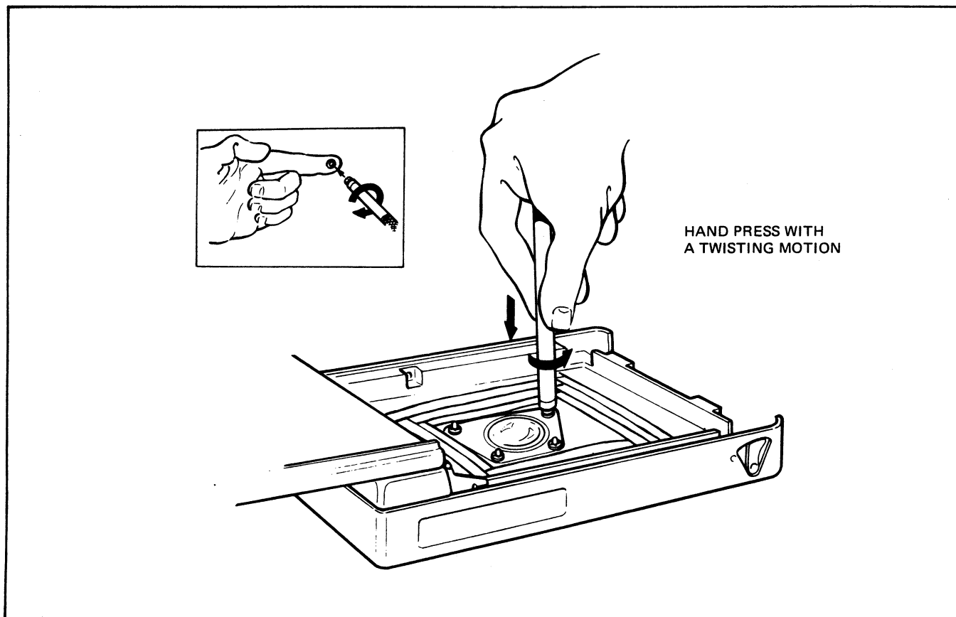
FIG. 5.9 INSTALLING NEW FASTENERS
