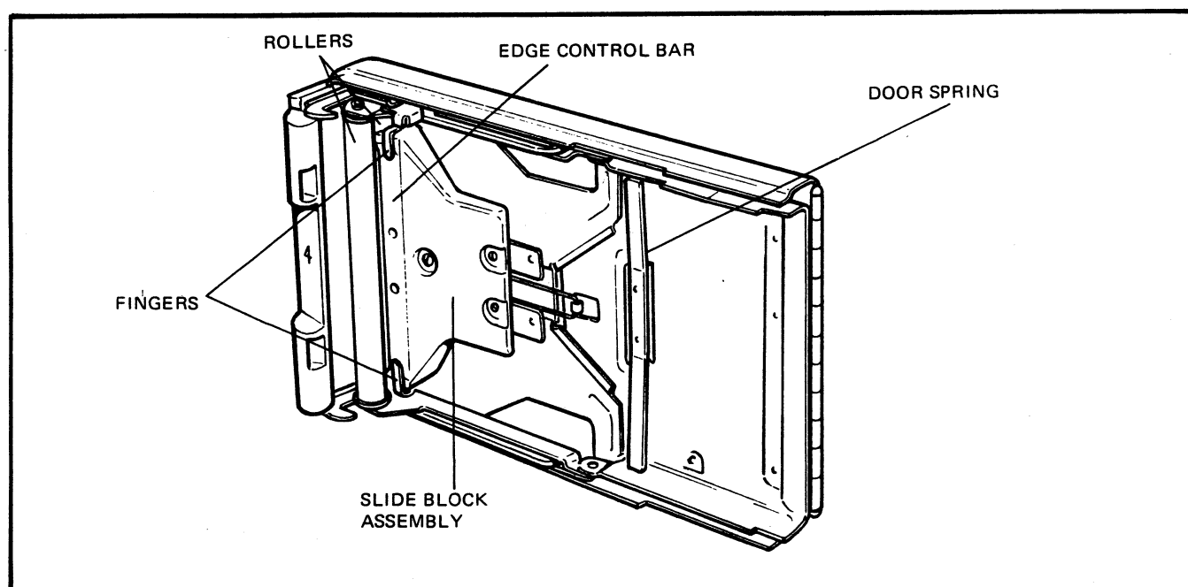
FIG. 2.4 VIEW OF REAR DOOR COMPONENTS
