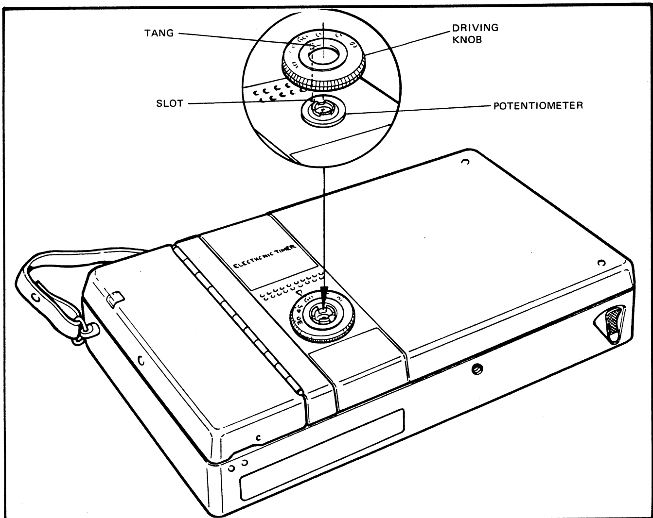
FIG. 5.38 INSTALLING THE NEW KNOB
