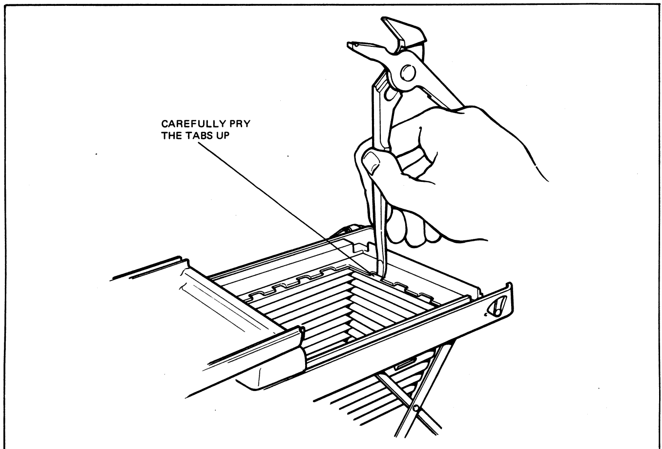
FIG. 5.12 PRYING THE BELLOWS TABS
