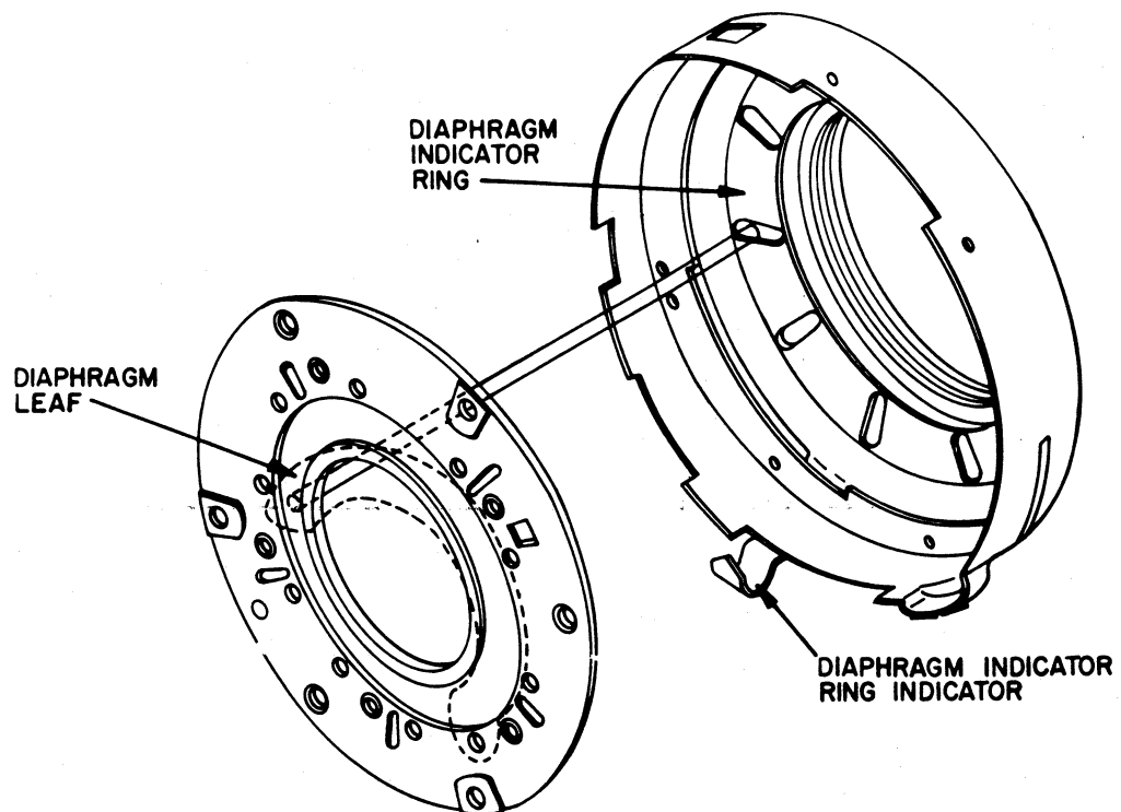
Figure 6. DIAPHRAGM OPERATION
