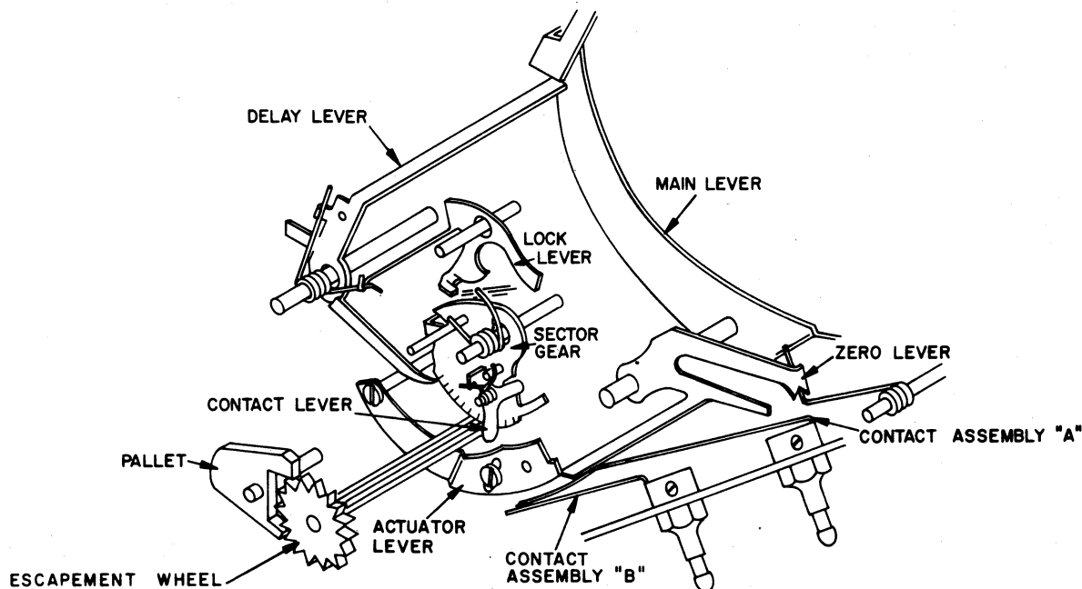
Figure 7. SYNCHRONIZER OPERATION
