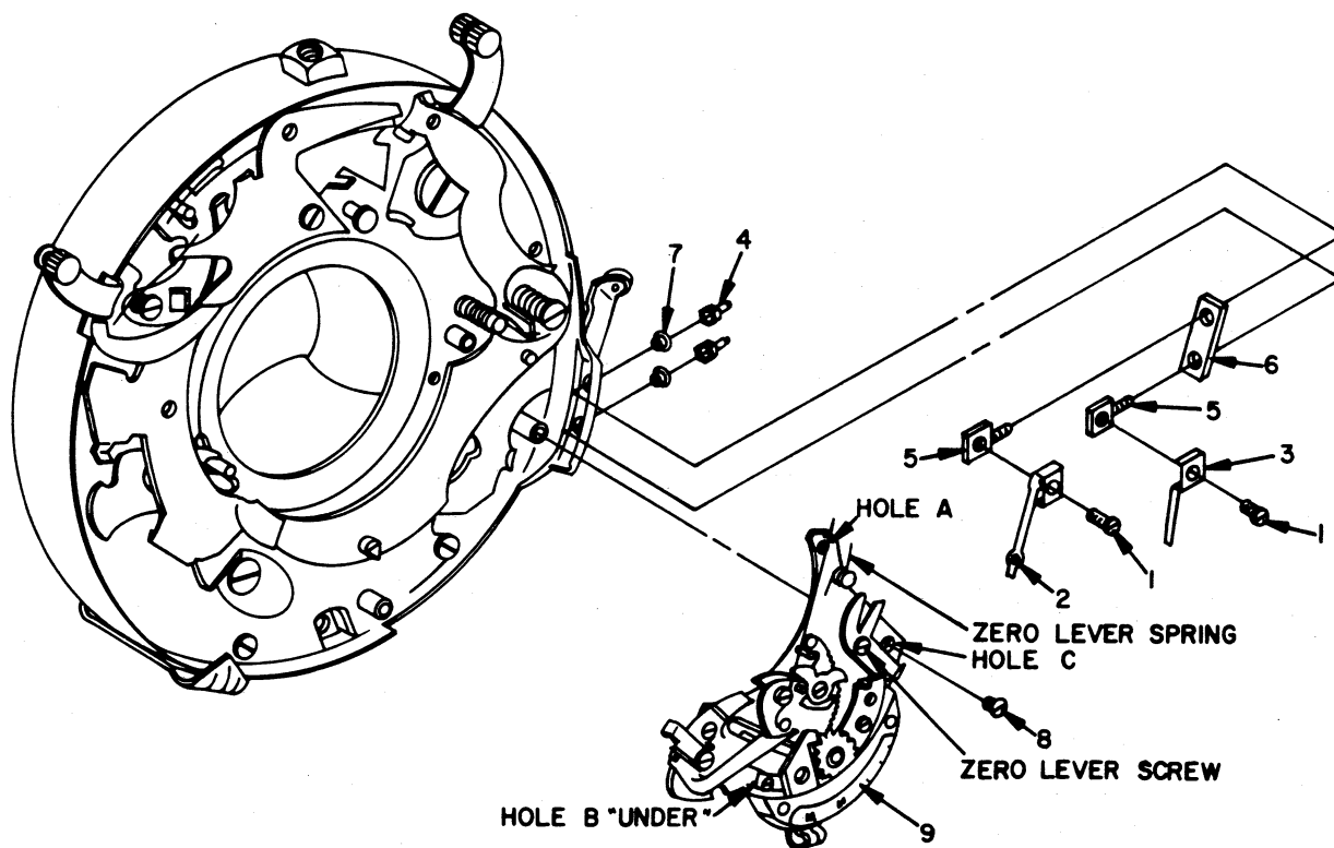
Figure 9. NO. 1 SHUTTER, DISASSEMBLY - STAGE 2
