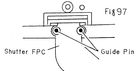
(Top View of Camera)
