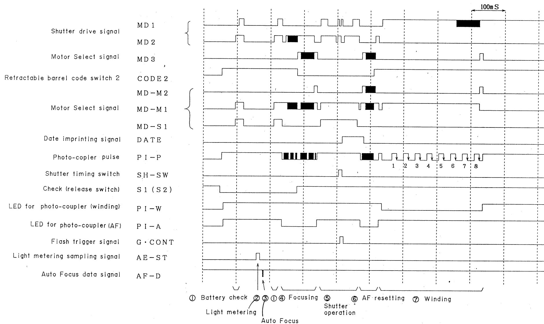
Timing Chart
