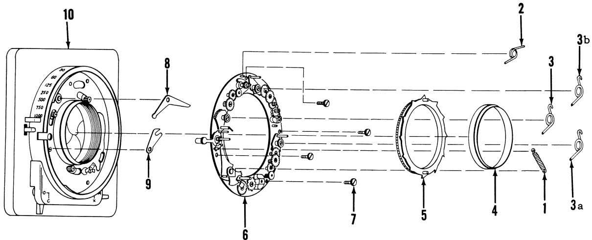
Figure 23. SHUTTER ASSEMBLY - SECOND
