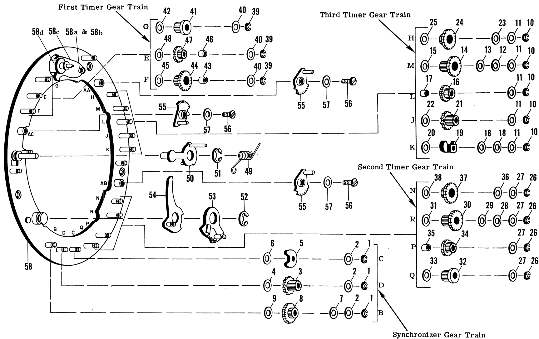
Figure 26. CONTROL PLATE COMPLETE
