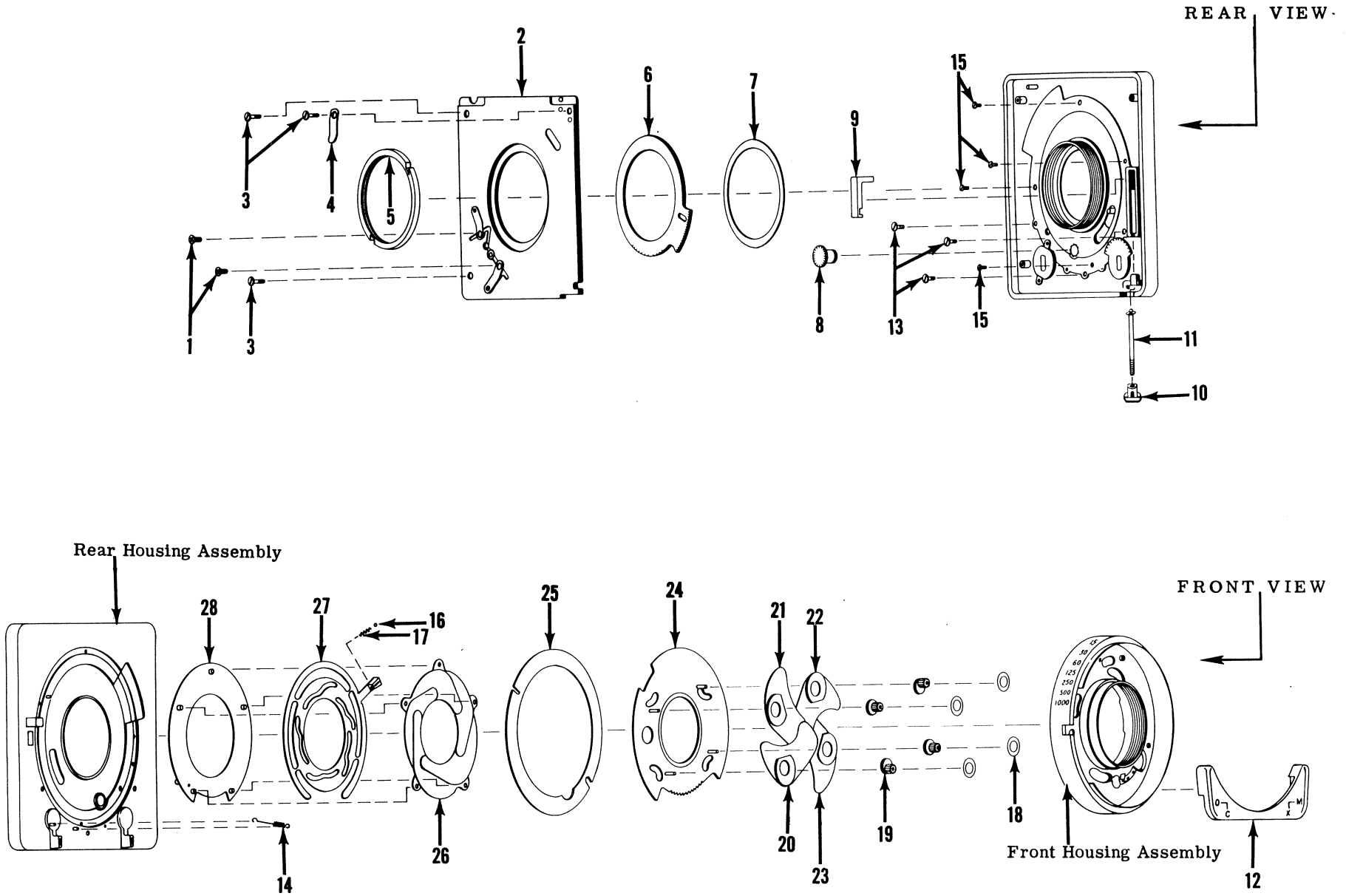
Figure 24. SHUTTER ASSEMBLY - FIRST (Model 2A)
