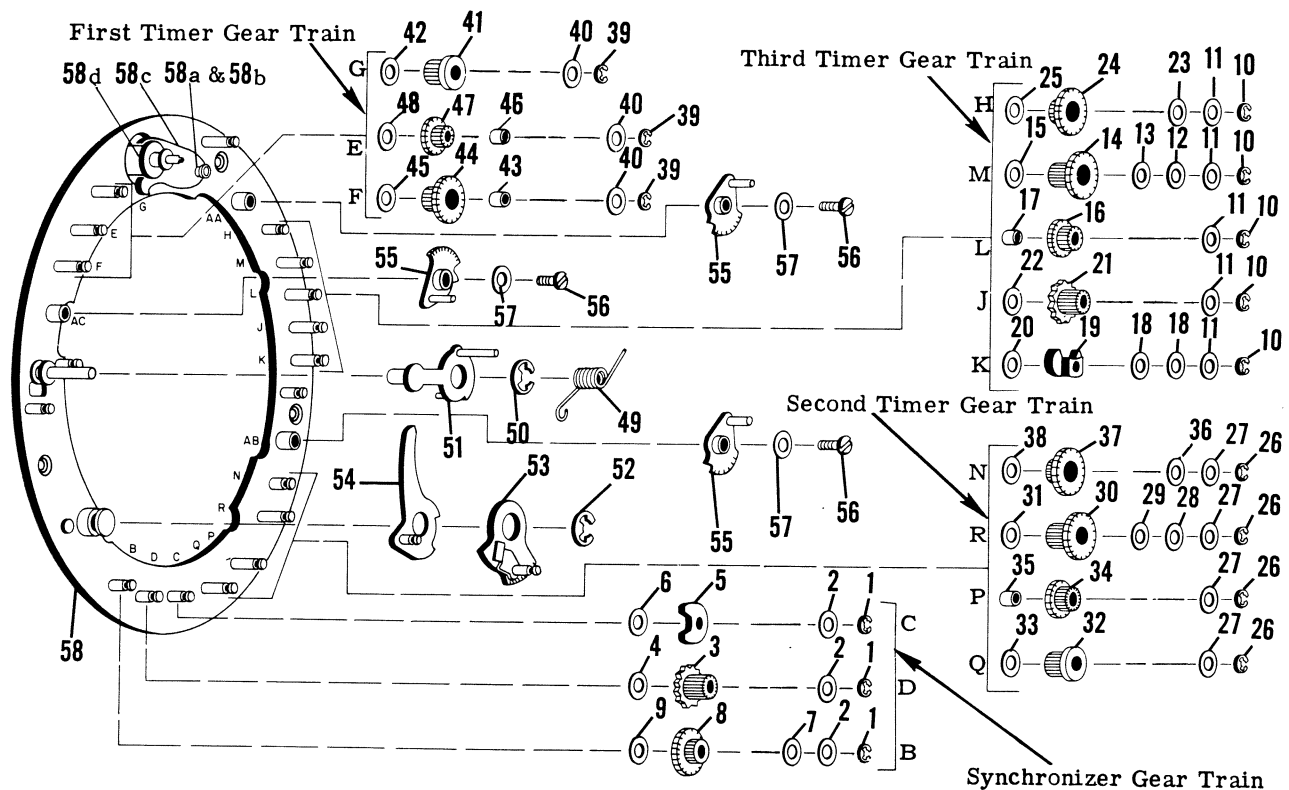
Figure 5. CONTROL PLATE COMPLETE
