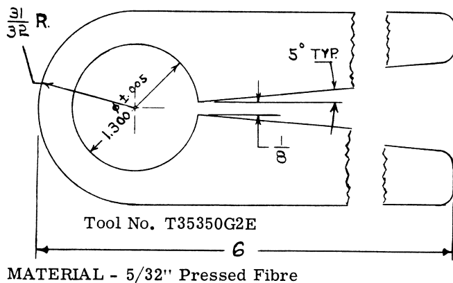
Figure 2. FRICTION WRENCH (use on rear lens element)
