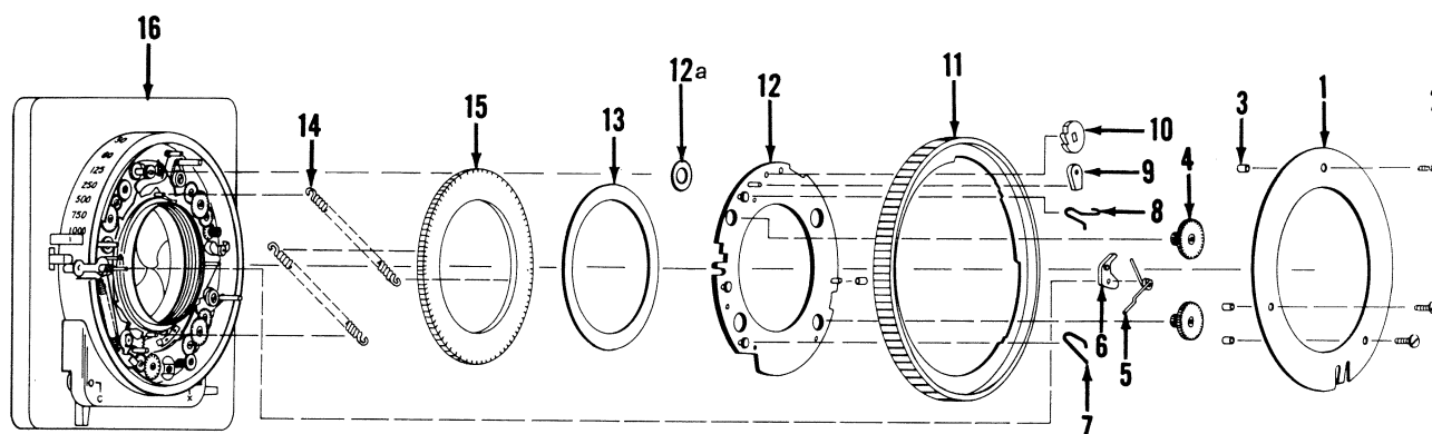
Figure 22. SHUTTER ASSEMBLY - THIRD
