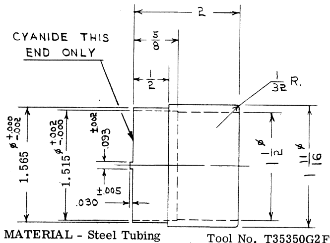
Figure 1. TUBULAR WRENCH (use on front lens element)
