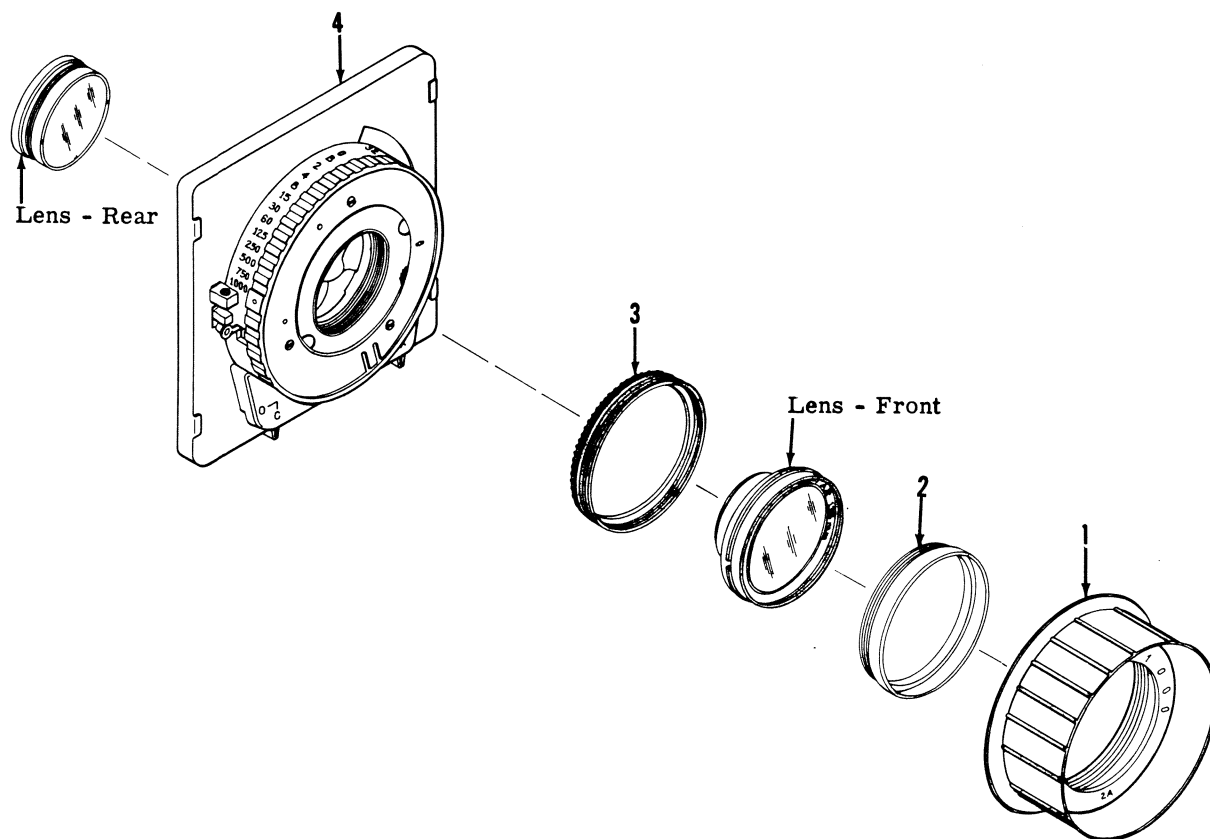
Figure 21. GRAFLEX 1000 SHUTTER
