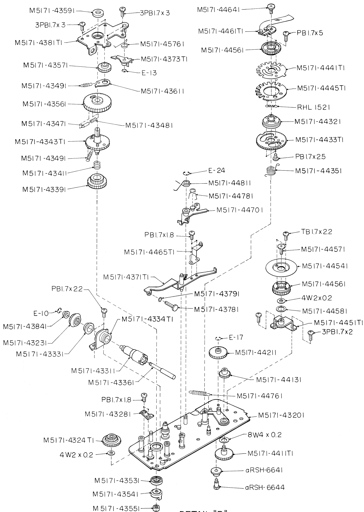
DETAIL "B"
