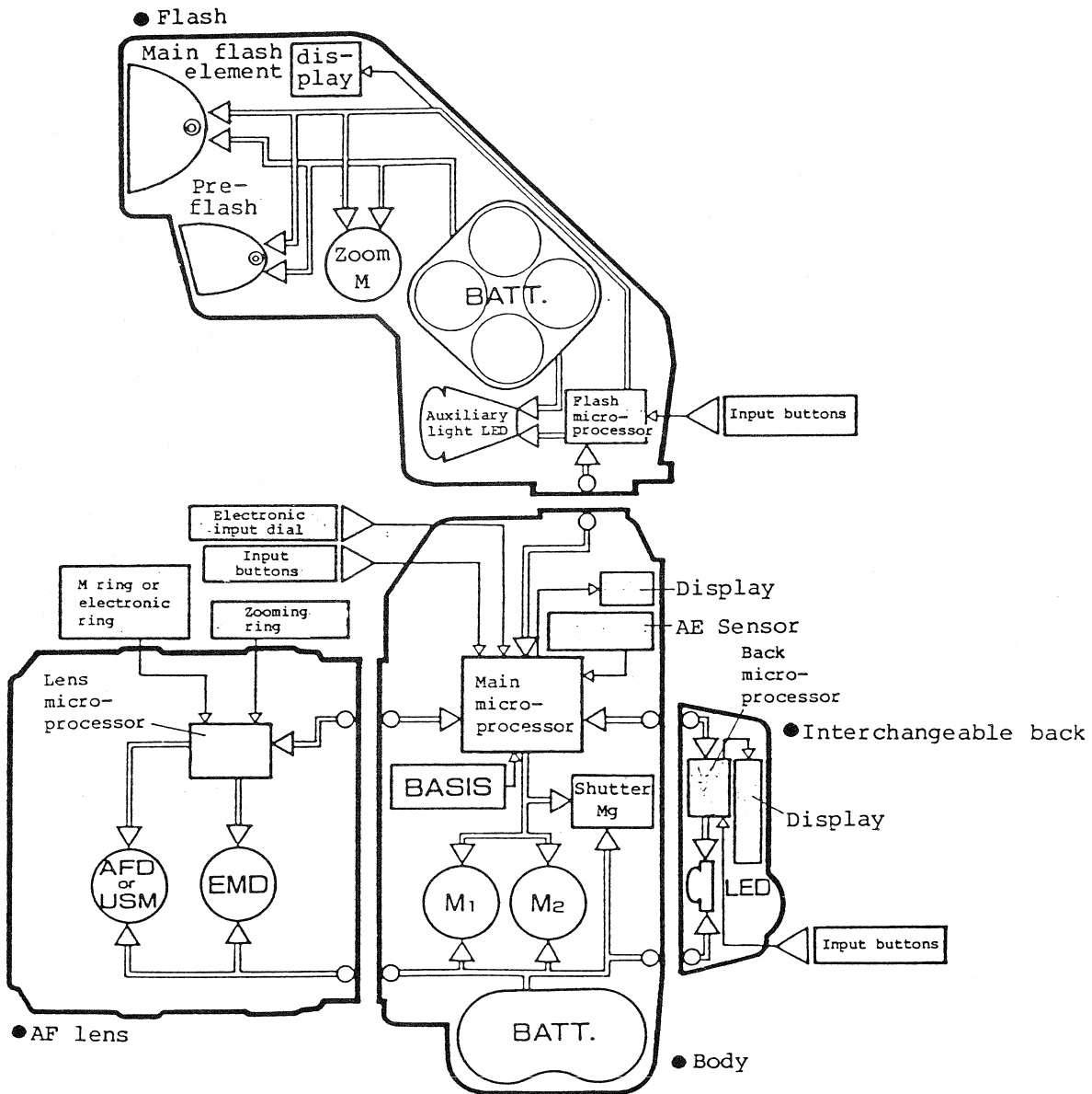
Fig. 1: Control System Structure
