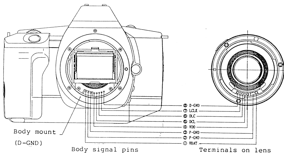
[1]-Fig.-2 Electronic mount signals
