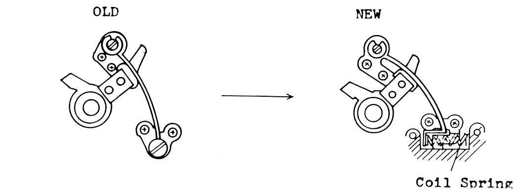
Brake Band
