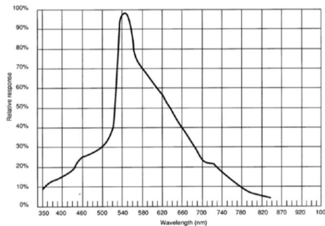
Figure 5 Spectral response
