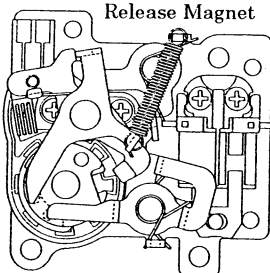
One revolution limit released by operation of One Revolution Limit Release Magnet
