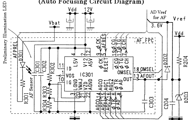
(Auto Focusing Circuit Diagram)
