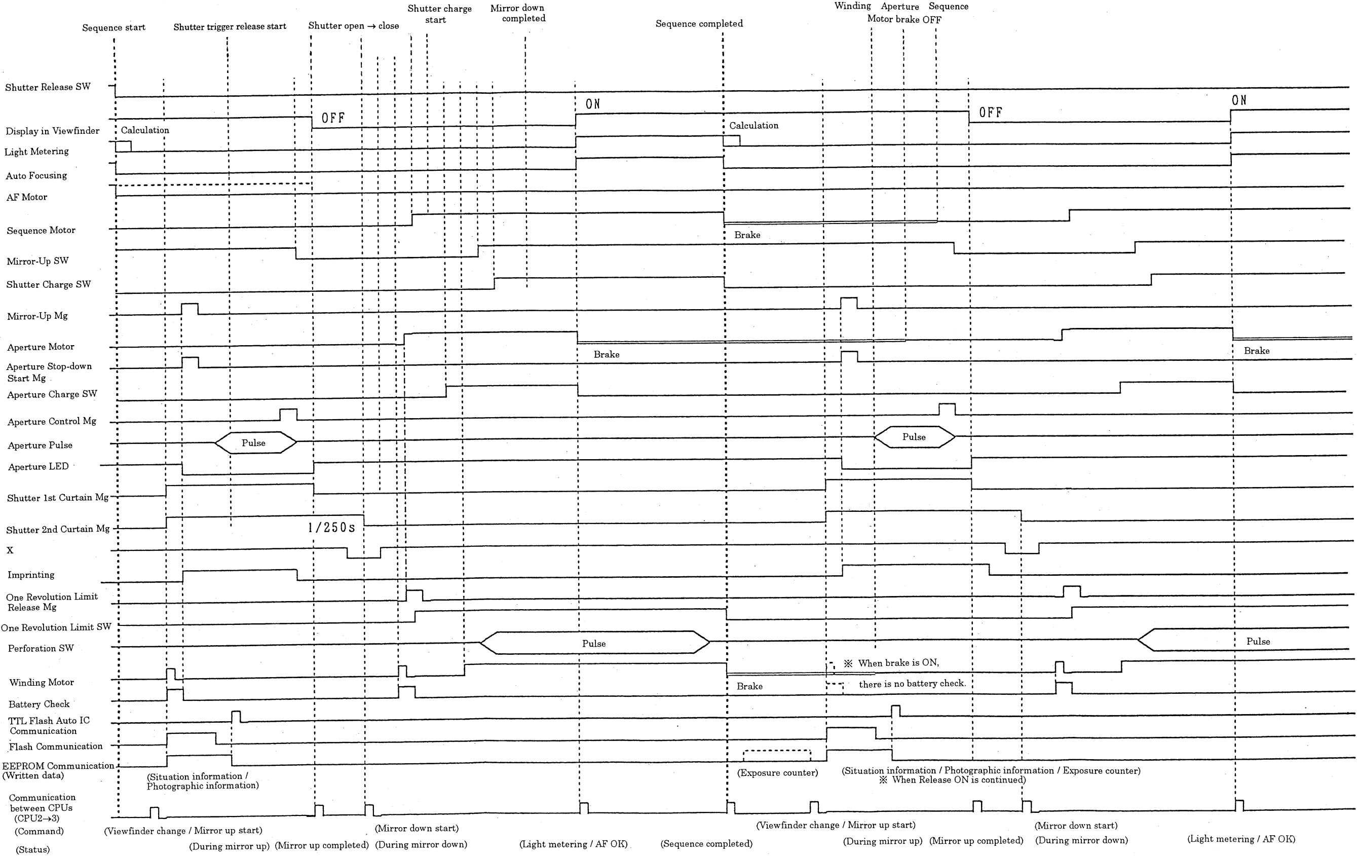
TIMING CHART * AF Mode, CH Mode, ISO 100
