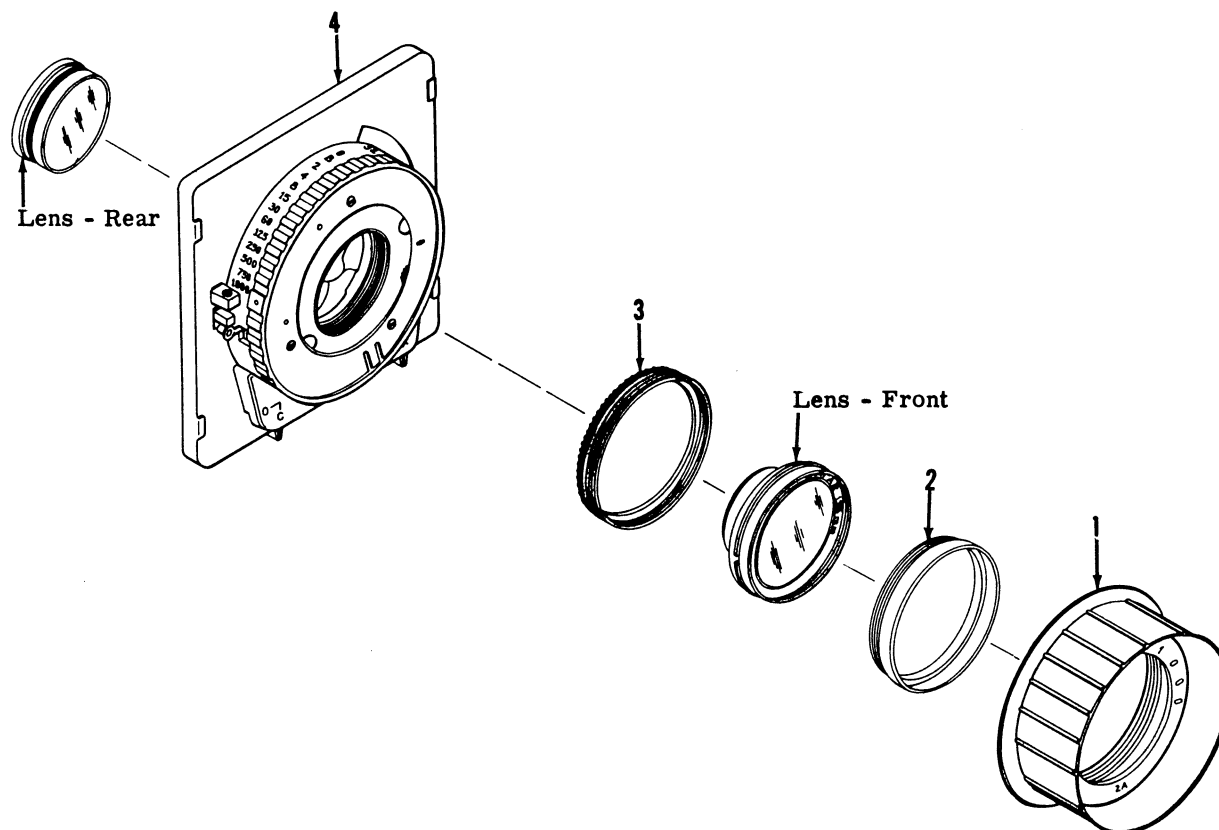
Figure 21. GRAFLEX 1000 SHUTTER
