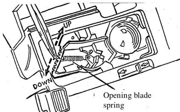
Fig. 4 Adjusting Opening Blade Spring
