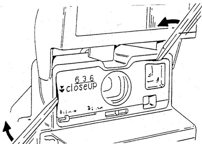
Fig. 9 Removing the Panel (Front Plate) from the Apron
