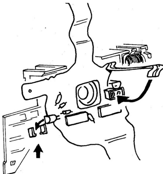
Fig. 28 Replacing the Flex on the Base Block
