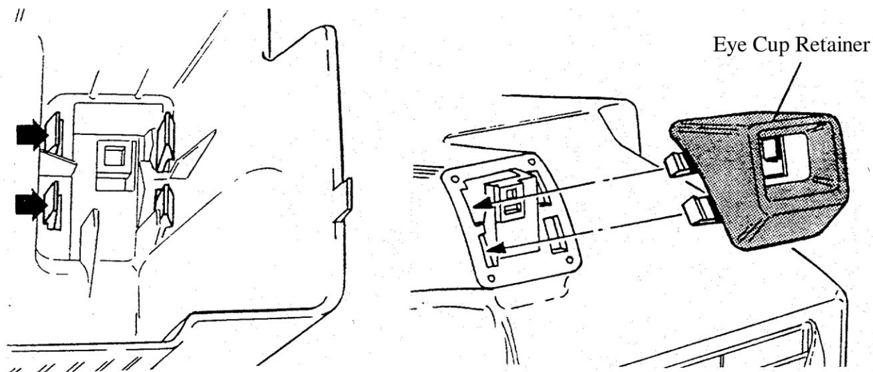
Fig. 16 Removing the Eye Cup/Retainer
