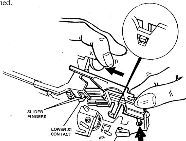
Fig. 46 Verifying Slider-Switch contact relationship
