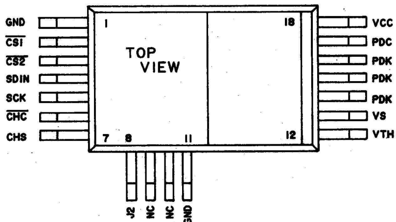
[Flash control IC terminal arrangement]
