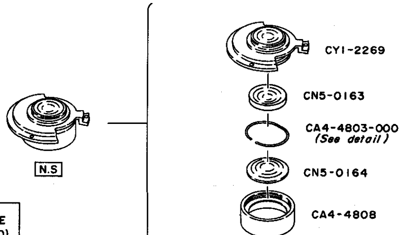
CA4-4803-000 detail
