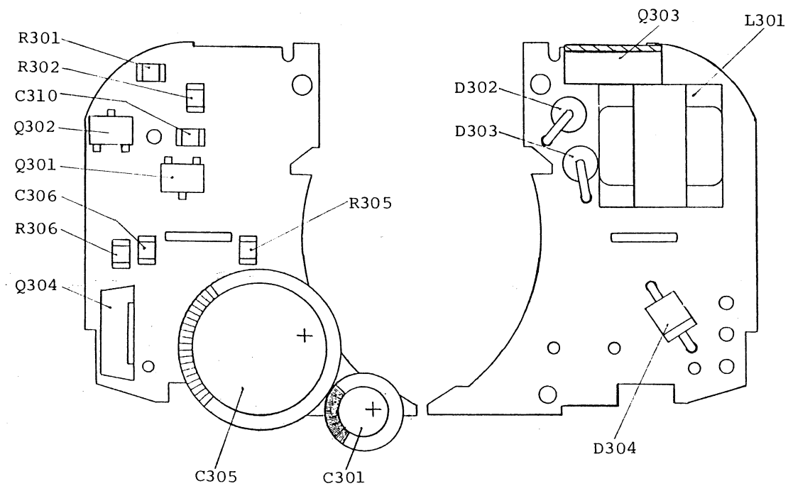
Flash Board (1)
